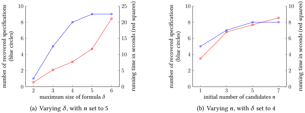
Fig. 7. Number of recovered specifications and running time for different choices of hyperparameters n and \delta
