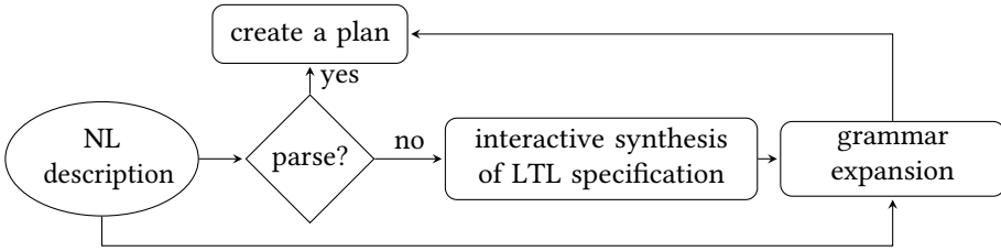
Fig. 1. Schematic view of LTLTALK
