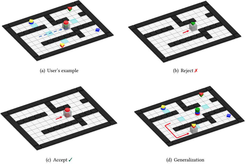
Fig. 2. User's interaction with LTLTALK. In 2(a) the user provides an example for the command take one red item from 7,4 by moving the robot to (7, 4) and picking a red item. Afterwards, based on the example and the (natural language) command, a number of candidate specifications is created. In 2(b) LTLTALK shows the robot picking one green item, which the user rejects. In 2(c) LTLTALK shows the robot picking (7, 4) without ever going through a wet tile and picking only one red item. The user accepts it, thus narrowing down the set of candidates to a single specification. Finally, 2(d) shows that LTLTALK generalized from the inferred specification and now understands commands such as take every triangle item from 4,0 .
