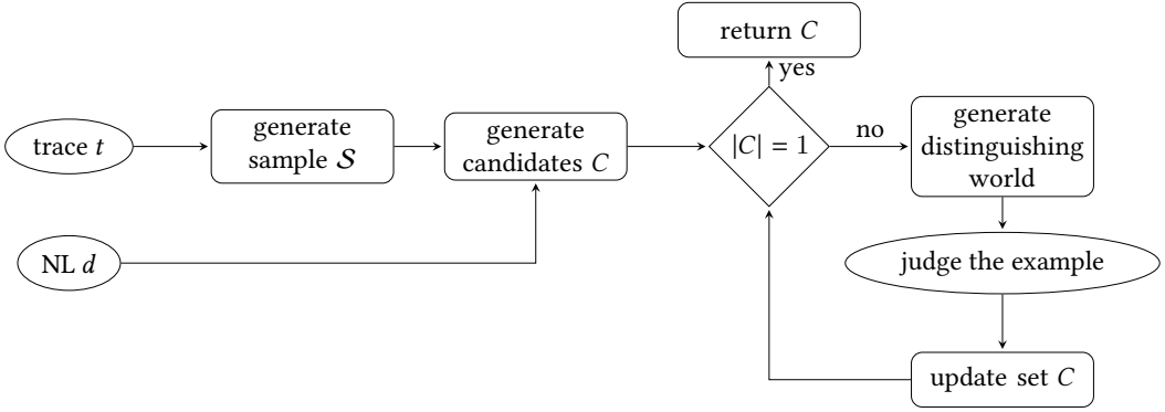
Fig. 4. High-level interactive synthesis algorithm
