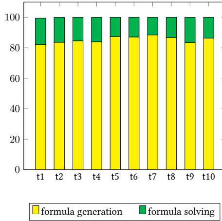
Fig. 6. Relative times needed to generate and to solve formula \Phi_{\delta}^{S,L}
