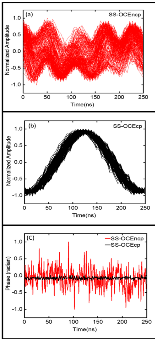
FIGURE 3. Fringe stability for (a) the SS-OCEncp and (b) the SS-OCEcp systems and (c) the measured phase for both systems.
