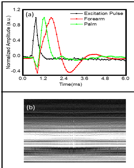
FIGURE 5. (a) Normalized amplitude of the displacement caused by the SAW for different locations on hand. (b) OCT frame in M-mode for the forearm skin acquired over 25 milliseconds at one location, image size in depth equals 1 mm.
