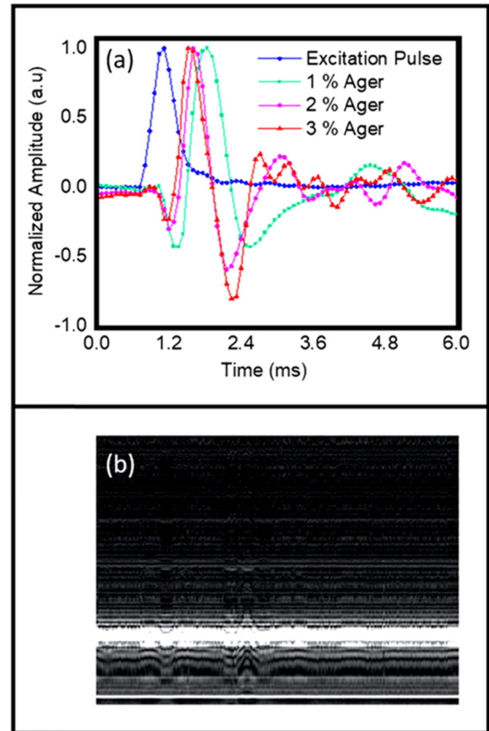
FIGURE 4. (a) Normalized amplitude of the displacement caused by the SAW for different concentrations of the agar phantoms. (b) OCT frame in M-mode for the 3% agar phantom acquired over 25 milliseconds at one location, image size in depth equals 1 mm.
