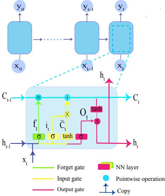
FIG. 11. An LSTM-NN structure made of a chain of repeating modules, where each module includes three gates.
