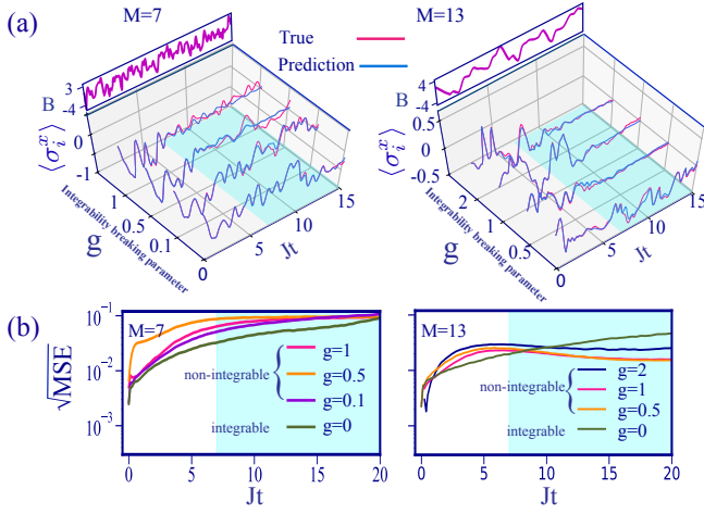
FIG. 17. Comparing the power of the LSTM-NN in predicting the dynamics of quantum-integrable models versus quantum non-integrable models. (a) Comparing the performance of the LSTM-NN in predicting \langle \sigma_i^x \rangle against the true evolution for different values of g under the shown driving fields. (b) The \sqrt{\text{MSE}} versus time in predicting all the first and second-order moments of spin operators for different values of g where the spin-ring is driven by Gaussian random transverse fields. For each value of g , the NN is evaluated on 1000 realizations for system sizes M = 7 and M = 13 . The blue highlighted region shows the interval that the NN has not been trained on.
