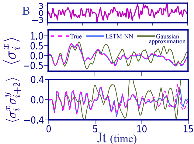
FIG. 6. Illustrating the power of the NN in finding internal representations of higher-order correlations. We compare the NN predictions with the solutions of the equations of motion for correlators, truncated at the Gaussian level. The NN prediction is much closer to the true dynamics, especially at longer times. (A spin ring of size M = 7 is driven by the transverse field shown at the top of the panel; spins are initially prepared in the z direction)
