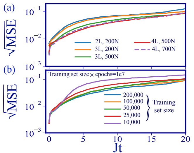
FIG. 13. Role of the LSTM-NN size and training set size on the performance of LSTM-NN. (a) The \sqrt{\text{MSE}} versus time for different NN size. L and N stand for number of layers and number of neurons, respectively. (b) The \sqrt{\text{MSE}} versus time for different training set size.
