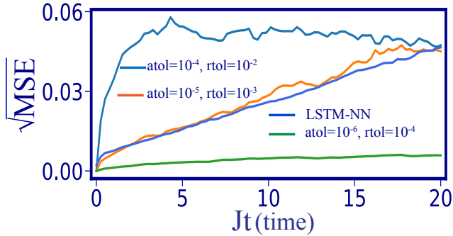
FIG. 16. Comparing the error in predicting the dynamics of the observables by the LSTM-NN vs. the error in numerical integration for different relative and absolute tolerances. The shown results are related to the driven TFI model with M = 15 and we averaged over 100 realizations of random driving fields.
