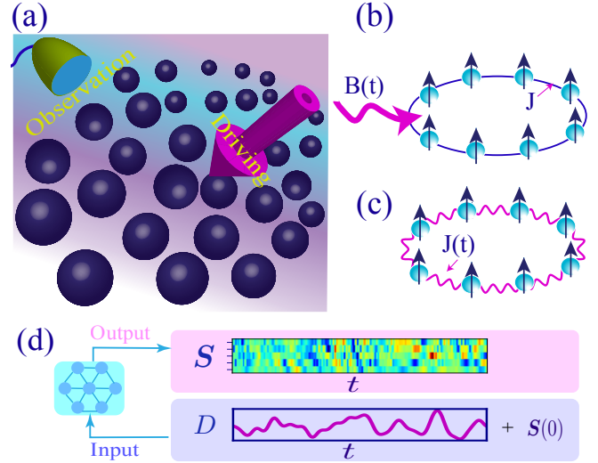
FIG. 1. Scenario considered in this work. (a) Schematic representation of a quantum many-body system subject to an arbitrary driving field, where the goal is to predict the time-evolution of a set of observables. The models that we explore here, as for illustration, are spin ring subject to (b) time-dependent magnetic field or (c) time-dependent exchange couplings. (d) Schematic representation of input and output of the NN. The input of the NN is the driving trajectory D(t) , together with other time-independent parameters and a description of the initial state of the system shown by S_0 . As output the NN predicts the full evolution of expectation values of observables of interest, generically denoted by S(t) in the figure. This includes local observables but may also comprise, e.g., spatial two-point correlators.
