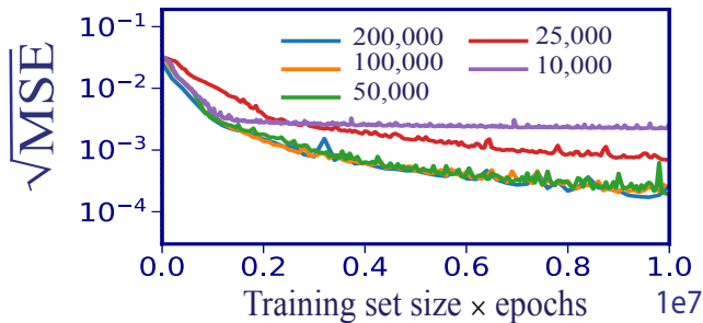
FIG. 4. The error \sqrt{\text{MSE}} versus number of instances that the NN has seen during training for different training set sizes (results for a M = 7 spin ring, training on Gaussian random driving fields).
