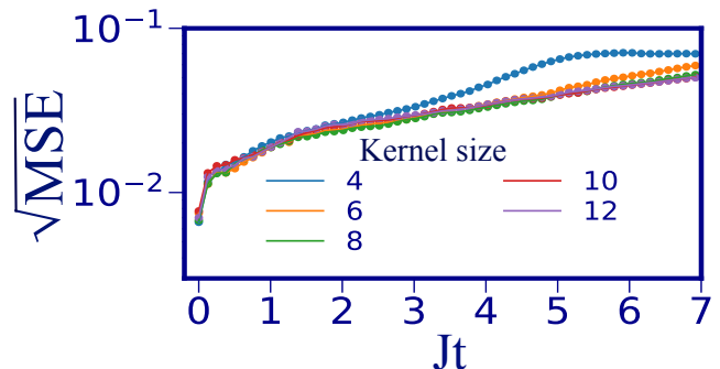
FIG. 12. The performance of a temporal 1D-CNN for different kernel sizes on the TFI model driven with Gaussian driving random fields, ( M = 15 ). The \sqrt{\text{MSE}} versus time averaged over all the selected observables and over 1000 realizations of Gaussian random driving fields.
