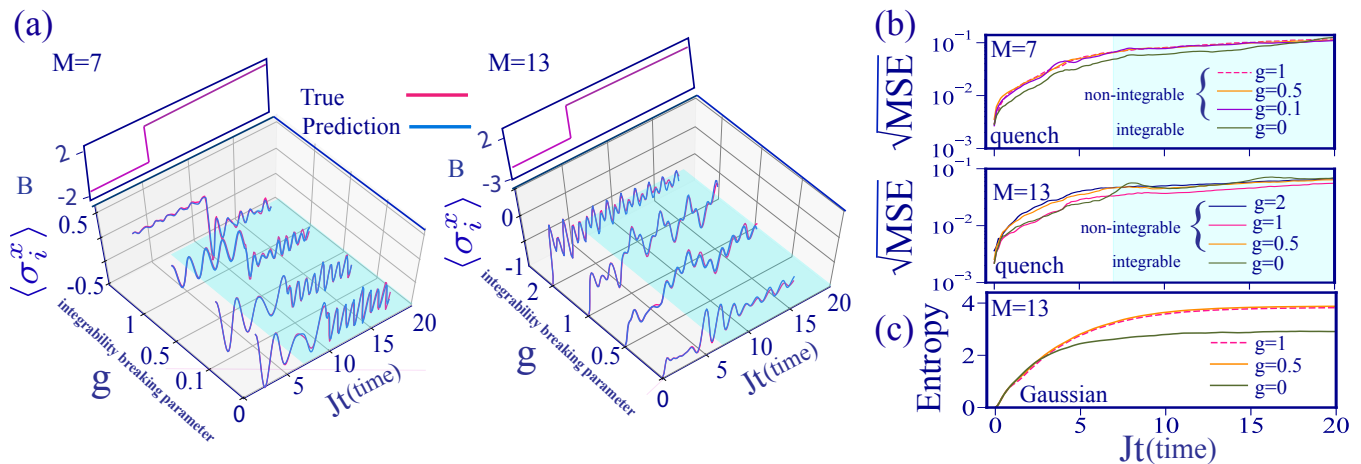
FIG. 8. Comparing the power of the LSTM-NN in predicting the dynamics of quantum-integrable models versus non-integrable models. (a) Comparing the performance of the LSTM-NN in predicting \sigma_i^x against its true evolution for different values of the integrability-breaking parameter g under the quenches shown here. (b) Prediction error versus time, for different values of g , where the spin-ring is subject to different sorts of quenches. For each value of g , the NN is evaluated on 1000 realizations for system sizes M = 7 and M = 13 . The light blue regions show the interval that the NN has not been trained on. (c) Evolution of the entanglement, as measured by the von Neumann entropy of a subsystem (averaged over 1000 realizations of random driving fields).
