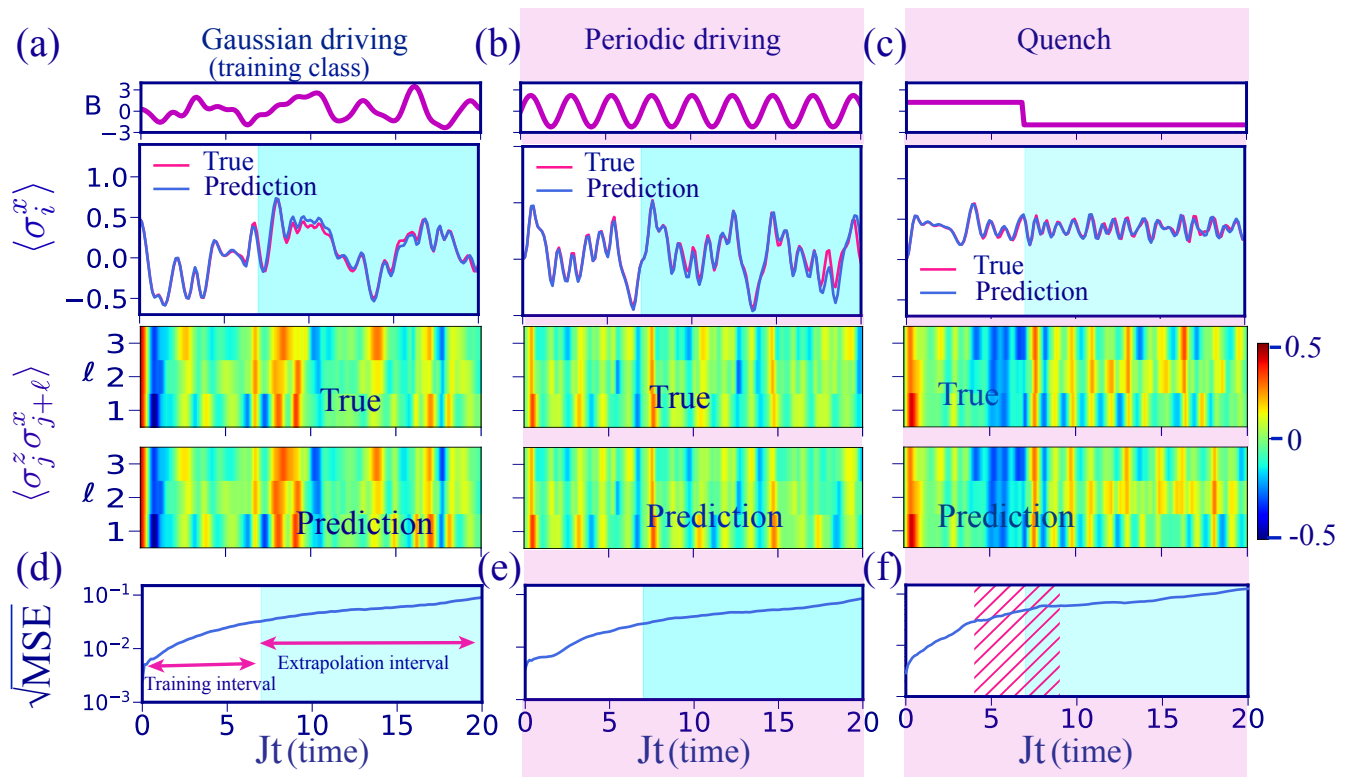
FIG. 3. Demonstrating the high accuracy of the LSTM-NN in predicting the dynamics of a spin system under arbitrary driving. We train the NN on Gaussian random driving fields for a fixed time interval (here: Jt \in [0, 7] ) and then evaluate the prediction of the NN for different classes of driving fields, and also for a larger time interval ( Jt \in [0, 20] ). In this example, we compare the true and predicted evolution of \langle \sigma_i^x \rangle and \langle \sigma_i^z \sigma_{i+\ell}^z \rangle for a transverse-field Ising spin ring of size M = 7 . Comparisons are displayed for different classes of driving fields: (a) a realization of a Gaussian process that has not been seen during training, (b) periodic driving, and (c) a quench. In the case of Gaussian driving, the spins are initialized in a translationally-invariant product state with random spin direction, while in (b) and (c) we chose to prepare the spins along the z -direction. The time window highlighted in light blue ( Jt \in [7, 20] ) corresponds to a region beyond the one where the NN was trained on. The last row shows the evolution of the error (as given by \sqrt{\text{MSE}} , see main text) of the NN's prediction averaged over all the selected observables and over 1000 realizations of each type of driving field: Gaussian random fields in (d), periodic fields in (e), and (f) quenches between random static parameter values (quench times randomly chosen inside hatched region). For (d,e,f), the spins are initialized in a product state with random spin direction. Note that in the second and third column (highlighted in pink) the driving fields are not even in the class of functions that the NN has been trained on.
