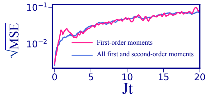
FIG. 14. Comparing the performance of the NN for the case where it is trained just over first-order moments of spin operators, vs. the case where it is trained over all first and second-order moments of spin operators. The \sqrt{\text{MSE}} versus time averaged over all the selected observables and over 1000 realizations of Gaussian random driving fields.
