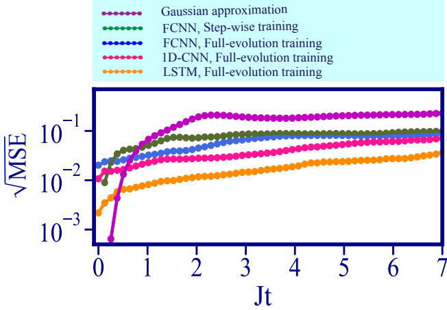
FIG. 15. Comparing the performance of different NN architectures against Gaussian approximation.
