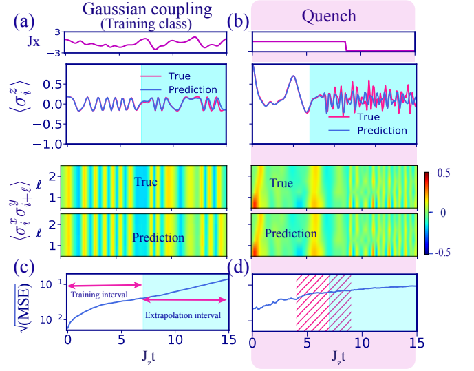
FIG. 18. The power of the LSTM-NN in predicting the dynamics of a Heisenberg spin ring under time-dependent exchange couplings with M = 9 . The NN is trained on Gaussian random exchange couplings in J_z t \in [0, 7] and then is evaluated on a new set of Gaussian random exchange couplings as well as different sorts of quenches in the time window J_z t \in [0, 15] . Comparing the real and predicted evolution of \langle \sigma_i^x \rangle and \langle \sigma_i^x \sigma_{i+\ell}^y \rangle for different values of \ell under the shown (a) Gaussian random coupling (b) quench (in direction of x ) at the top of each panel. The highlighted blue regions denote the time window that the NN has not been trained on. The highlighted light pink column remarks that NN is evaluated on the class of couplings that the NN has never seen. The \sqrt{\text{MSE}} in predicting all first and second-order moments of spin operators where the spin ring is driven by (c) 1000 Gaussian random exchange couplings, (d) 1000 random quenches in direction of x . The striped area shows the region in which the time of the jump has been randomly chosen.
