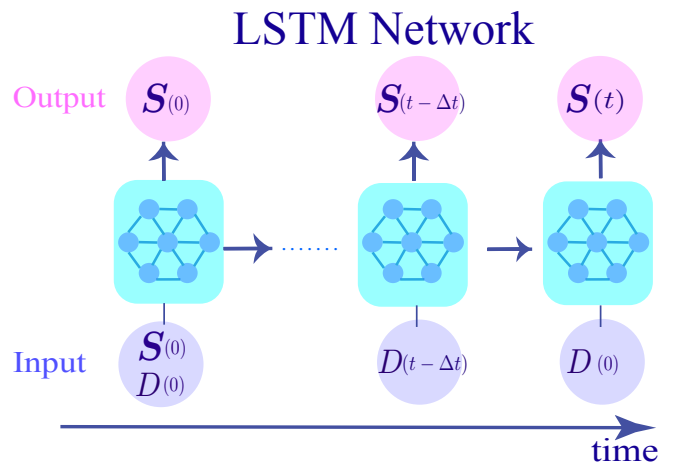
FIG. 2. Schematic representation of our training strategy using a LSTM-NN. Horizontal arrows indicate the content of the internal neural memory being passed to the next time step.
