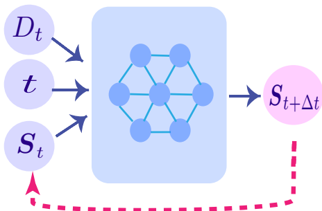
FIG. 9. Schematic representation of the alternative training strategy (“step-wise training”) introduced in the text. The output of the NN (i.e. the predicted evolved expectation values) is fed back as input, generating the dynamics one step at a time.
