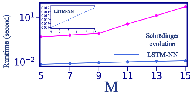
FIG. 7. Runtime versus system size, comparing the time needed for evaluating the NN against direct Schrödinger evolution (evaluated using the qutip implementation). The inset shows the runtime versus system size for the NN in normal scale. The shown results are for TFI model driven by Gaussian random fields up to Jt = 20 .
