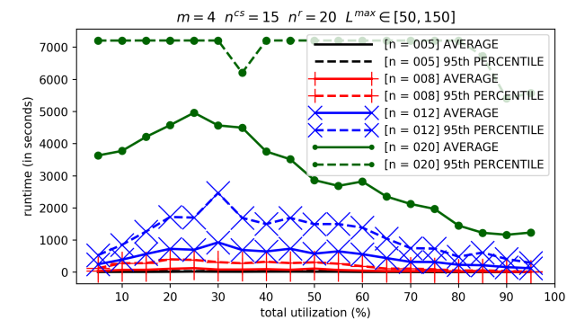
(g) FP-SAG-SR runtime for varying task set size n
