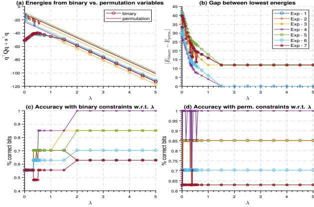
Figure 7. Studying the problem by exhaustive solutions on a classical computer. We solve seven random synthetic problems with n = 3 , m = |\mathcal{V}| = 3 and \sigma = 0.2 by searching over binary variables (binary) or permutation matrices (perm.) exhaustively for the global optimum. We show: (a) the energies attained for both cases, (b) the gap (absolute difference) between the lowest energies in (a), (c) the ratio of correctly guessed bits as a function of the regularizer ( \lambda ) for the binary constraints, (d) same plot in (c) but for permutation matrices. Note, due to significant noise, the global optimum is not always the same as ground truth.
