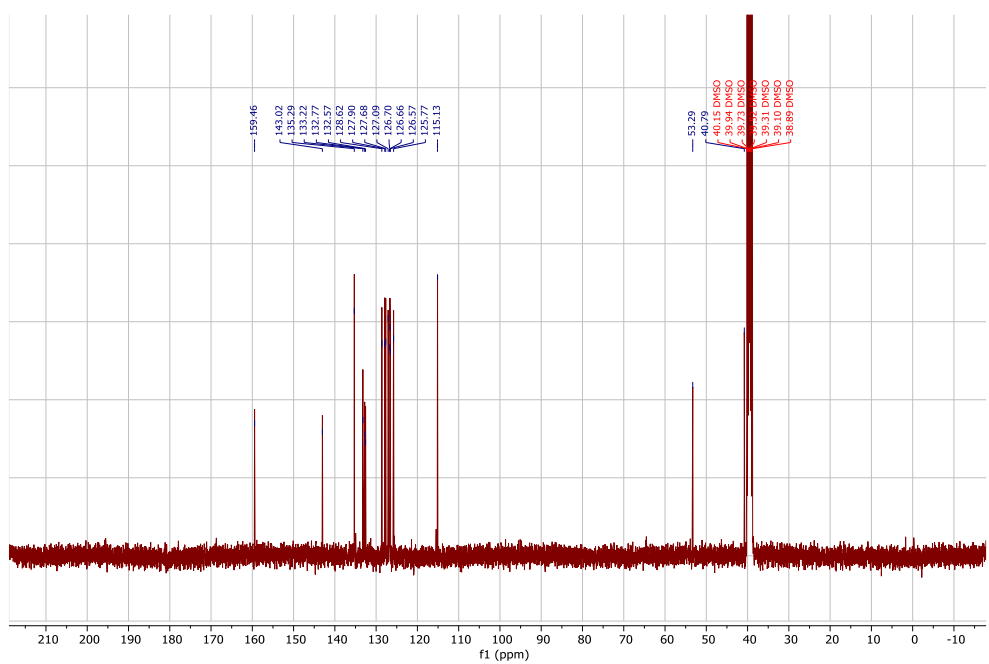
Figure 6.30. 13 C NMR 22
