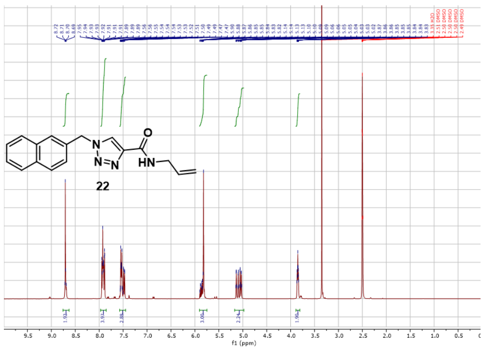
Figure 6.29. 1 H NMR 22
