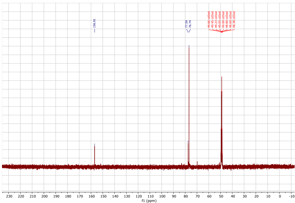
Figure 6.4. 13 C NMR 4
