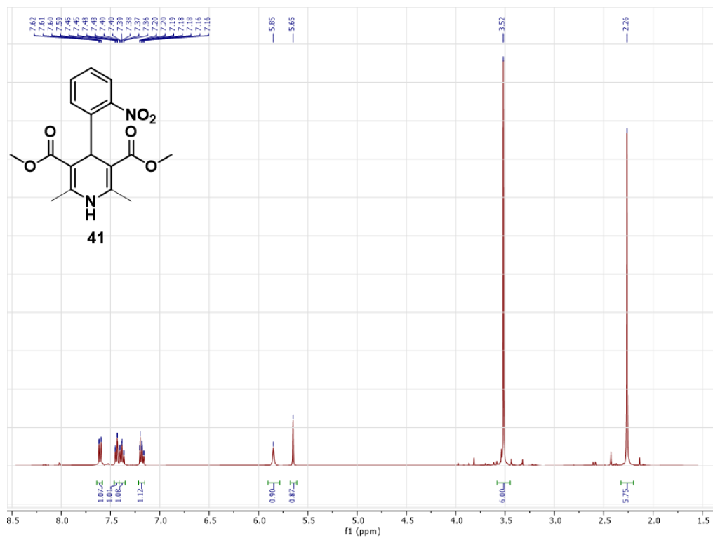
Figure 6.48. 1 H NMR 41
