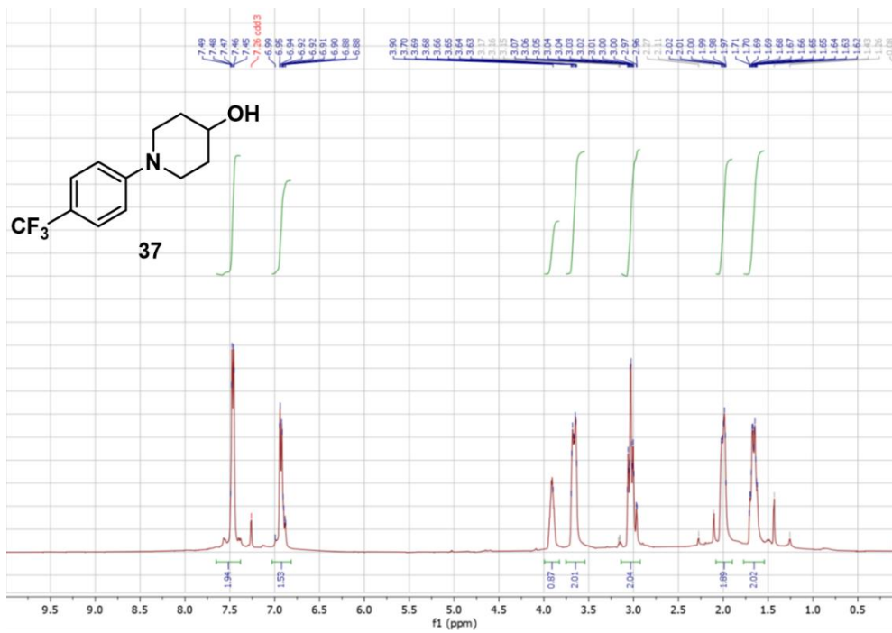
Figure 6.41. 1 H NMR 37
