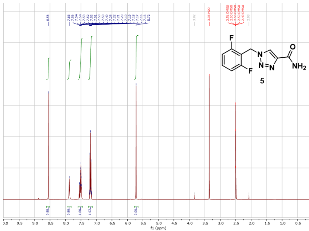
Figure 6.5. 1 H NMR 5
