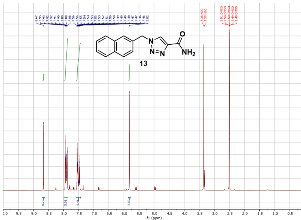
Figure 6.11. 1 H NMR 13
