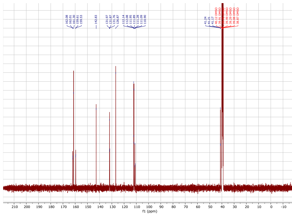
Figure 6.6. 13 C NMR 5
