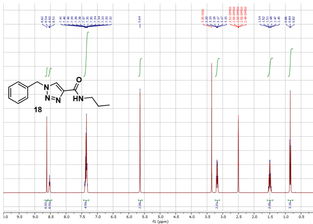
Figure 6.21. 1 H NMR 18
