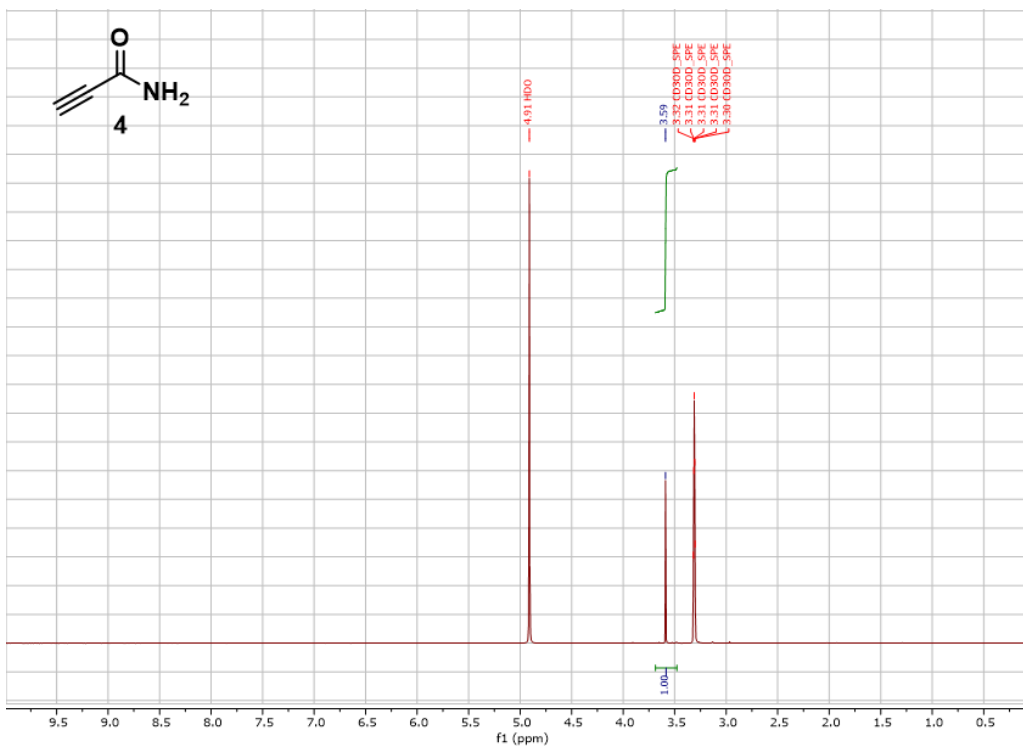
Figure 6.3. 1 H NMR 4
