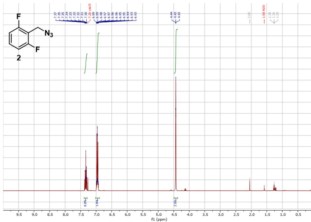
Figure 6.1. 1 H NMR 2
