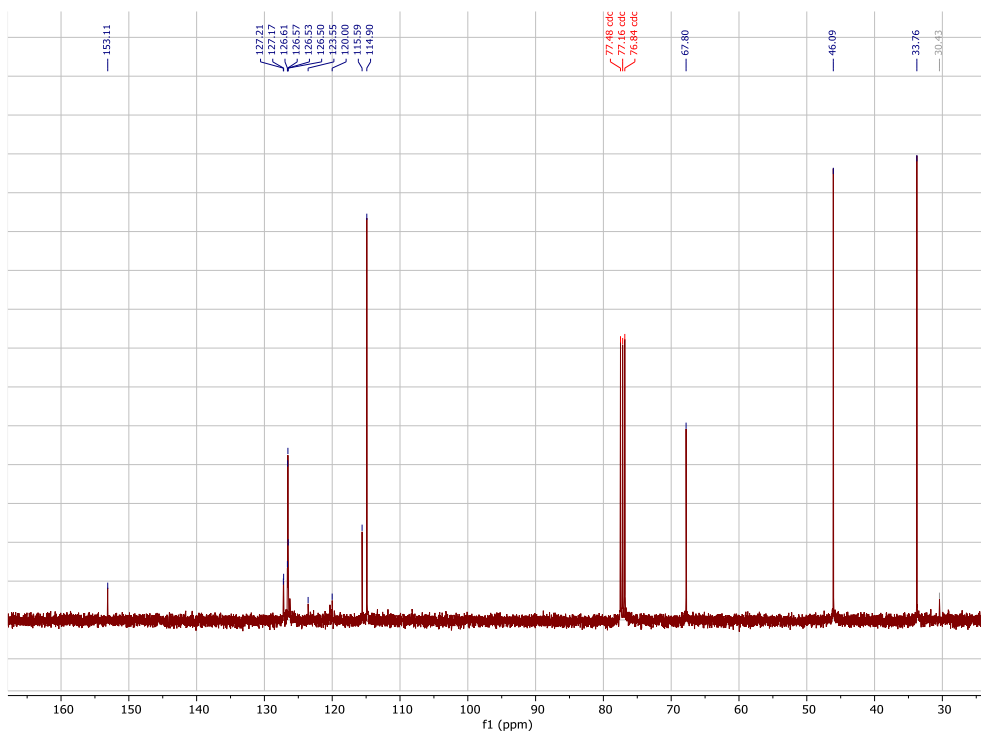
Figure 6.42. 13 C NMR 37
