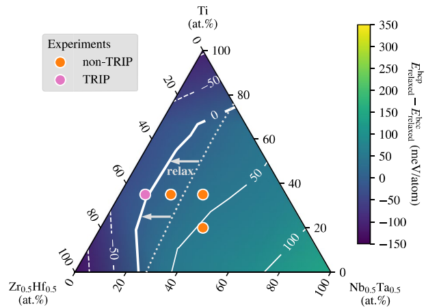
Fig. 7 Ab initio-computed relaxed energy differences between bcc and hcp for the pseudoternary \text{Ti}_x(\text{Zr}_{0.5}\text{Hf}_{0.5})_y(\text{Nb}_{0.5}\text{Ta}_{0.5})_{1-x-y} alloys. Compositions investigated experimentally in ref. 5 are shown by the circles. The thin gray dotted line shows the bcc–hcp equilibrium composition when the atoms are fixed to the ideal lattice sites (cf. Supplementary Fig. 8a). The two arrows highlight the impact of the relaxations. Visualization was performed using MPLTERN 56 .
