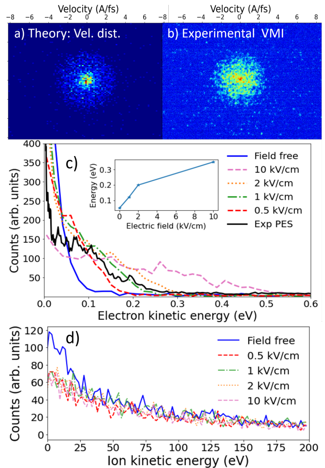
Figure 12. Comparison of theoretical and experimental results. a) Simulated electron velocity distribution for a doped droplet, \text{He}_{2171}\text{Xe}_{23} , exposed to a NIR pulse in an electric field of F = 1000 V/cm. b) Selected experimental electron VMIs for \text{He}_{8000}\text{Xe}_{20} ionized by NIR pulses in the presence of an electric field of 25 V/cm in the interaction region. c) Electron kinetic energy distributions from the simulation (colored lines) and the experiment (black line). d) Corresponding simulated ion kinetic energy distributions.
