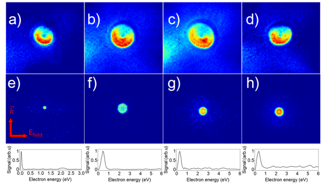
Figure 3. Selected single-shot electron images of Ne clusters. a-d) Large Ne clusters consisting of on average 6000 Ne atoms doped with 10 Xe atoms ionized by a MIR laser pulses. e-h) \text{Ne}_{2000}\text{Xe}_8 and their respective electron spectra (bottom row) ionized by NIR pulses.
