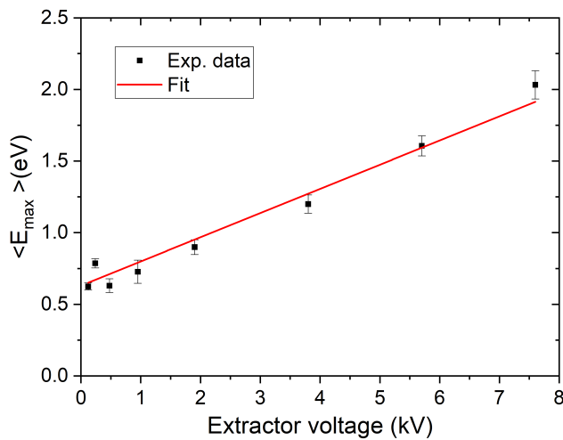
Figure 10. Dependence of the mean electron peak energy on the extractor voltage for \text{He}_{8000}\text{Xe}_{12} irradiated by NIR pulses. The red line is a linear fit of the data.
