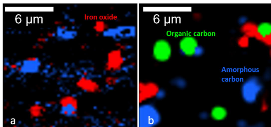
Fig. 9. Raman spectroscopic mapping of samples a) 10C-12O and b) 32C, denoting the regions of iron oxide (red), amorphous carbon (blue) and organic carbon (green).
