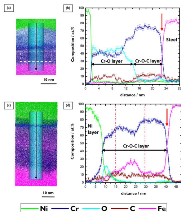
Fig. 4. (a) Three-dimensional APT result of sample 10C-12O, (c) Three-dimensional APT result of sample 32C, (b) and (d) 1-D elemental profile across the coating for the cylindrical ROIs in (a) and (c) respectively.
