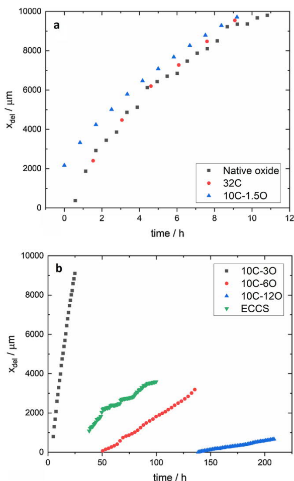
Fig. 14. Position of delamination front vs. time plots for samples a) 10C-1.5O, 32C and pure chromium with native oxide and b) 10C-3O, 10C-6O, 10C-12O and ECCS.
