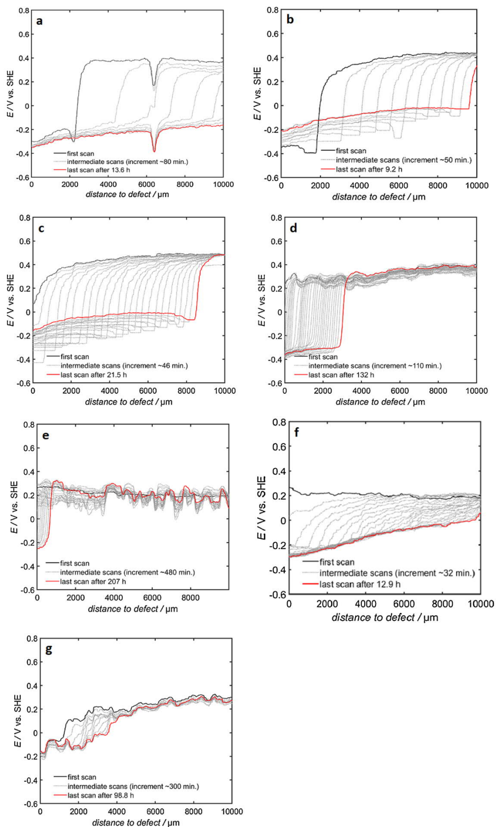
Fig. 13. Corrosion potential (E) plots as a function of distance from the defect obtained from Scanning Kelvin Probe for samples a) 32C, b) 10C-1.50, c) 10C-30, d) 10C-60, e) 10C-120, f) pure Cr with native oxide and g) ECCS.
