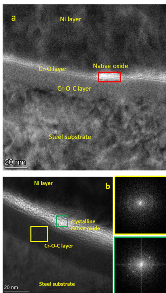
Fig. 3. a) TEM micrograph of the cross-section of the 10C-1.5O sample depicting native oxide formation (red box) and b) Fast Fourier transformations from the amorphous Cr-O-C layer (yellow box) and native oxide (green box) on the 10C-1.5O sample.
