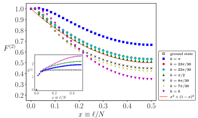
FIG. 2. Rényi entropy of excited states for spin-1 Heisenberg model. In the main panel, different symbols represent the quantity F^{(2)} of first excited state at various k with subsystem size x \equiv l/N . Red line shows the theoretical prediction. Typical Rényi entropy with subsystem size is shown in the inset.
