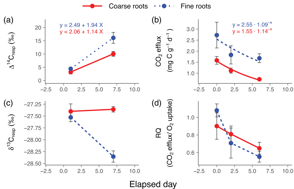
FIGURE 7 Results (mean \pm SE) for coarse roots ( > 2 mm) and fine roots ( \leq 2 mm) from repeated respiration incubations during 7 days. (a) the \Delta^{14}C signature of the respired CO_2 ( \Delta^{14}C_{resp} ). Presented are equations of linear regression models; (b) CO_2 efflux rates. Presented are equations that best fitted the results to the equation y = a \times b^{-x} ; (c) the \delta^{13}C signature of respired CO_2 ( \delta^{13}C_{resp} ); (d) RQ (ratio CO_2 efflux/ O_2 uptake). Results in panels (a) and (c) were measured in two-day flask incubations ( n = 4, 3 for coarse and fine roots, respectively), results in panels (b) and (d) were measured in short-term incubations ( \sim 20 min, according to the consecutive incubations order, n = 3, 4, 3 for coarse roots, and n = 3, 4, 4 for fine roots) [Colour figure can be viewed at wileyonlinelibrary.com ]
