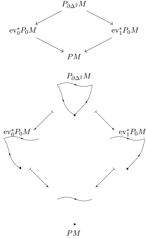
Figure 1: Elements in the spaces P_{\partial\Delta^2}M , ev_0^*P_0M and ev_1^*P_0M .
