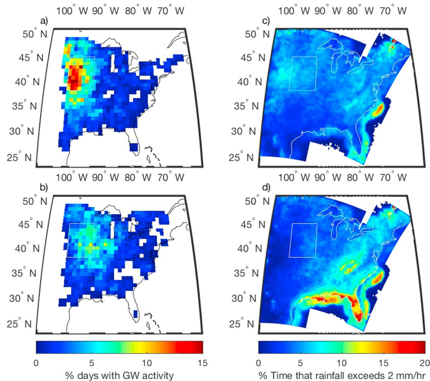
Figure 8. A compilation of occurrence rates of GWs in the 2–6 h frequency band observed at the Earth’s surface during thunderstorm season (May–August) during (a) local night (03:30–09:30 UT) and (b) local day (15:30–21:30 UT). (c and d) The percentage of time rainfall exceeded 2 mm/h during the same time intervals. Note that the color scale used on the left is different than in Figure 7. The area outlined in white in each panel is where surface GW activity is a maximum, from 38 to 45°N and 92 to 99°W.
