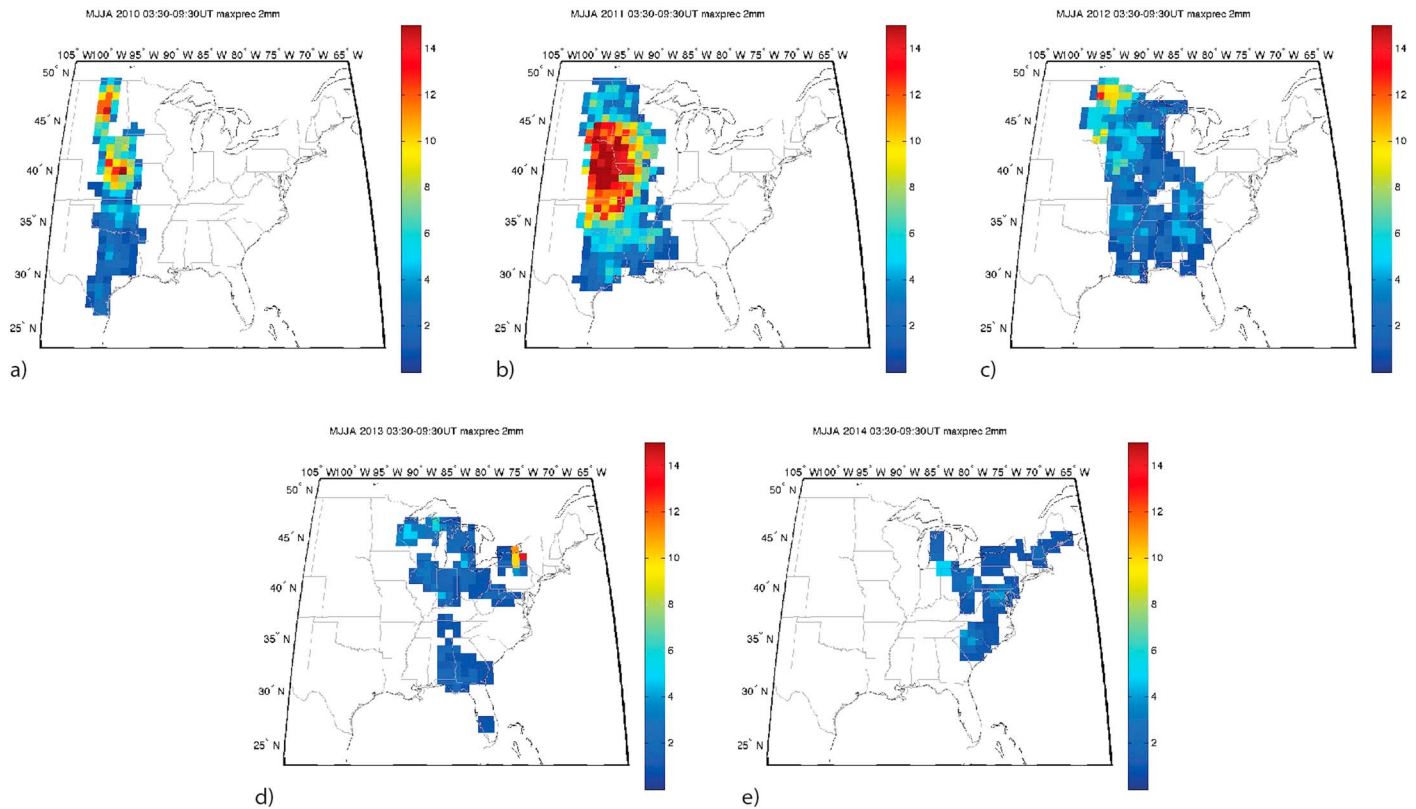
Figure 15. Year-to-year variability of gravity wave occurrence at ground level during the thunderstorm season (MJJA) from 03:30 to 09:30 UT. This time range includes the times shown in Figure 14. The region sampled changes from year to year due to the gradual eastward movement of the TA. Data recorded at times when precipitation exceeded 2 mm/h were excluded from these plots.
