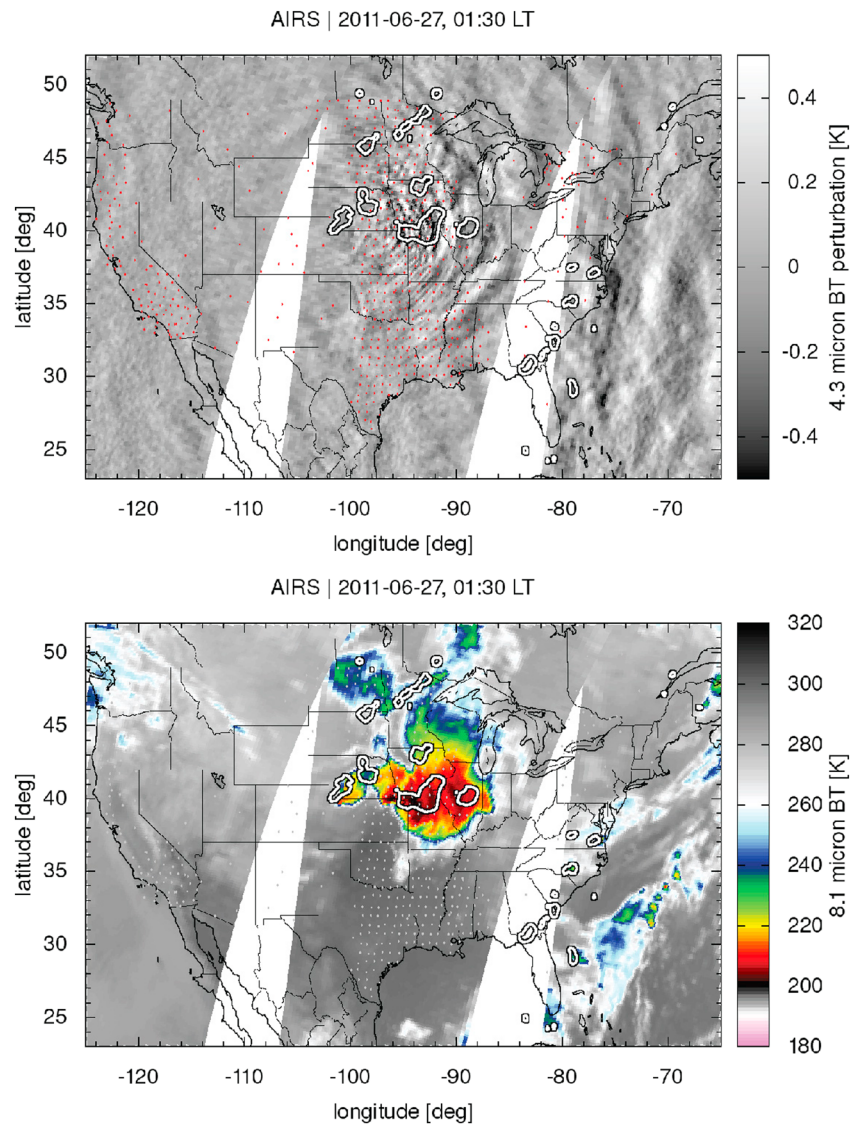
Figure 3. (top and bottom rows) BT perturbations in the 4.3 \mu\text{m} spectral region and BTs in the 8.1 \mu\text{m} spectral region, respectively. These images were taken from AIRS radiance measurements on 27 June 2011 during the nighttime, descending orbit. The contour lines in both panels show 6 mm/h maximum precipitation rates for 0700 UT. The small dots show the TA station locations on that date.
