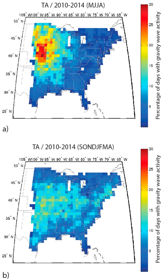
Figure 7. A compilation of the daily mean occurrence rate of GWs in the 2–6 h frequency band observed at Earth’s surface for (a) the 4 months from May through August and (b) the 8 months from September through April during the 5 year time span from 2010 to 2014.
