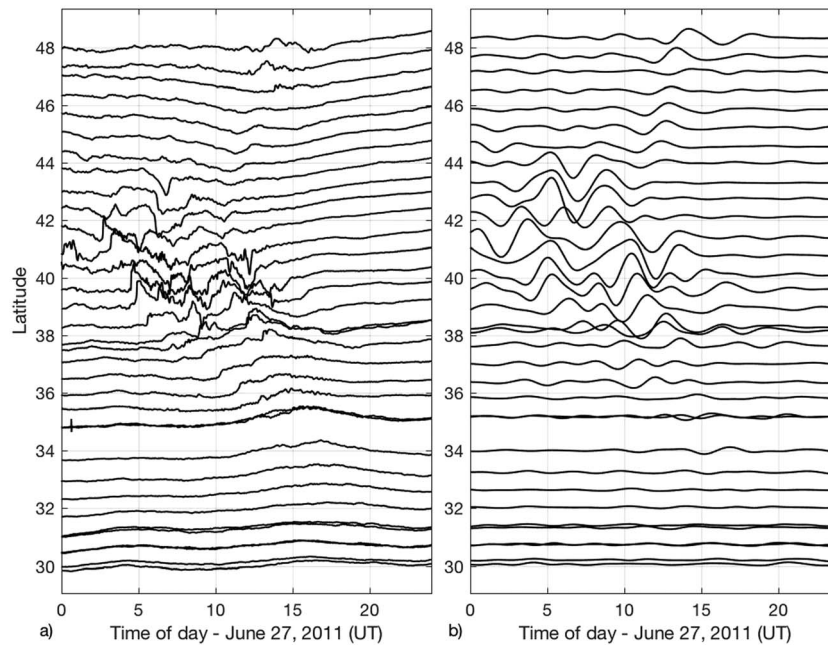
Figure 4. Record section from 27 June 2011 using stations located in a north-south column of the TA between longitudes 93°W and 94°W. Each line is a recording from a single station. (a) Raw data, with a scale of 800 Pa per degree latitude; (b) data bandpassed from 2 to 6 h using a Butterworth filter, with a scale of 400 Pa per degree latitude. Waves with amplitudes ~100 Pa are observed to propagate both northward and southward from a central region near 42°N.
