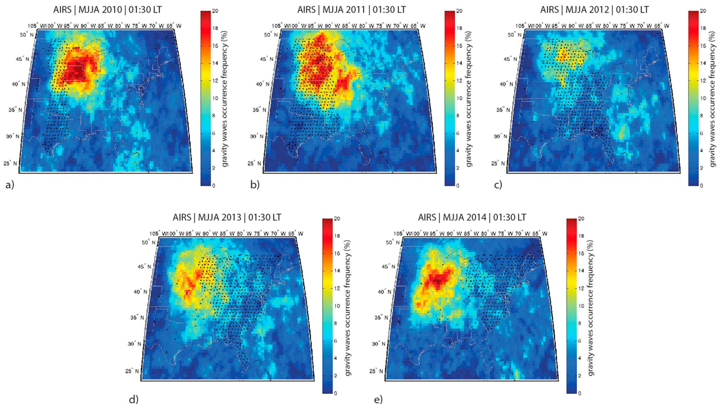
Figure 14. Year-to-year variability of gravity wave occurrence in the stratosphere during the thunderstorm season (MJJA) from observations made by the AIRS sensor during local nighttime, descending orbits. The small black dots represent stations within the TA and show the movement of the network through the years.
