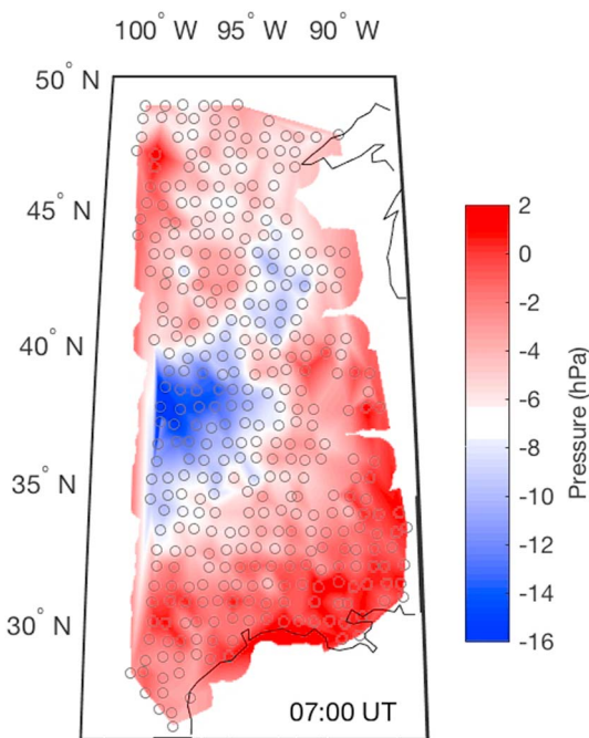
Figure 2. Map of the pressure variations (in hPa) at 0700 UT on 27 June 2011, with long-term mean pressure removed. The pressure at each station, shown by the open circles, is spatially interpolated.
