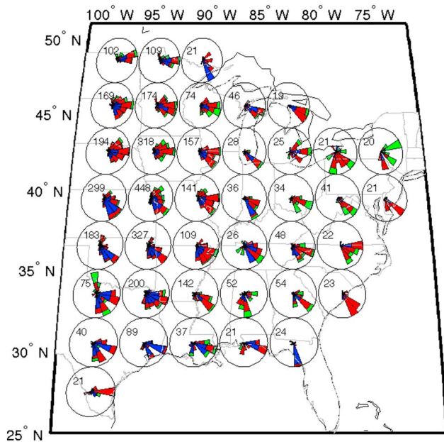
Figure 10. As for Figure 9, but showing phase velocities. The blue color indicates signals with velocities up to 25 m/s, the red color indicates velocities from 25–50 m/s, and the green color indicates higher velocities.
