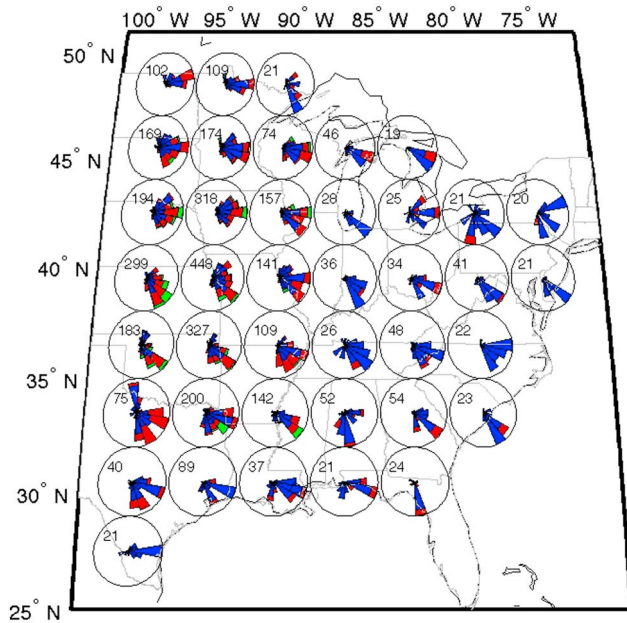
Figure 9. Angle histograms showing direction of propagation and amplitude of coherent waves detected during the thunderstorm seasons, May through August, compiled from 2010 to 2014. The blue color indicates signals with amplitudes from 60 to 100 Pa, the red color indicates amplitudes from 61 to 160 Pa, and the green color indicates larger amplitudes. The total number of detections made for each region is shown to the upper left of each histogram. All detections were made during the local night (from 03:30 to 09:30 UT). The largest waves are seen to the west of the Great Lakes. Most signals propagate in an eastward direction.
