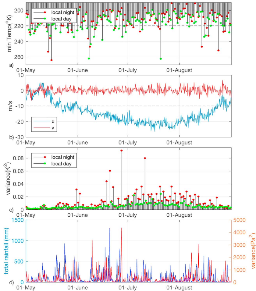
Figure 12. A comparison of observations from the AIRS sensor and the TA pressure sensors and the precipitation statistics for 1 May through 31 August 2011 in the region from 38 to 45°N and 92 to 99°W. (a) The AIRS minimum BT at 8.1 \mu\text{m} , which is a proxy for convective storm activity. Values from the ascending branch (local daytime measurements) are shown in green; the red dots indicate values from the descending branch (local nighttime). A dashed line at 220 K is a typical threshold for detecting deep convection used here as in Hoffmann and Alexander (2010); a variable-threshold approach is used here and in Hoffmann et al. (2013). (b) ERA-Interim zonal and meridional winds at \sim 35 km altitude at 6 h time intervals. The dashed line at 10 m/s marks the stratospheric wind speed; AIRS detections of GWs are not expected at lower wind speeds. (c) The variance of AIRS 4.3 \mu\text{m} BT perturbations, which is a proxy for GW activity in the stratosphere. The values for Figures 12a–12c are taken over the rectangular region from 41–44°N, 92–98°W. (d) The total hourly rainfall in this region (blue) and the variance of pressure perturbations in the 2–6 h band (red) at Earth’s surface. Pressure variance was computed after excluding stations at times when maximum precipitation exceeded 2 mm/h.
