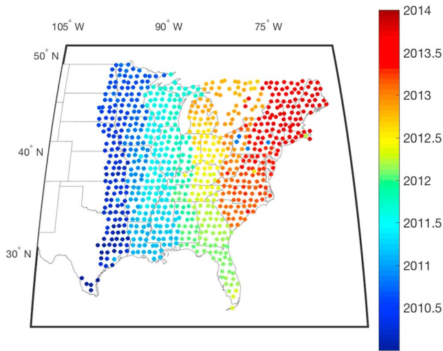
Figure 1. Deployment of stations in the TA that include MEMS sensors. Stations are color coded by the date they began operating. Each station was left in place for approximately 2 years before being moved from the west to the leading (eastern) edge of the network.
