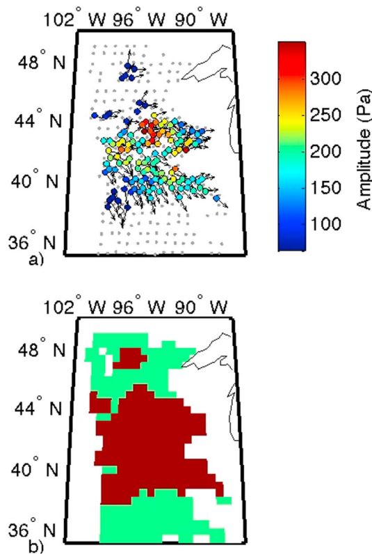
Figure 6. (a) Signal pressure amplitudes and direction of motion detected at the TA within the time period from 03:30 to 09:30 UT on 27 June 2011, coinciding with local nighttime. Each circle represents a coherent GW detection at a single triad, color-coded by the amplitude of the beamformed signal. The arrows show the direction of propagation. Station locations are indicated by gray dots. (b) The green bins show areas where the TA was deployed, but GWs were not detected for this time period. The dark red bins show areas where detections were made.
