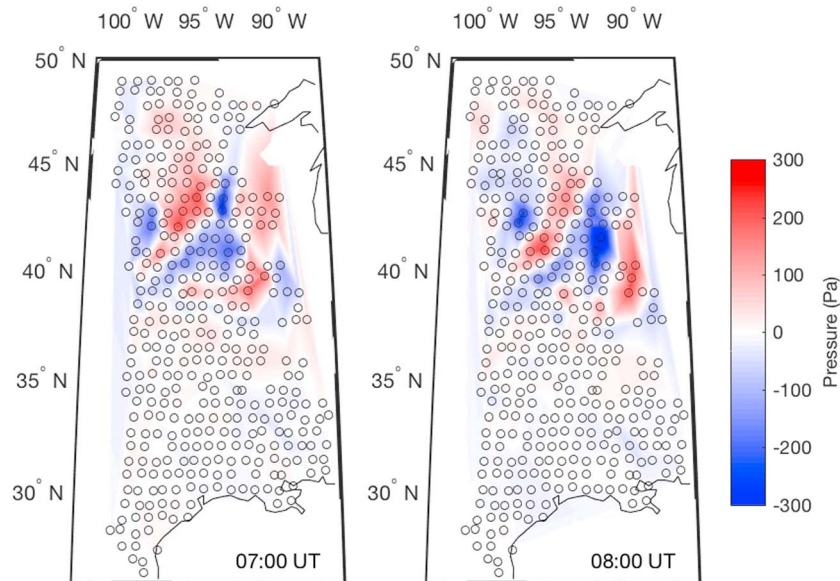
Figure 5. Maps of the pressure variations (in Pa) in the 2–6 h band at 2 times (0700 and 0800 UT) on 27 June 2011. The bandpassed pressure measurements are spatially interpolated between stations, shown by the open circles.
