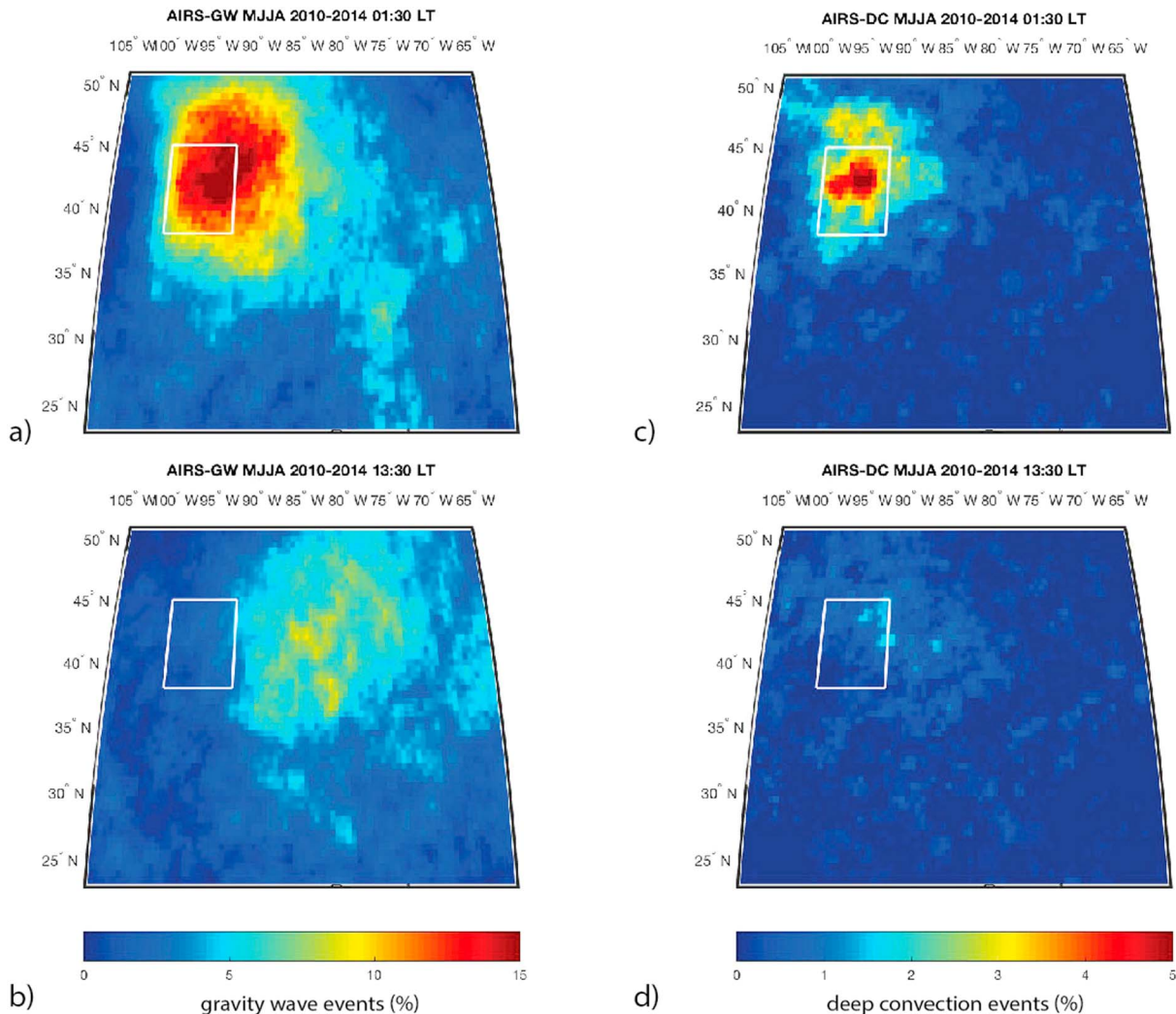
Figure 11. (left column) The occurrence frequency of GWs in the stratosphere is shown over the entire study area from observations made by the AIRS instrument during May through August from 2010 through 2014. Results from (a) descending orbits during the local nighttime and (b) ascending orbits during the local daytime are shown. The occurrence frequency of deep convection events for the (c) descending and (d) ascending orbits. The bins in these images are 0.5^\circ on a side. The area outlined in white in each panel is where convective activity at nighttime is a maximum, from 38 to 45^\circ\text{N} and 92 to 99^\circ\text{W} .
