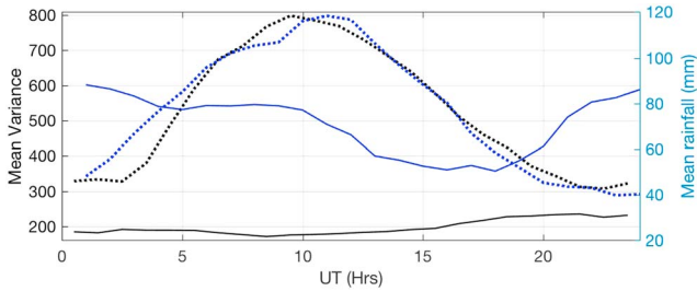
Figure 13. Mean TA pressure variance ( \text{Pa}^2 ) and total rainfall per hour in two rectangular regions near the Great Lakes during the thunderstorm season, MJJA. The heavy dashed curves represent observations from 38 to 45°N and 92 to 99°W; the black color is the mean hourly pressure variance in 2011, and the blue color is the average total rainfall during this same period. The solid curves are from observations made in the same latitude range in 2013 but in the much less active area from 82 to 89°W, with the black and blue lines representing the pressure variance and total rainfall, respectively.
