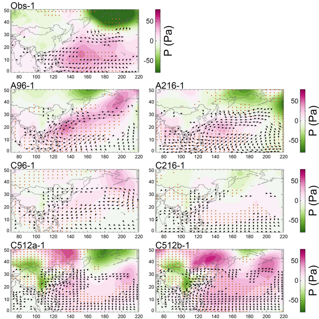
Figure 9. Regressions of P_{SF} (shading) and 850 hPa wind (arrows) against normalised MAM EOT time series corresponding to Obs-1. Stippling indicates confidence levels exceeding 90 %. Wind arrows are drawn when at least one component is statistically significant and the wind speed exceeds 0.1 \text{ m s}^{-1} .
