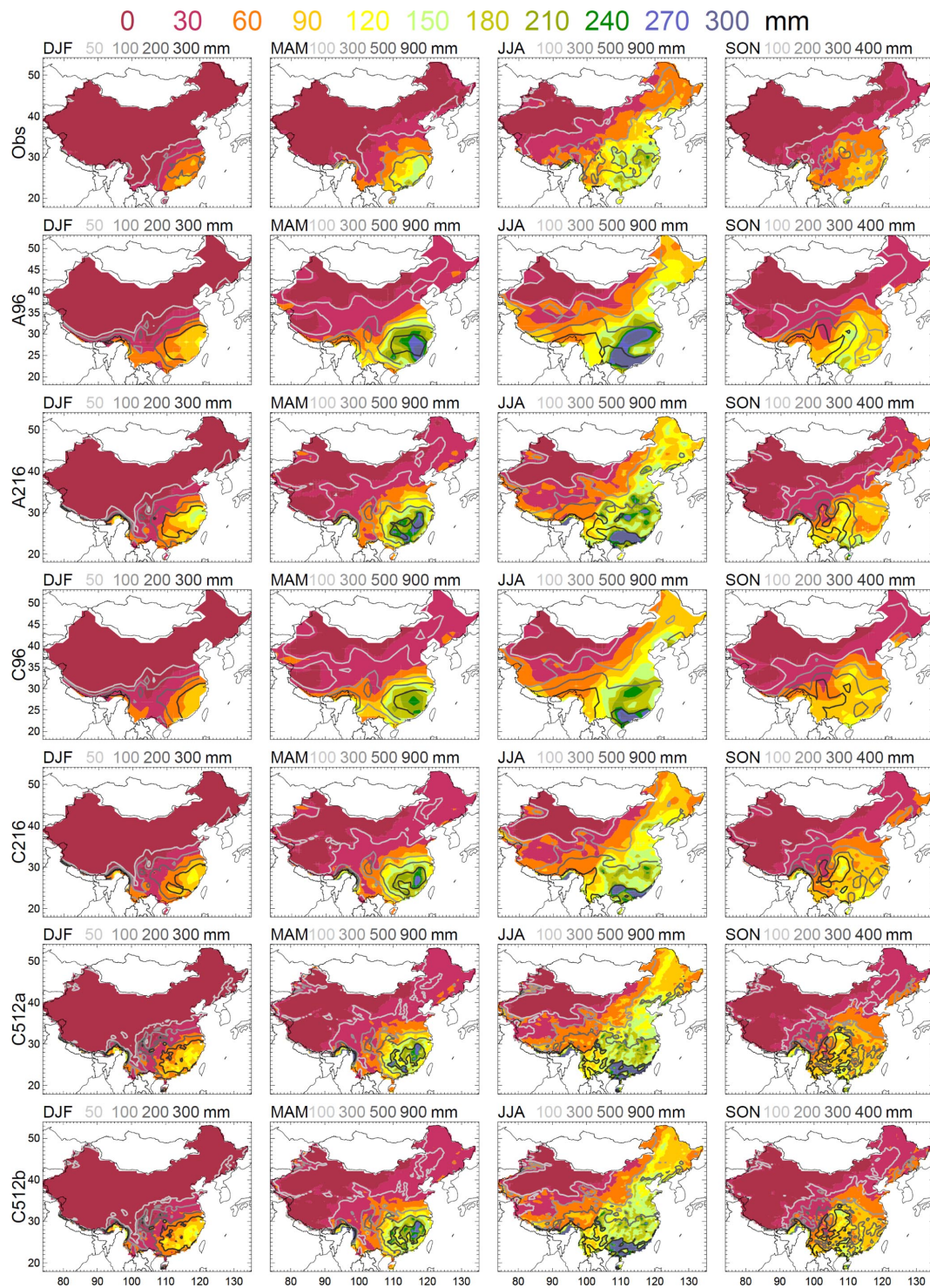
Figure 2. Climatological seasonal total precipitation (grey contours) and interannual standard deviation (shading) for 1951–2007 observations (top) and the full length of each simulation. The season is indicated above the panels.
