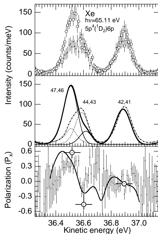
FIG. 2. Experimental results for the decay of Xe 4d_{5/2}^{-1}6p(J=1) to the multiplet of 5p^4(^1D_2)6p states. Top panel: spin separated intensities I_+ , I_- derived from 10 meV wide intervals of the measured spectra (open symbols: I_+ ); middle panel: I_+ , I_- from our least squares analysis (solid lines: I_+ , bold solid line: sum of the two underlying components for I_+ , dotted and dot-dashed lines: I_- ); bottom panel: spin polarization data derived analogous to the top panel (dots) and spin polarization results of the least squares analysis (solid line and open symbols).
