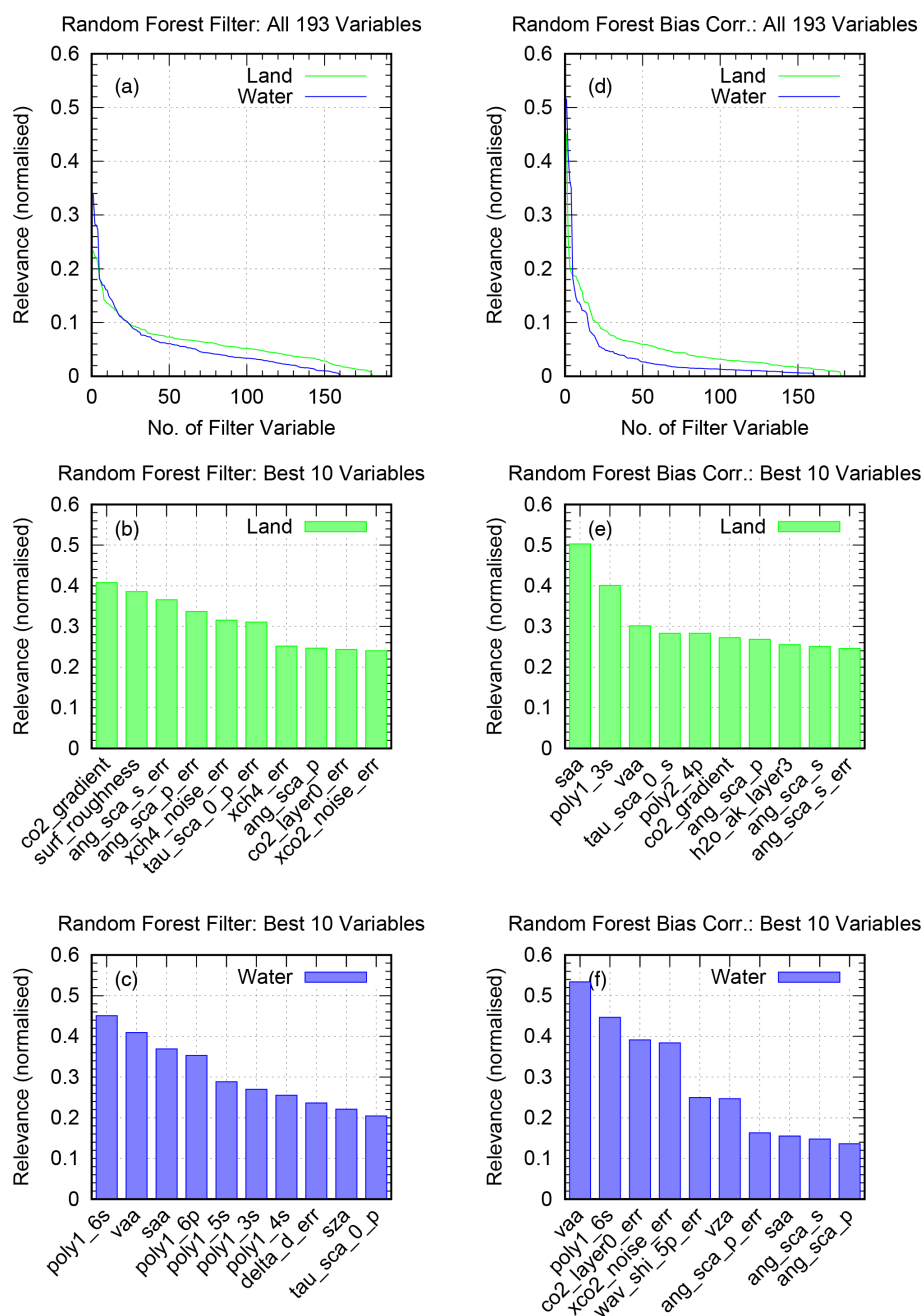
Figure 5. Random forest results for GOSAT. (a–c) Results from the random forest filter. (d–f) Results from random forest bias correction. (a, d) Normalised relevance (score) of all filter variables. (b, e, c, f) Selected variables and their relevance for the land and water surfaces.
