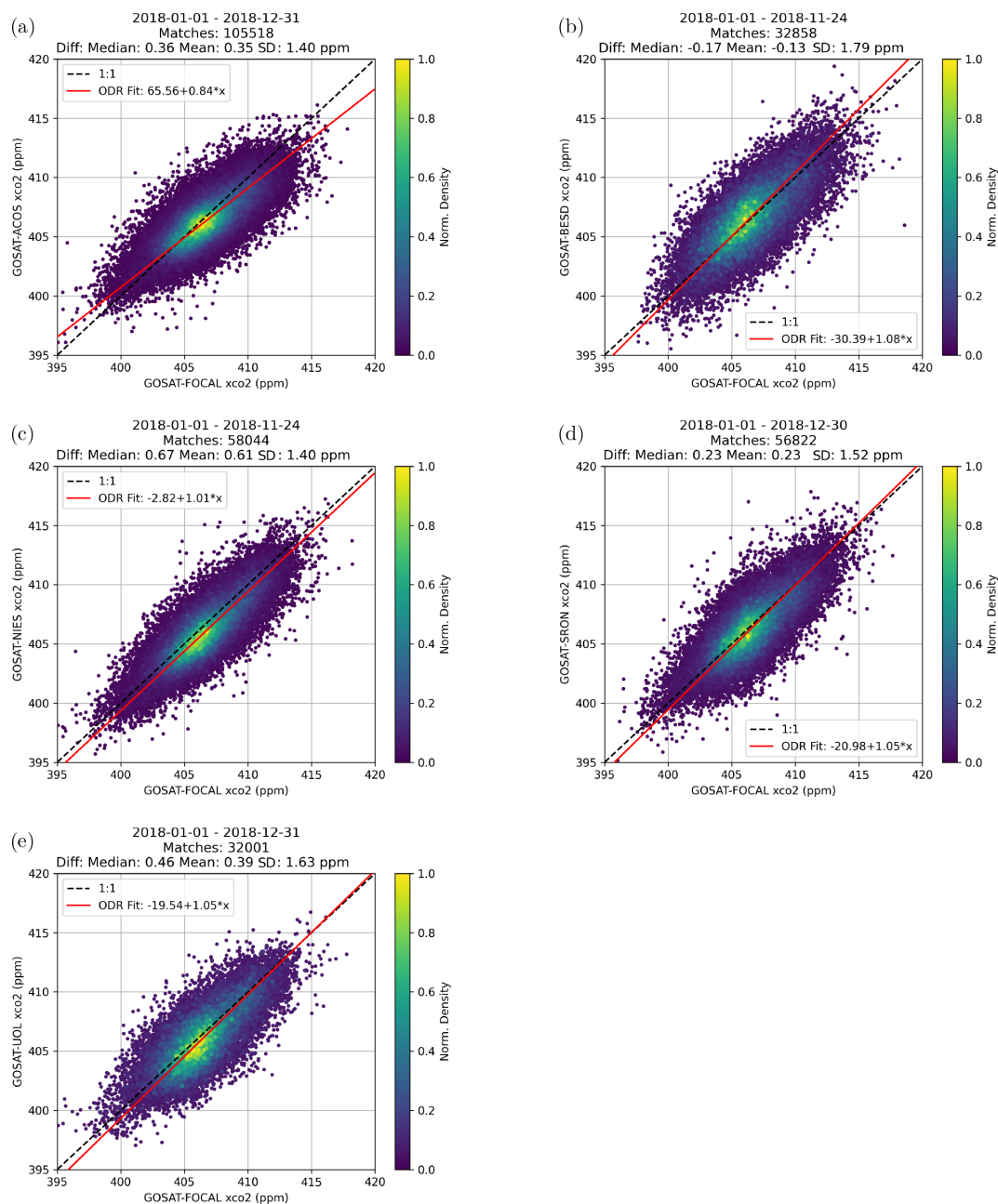
Figure 14. Comparison of GOSAT-FOCAL data ( x axis) from 2018 with other GOSAT data ( y axis). The colour of the data points corresponds to the density of data points at that location (normalised to a maximum value of 1). The dashed line corresponds to perfect agreement. The red line shows the result of a linear fit using the orthogonal distance regression (ODR) method. The total number of collocated data as well as the median, mean, and standard deviation of the XCO 2 differences between the two data sets are given in the title of the sub-plots. (a) FOCAL vs. ACOS. (b) FOCAL vs. BESD. (c) FOCAL vs. NIES. (d) FOCAL vs. SRON. (e) FOCAL vs. UoL.
