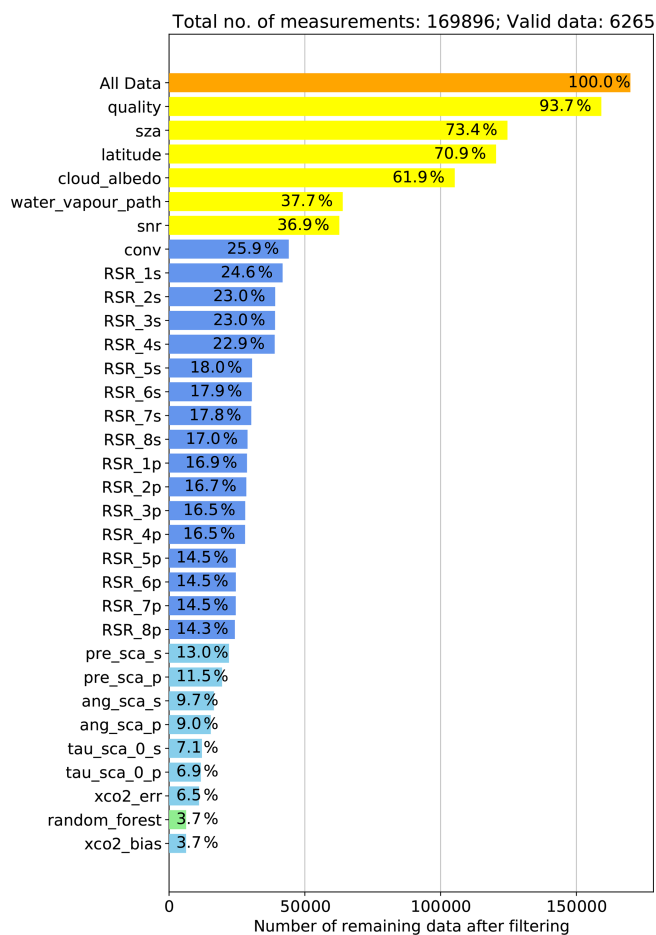
Figure 3. Same as Fig. 2, but for GOSAT-2.
