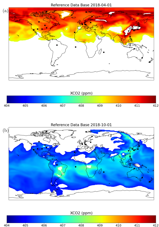
Figure 1. XCO 2 from the GOSAT-FOCAL reference database. The black markers show the locations of TCCON stations. (a) 1 April 2018. (b) 1 October 2018.
