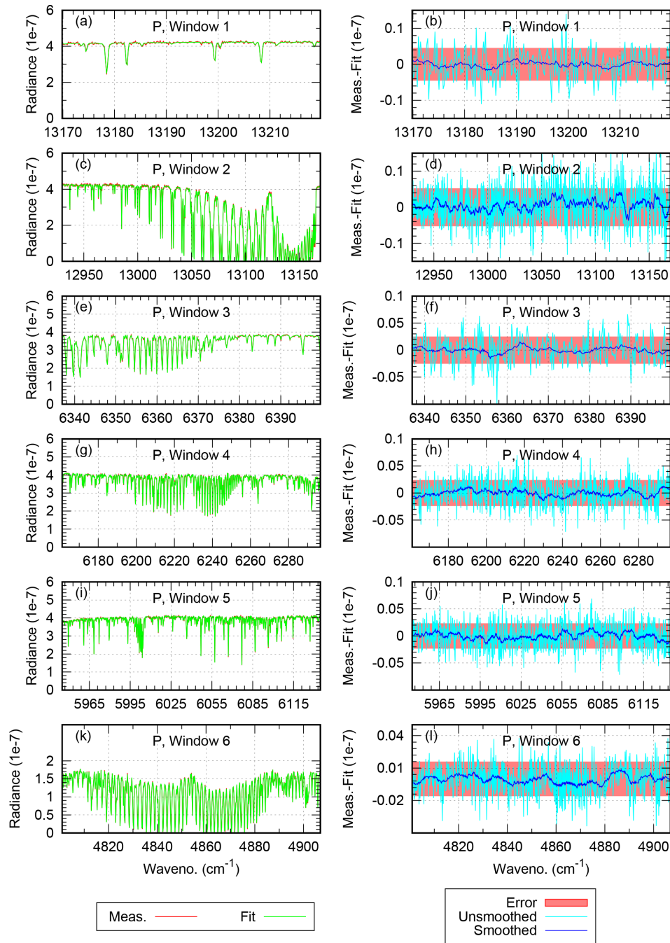
Figure 8. Example for a single GOSAT measurement (P polarisation): (a, c, e, g, i, k) measured (red) and retrieved (green) spectra in the different fit windows; because of the good agreement the red curve is essentially barely visible below the green curve. (b, d, f, h, j, l) Corresponding residuals (measurement – fit). Light blue: unsmoothed. Blue: smoothed with a boxcar width of 21 spectral pixels (= 4.2 cm -1 ). Red: estimated noise error range. The radiance unit is W cm -2 cm sr -1 .
