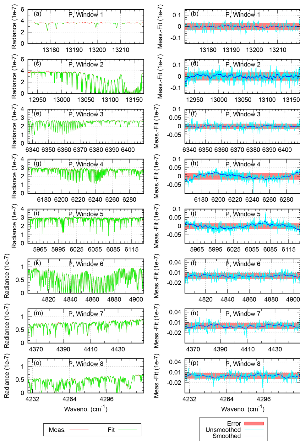
Figure 9. Same as Fig. 8, but for GOSAT-2.
