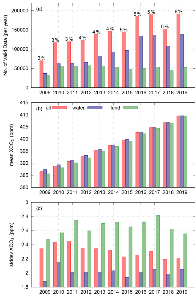
Figure 10. Statistics for valid GOSAT measurements (after pre- and post-processing filtering) for each year. Blue: measurements over water. Green: measurements over land. Red: all data. (a) Number of valid measurements, including the percentage of all originally available measurements. (b) Global mean XCO 2 . (c) Corresponding standard deviation.
