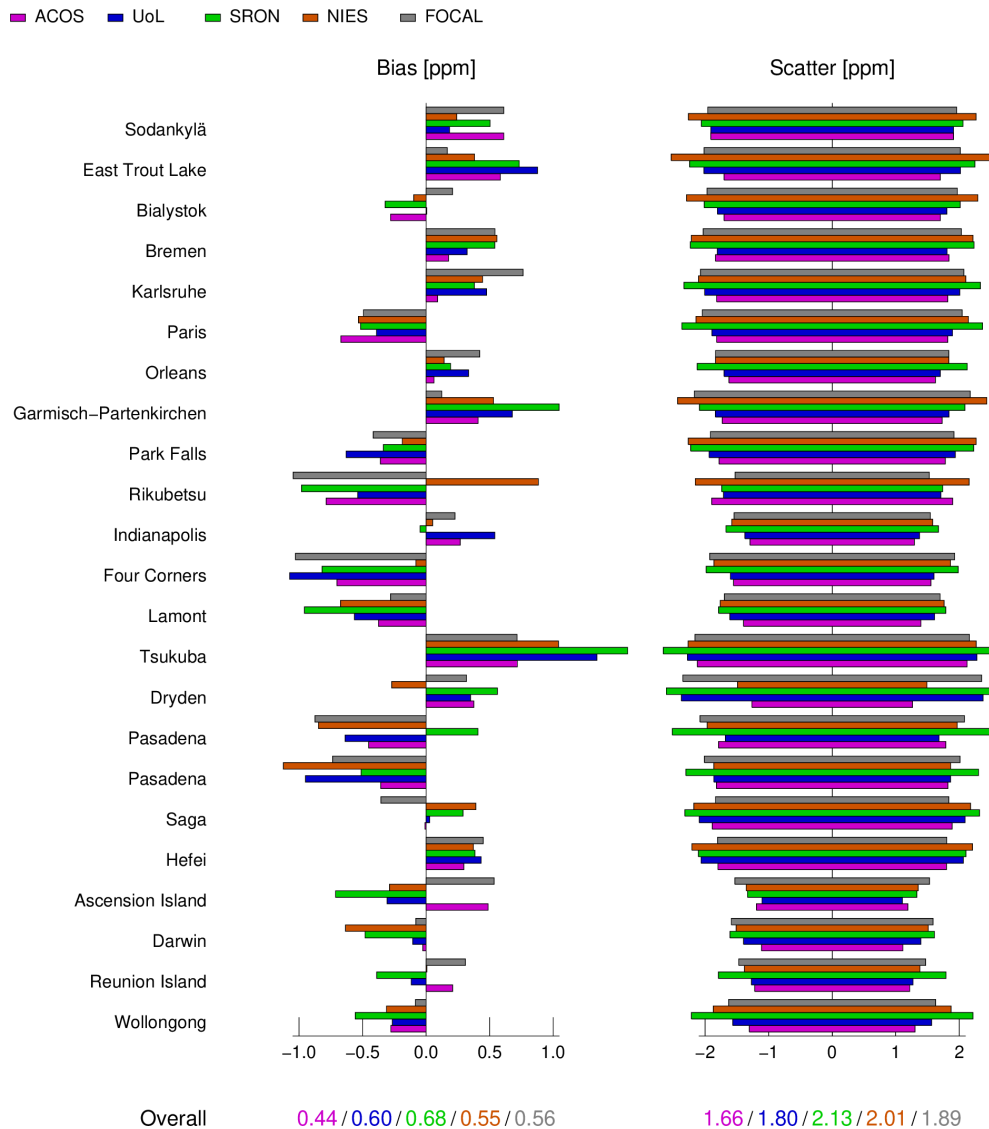
Figure 16. Overview of TCCON validation results for GOSAT.
