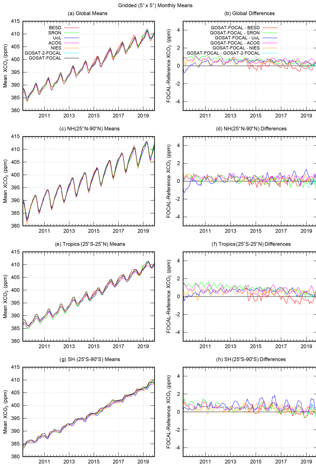
Figure 20. Gridded monthly mean time series of different GOSAT XCO 2 products. (a, c, e, g) Time series of mean XCO 2 for four different regions (from top to bottom: global, Northern Hemisphere, tropics, Southern Hemisphere). (b, d, f, h) Corresponding differences to the GOSAT-FOCAL product.
