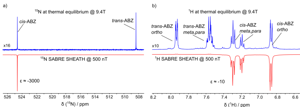
Figure 5. ^{15}\text{N} NMR spectra (a) and ^1\text{H} NMR spectra (b) showing comparison of ^{15}\text{N},^{15}\text{N}'\text{-ABZ} signals in thermal equilibrium (blue, absorption peaks) and after SABRE SHEATH hyperpolarization at 500 nT (red, emission peaks). The phases in SABRE SHEATH spectra were set with respect to corresponding thermal spectrum. The ^{15}\text{N} NMR spectrum at thermal equilibrium shown in (a) was averaged for 128 times. Otherwise, all the compared spectra were acquired with identical acquisition and processing parameters. The experimental protocol for the SABRE experiments is shown in Figure 2a.
