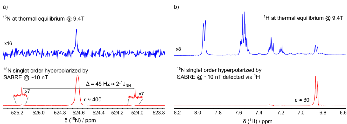
Figure 7. ^{15}\text{N} NMR spectra (a) and ^1\text{H} NMR spectra (b) showing comparison of ^{15}\text{N},^{15}\text{N}'\text{-ABZ} signals in thermal equilibrium (blue) and after SABRE SHEATH hyperpolarization at 10 nT of the singlet order of the ^{15}\text{N} spin pair (red). The thermal spectrum in (a) was acquired in 4 scans with proton decoupling. This narrowed the line and increased SNR. Hyperpolarized ^{15}\text{N} spectrum exhibits outer singlet-triplet coherences. The experimental protocol for the SABRE experiments is shown in Figure 2b.
