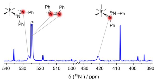
Figure 4. Fragments of the ^{15}\text{N} NMR spectrum showing signals of ^{15}\text{N},^{15}\text{N}'\text{-ABZ} in Ir-Imes complexes, polarized by SABRE SHEATH at 500 nT. The phase of the spectrum was adjusted to have absorptive signals. The experimental protocol is shown in Figure 2a.
