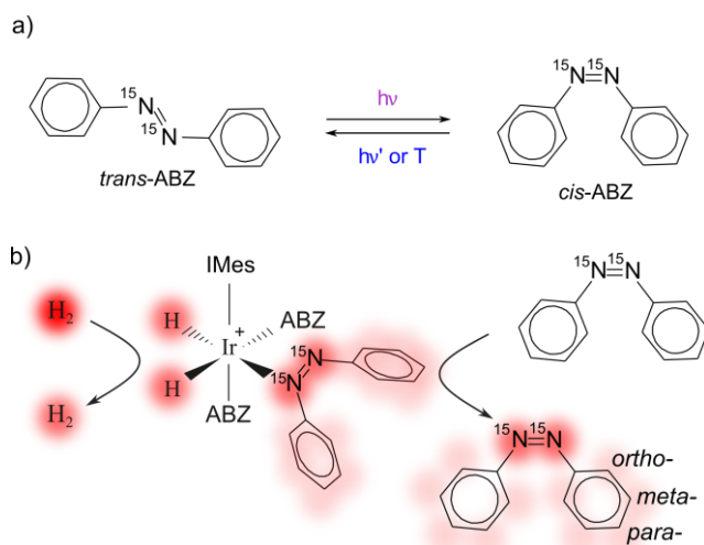
Figure 1. (a) Chemical structure and photochromic property of azobenzene (ABZ). (b) Scheme of SABRE with cis -ABZ showing polarization transfer from a parahydrogen molecule to cis -ABZ within a reversibly formed Ir-Imes activated complex.
