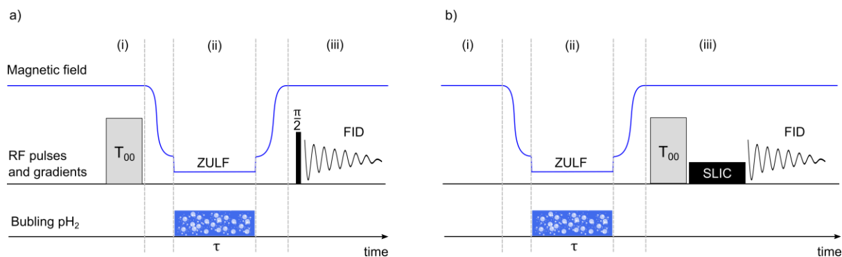
Figure 2. Experimental protocols. (a) Field cycling in a SABRE SHEATH experiment with consecutive (i) destruction of equilibrium magnetization at the high field of the NMR spectrometer, followed by transfer of the sample into the magnetic shield, (ii) bubbling parahydrogen at ZULF conditions in a variable magnetic field for a time \tau , and (iii) backward transfer of the sample and excitation of the NMR signals by a hard pulse. (b) Field cycling in a SABRE SHEATH experiment to observe hyperpolarized singlet order of the 15 N spin pair in cis - 15 N, 15 N'-ABZ. In this case, excitation is performed by using a SLIC pulse (see in the text). The T_{00} block indicates a filter based on 90° pulses with pulsed field gradients; for details see reference 19 .
