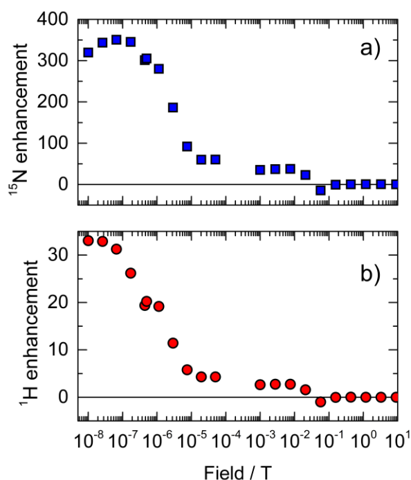
Figure 8. Field dependence of ^{15}\text{N} NMR signals (a) and ^1\text{H} NMR signals (b) corresponding to singlet order of the ^{15}\text{N} spin pair in cis - ^{15}\text{N},^{15}\text{N}' -ABZ hyperpolarized by SABRE SHEATH. The experimental protocol for the SABRE experiments is shown in Figure 2b. All the functions were normalized by the integral intensity of the corresponded signal intensity at thermal equilibrium.
