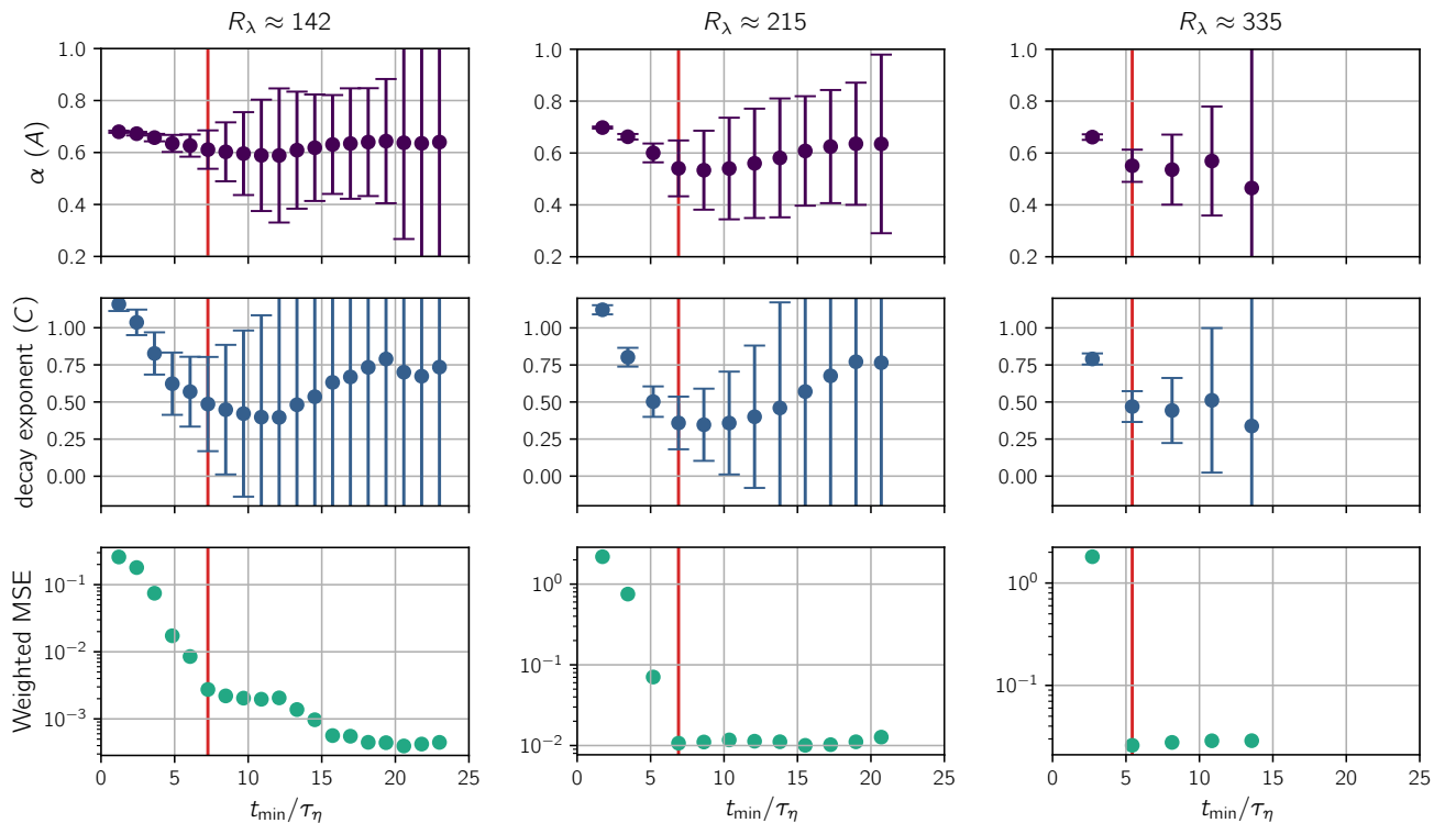
Supplementary Figure S5. Different fit choices for extrapolating the steepest-descent minimum. We use the simple decay function (B3) to capture the evolution of the minima for different finite-time Cramér functions. In order to obtain a satisfactory fit, it is helpful to leave out a transient regime of data points t < t_{\min} until only the asymptotic behavior is captured by the fit. Here we show the resulting values of \alpha = A (top) and the decay exponent C (middle) for different choices of t_{\min} in all of the simulations (left to right). The time scale B is not shown. We justify the choice of t_{\min} by computing the weighted mean squared error (MSE, bottom) given by \sum_{i=1}^N (\delta_i/\sigma_i)^2/(N-3) , where N is the number of data points included, \delta_i are the fit errors and \sigma_i the standard deviations (error bars) of the data points. The quantity \sum_{i=1}^N (\delta_i/\sigma_i)^2 is minimized by the fit, which we divide by the number of degrees of freedom N-3 for comparison. We choose t_{\min} as the start of the first plateau of the weighted MSE (red lines).
