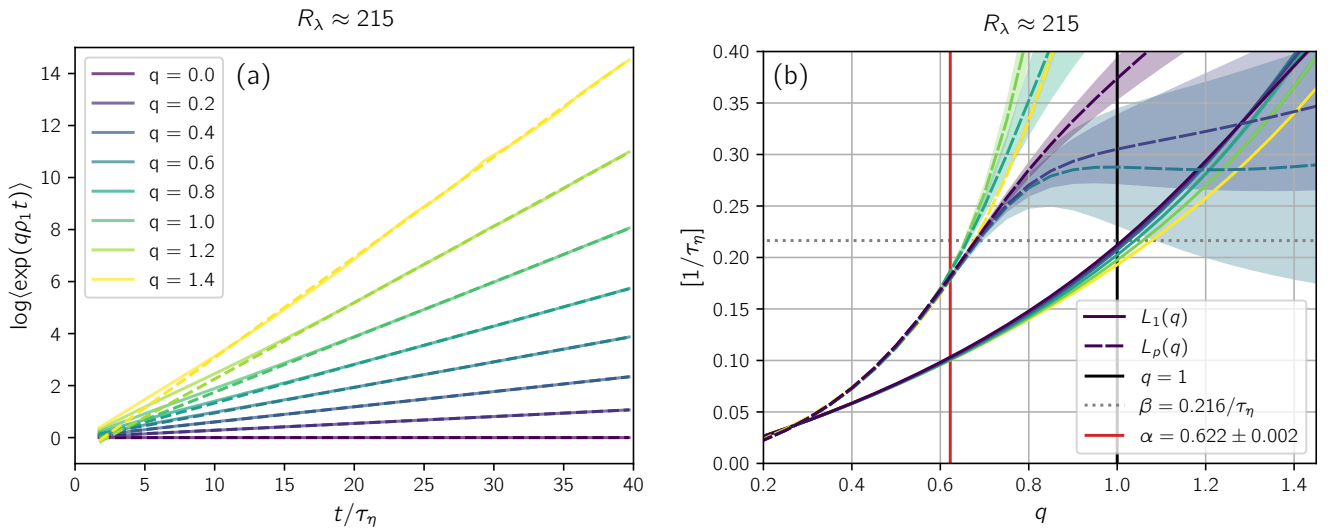
Supplementary Figure S6. Generalized Lyapunov exponents in the main simulation. (a) Plotting the cumulant-generating function of \rho_1(t)t for fixed argument q as a function of time (solid lines), the GLE can be estimated as the asymptotic slope of the curve by an affine fit of the interval t \in [20\tau_\eta, 40\tau_\eta] (dashed lines). (b) Generalized Lyapunov exponents can be used to estimate \beta and \alpha . The first standard GLE L_1(q) (solid lines) is shown for t_{\max} ranging from 12.08\tau_\eta (yellow) to 39.68\tau_\eta (violet). The curvature peak GLE L_p(q) is shown for the same times (dashed lines). For comparison, we also show the line q = 1 (solid, black), the value of \beta estimated from curvature peak number (dotted, grey) and the value of \alpha estimated from the curvature PDF (solid, red).
