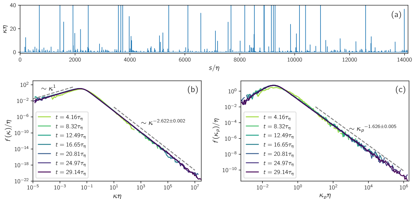
FIG. 2. Curvature peaks are localized extreme events along the loop. (a) Curvature along a material loop at t = 29.14\tau_\eta as a function of arc length s . The function is highly spiked, indicating that high curvature only occurs in isolated narrow regions. These isolated peaks contribute to the high-curvature tails of the curvature PDF. (b) Curvature PDF of material loops at times t = 4.16\tau_\eta (light green) up to t = 29.14\tau_\eta (violet). (c) PDF of curvature peaks of material loops at the same times. The high-curvature regime is fitted by power laws in the regions indicated by the dashed lines using binomial error estimates.
