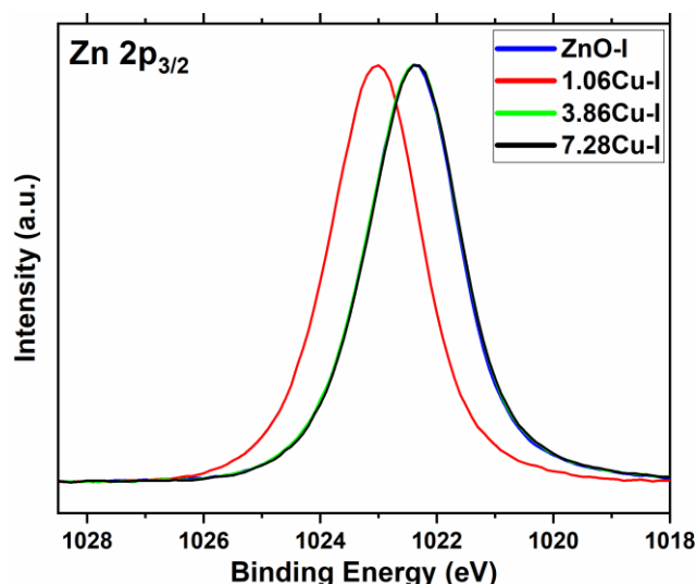
SI 5.34: Zn 2p spectra of some Cu-I series samples.
