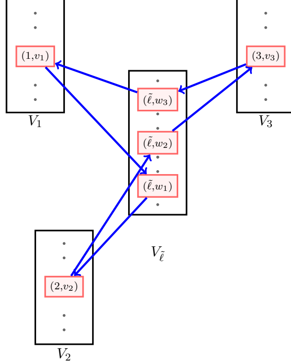
Figure 2: Illustration of the first part of the construction. The cycle in the figure visits the parts V_1 , V_2 and V_3 exactly once and the part V_{\tilde{\ell}} three times. It is given by (\tilde{\ell}, w_3) \rightarrow (1, v_1) \rightarrow (\tilde{\ell}, w_1) \rightarrow (2, v_2) \rightarrow (\tilde{\ell}, w_2) \rightarrow (3, v_3) \rightarrow (\tilde{\ell}, w_3) .
