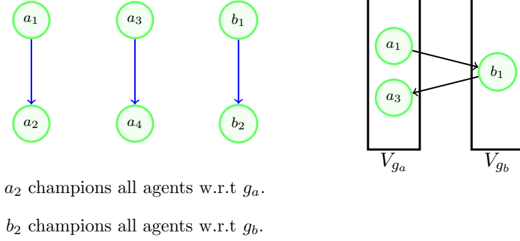
Figure 1: Illustration of a group champion graph. We have an instance with six agents \cup_{i \in [4]} a_i and \cup_{i \in [2]} b_i and two unallocated goods, namely g_a and g_b . The agents \cup_{i \in [4]} a_i find g_a valuable and the agents \cup_{i \in [2]} b_i find g_b valuable. The envy graph E_X of the instance is shown on the left side. E_X shows that s(a_2) = a_1 , s(a_4) = a_3 , and s(b_2) = b_1 . Also, we have that agent a_2 champions all the agents w.r.t g_a and b_2 champions all the agents w.r.t g_b . The group champion graph (right) has two parts, V_{g_a} corresponding to g_a and V_{g_b} corresponding to g_b . V_{g_a} contains the sources of all the agents that find g_a valuable, namely a_1 and a_3 . Similarly, V_{g_b} contains b_1 . There is an edge from a_1 to b_1 as a_2 (which is reachable from a_1 in E_X ) champions b_1 w.r.t to g_a . Similarly, there is an edge from b_1 to a_3 as b_2 (which is reachable from b_1 in E_X ) champions a_3 w.r.t to g_b .
