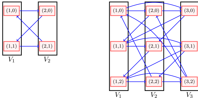
Figure 4: Illustration of the construction of d -partite graph G that satisfies all the conditions in Definition 2, for d = 2 (left) and d = 3 (right).
