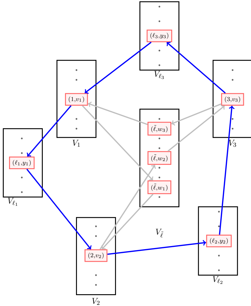
Figure 3: Illustration of the existence of a cycle that visits every part at most once. We take the instance in Figure 2, where there exists a cycle C that visits every part other than V_{\tilde{l}} at most once. The edges of the cycle C are light gray color in color. The figure shows how to obtain a cycle C' that visits every part at most once from C . The edges of C' are blue in color. For all i \in [3] , we replace the subpath in C of the form (i, v_i) \rightarrow (\tilde{l}, w_i) \rightarrow (i+1, v_{i+1}) ( 3+1 is to be interpreted as 1) by (i, v_i) \rightarrow (\ell_i, y_i) \rightarrow (i+1, v_{i+1}) to get C' .
