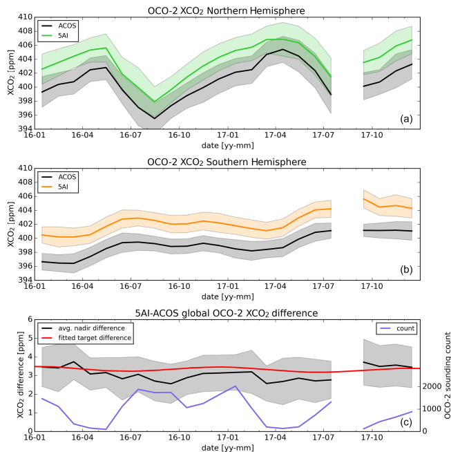
Figure 7. Temporal variation in 5AI and the raw ACOS B8r retrieved X_{CO_2} in the Northern Hemisphere (a), Southern Hemisphere (b), and the global difference (c). Panel (c) compares 5AI–ACOS difference for nadir and target OCO-2.
