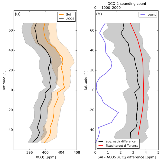
Figure 6. Latitudinal variation in 5AI and the raw ACOS B8r retrieved X_{CO_2} (a) and their difference (b). Panel (b) compares the 5AI–ACOS average difference for nadir soundings and 5AI–ACOS difference fitted on target sessions (bottom axis). The number of available nadir soundings is also shown in panel (b) (top axis).
