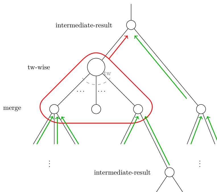
■ Figure 3 Partial sketch of the tree T of the tw-wise tree decompositions. Colored arrows represent operations of the algorithms, with red indicating that the result of the tw-wise operations is calculated via a tw-wise matrix product, and green indicating that the result of that subtree is ANDed pointwise with the result of all other subtrees.
