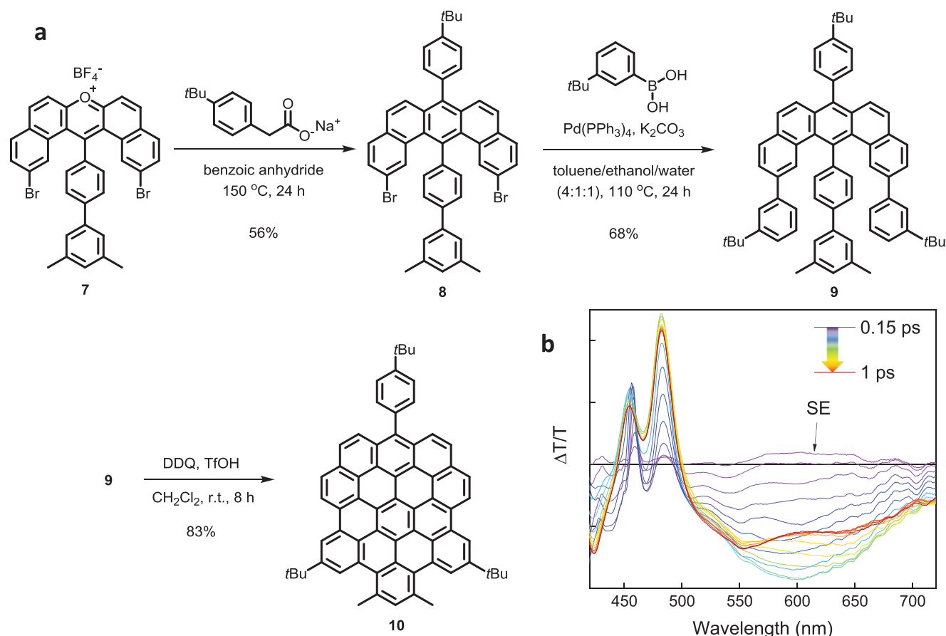
Figure 3. a) Synthetic route for HBC 10. b) TA measurements highlight the presence of a SE signal for HBC 10. However, the ultrafast decay (200 fs) hinders its application as an optical gain material. a,b) Adapted under the terms of the Creative Common CC BY license. [68] Copyright 2020, the Royal Society of Chemistry.
