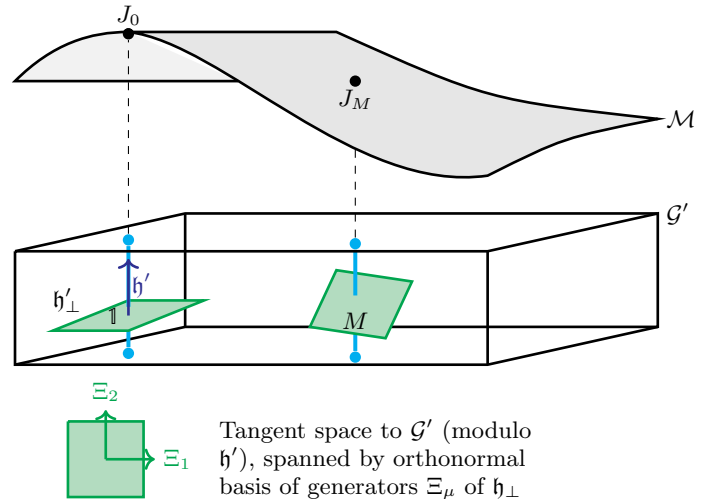
FIG. 1. Parametrization of Gaussian states. We fix a (pure) reference Gaussian state vector |J_0\rangle and then use the subgroup \mathcal{G}' \subset \mathcal{G} to generate the manifold \mathcal{M} described by complex structures J_M = MJ_0M^{-1} for M \in \mathcal{G}' .
