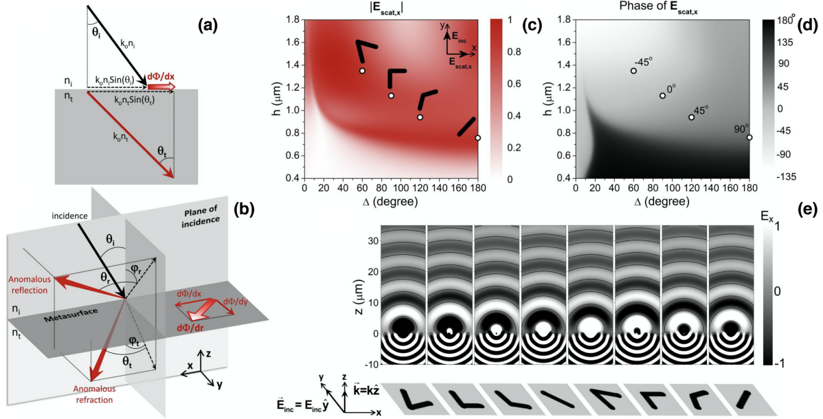
Figure 1.11: Basics of the metasurface lens theory. The interface between two media obeys the generalized Snell's law, where a constant phase gradient (a) d\Phi/dx in the 2D case and (b) d\Phi/dr in the 3D case represent an effective wavevector. Each gold antenna provides (c) nearly identical amplitude of the scattered electric field and (d) incremental phases of \pi/4 . (e) Simulation of the wavefront propagation for each unit. Figure adapted from [116].
