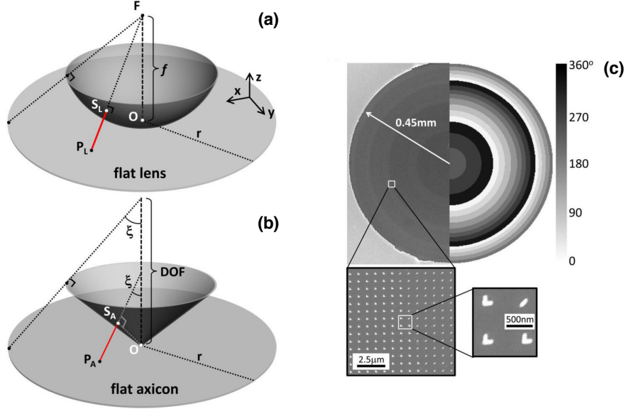
Figure 1.12: Design concept of flat lenses and axicons. (a) Hyperboloidal phase profile created by a meta-lens. (b) Conical phase profile created by a meta-axicon. (c) Typical structure of a meta-lens with discretized phase profile by eight antennas across the surface. Figure adapted from [116].
