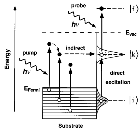
FIG. 1. Direct vs indirect excitation mechanism in pump-probe two-photon photoemission. For direct excitation the transition rates between the levels |i\rangle , |k\rangle , and |f\rangle are given by the transition-dipole moments and the electric fields at the surface. In the indirect process the first photon is absorbed in the substrate followed by scattering of a photoexcited electron into the intermediate state |k\rangle .
