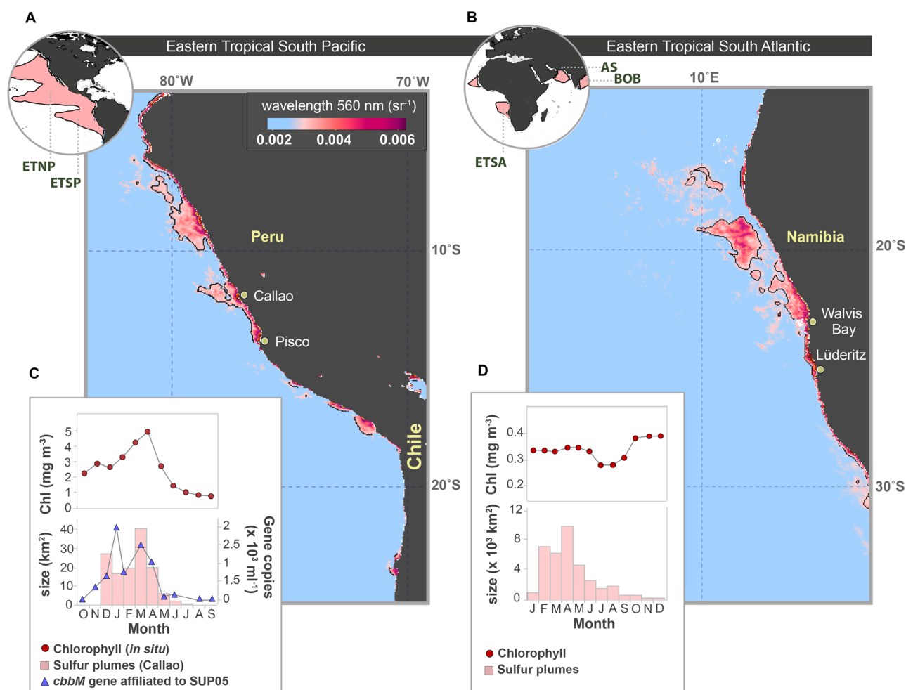
Fig. 2. Distribution and prevalence of sulfur plume activity in oxygen minimum zones. Sulfur plumes develop in eutrophic upper shelf waters (< 200 m water depth). Sulfur plumes can also be transported into the offshore OMZ (> 200 m water depth) due to lateral transport processes (e.g., mesoscale eddies). (A,B) Remote sensing images of sulfur plumes using the water-leaving reflectance wavelength of 560 nm (optimal waveband for sulfur plume detection; Ohde et al. 2007; Ohde and Dadou 2018). The images shown are seasonal composites from 21 December to 20 March 2004–2005. The images were acquired by moderate resolution imaging spectroradiometer (MODIS) downloaded from the NASA Ocean Color Database and processed using SeaDas software ( www.seadas.gsfc.nasa.gov/ ). In the world atlas globes, the contour line indicates 20 \mu\text{M} of \text{O}_2 , which represents the traditional upper boundary of the OMZ water mass. The total area of the OMZ (at a 20 \mu\text{M} \text{O}_2 cutoff) is indicated by the red shading. The oxygen data is based on world atlas data from 2013. Abbreviations indicated stand for: eastern tropical South Pacific (ETSP), eastern tropical North Pacific (ETNP), eastern tropical South Atlantic (ETSA), Arabian Sea (AS), and the Bay of Bengal (BOB). (C,D) Seasonality of chlorophyll and sulfur plume development in the ETSP and ETSA regions reproduced from Ohde 2018 and Echevin et al. 2008, and from Ohde and Dadou 2018 and Lamont et al. 2018, respectively. Panel c also includes a marker gene associated to the SUP05 clade; the ccbM gene is involved in carbon fixation via the Calvin–Benson–Bassham cycle, data is reproduced from Léniz et al. 2017. Shown are the maximum ccbM copy numbers of the three sampled depths by Léniz et al. 2017. Note that panel C is representing local remote sensing data off the coast of Callao from 11.8°S to 12.4°S; while panel D presents regional remote sensing covering the Namibian shelf from 22°S to 26°S, hence the differences in sulfur plume size between the two studies.
