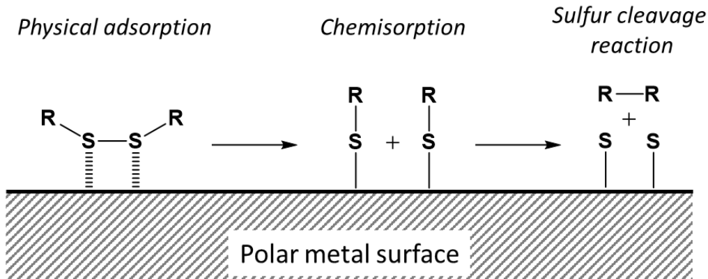
Figure 2.3.4: Sulfur carriers on a polar metal surface showing physical adsorption, chemisorption and finally sulfur cleavage reaction.
