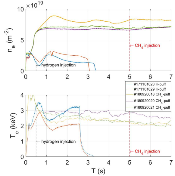
Figure 2: Upper figure: Line integrated densities for the hydrogen and methane puffing. Lower figure: Electron temperatures from channel #13 of the ECE system. The dashed line indicates the beginning of the gas injection
