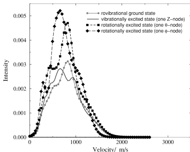
FIG. 10. Asymptotic velocity distributions for an averaged resonance lifetime \tau = 10 fs for different eigenstates of the electronic ground-state PES. The velocity distributions are averaged with respect to the rotational state of the desorbing CO-molecule.
