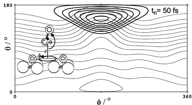
FIG. 7. \theta – \phi -snapshot of rovibrational ground-state wave packet after time evolution of 50 fs on the PES of the electronically excited state. The CO molecule has left its strongly tilted equilibrium geometry towards an upright adsorption geometry. Simultaneously, the molecule starts to rotate within a plane parallel to the surface.
