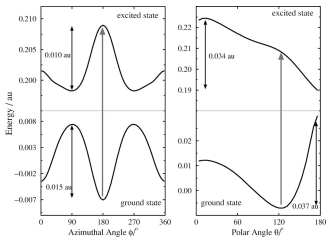
FIG. 4. 1D cuts through electronic ground- and excited-state PES. Left : \phi -corrugation at \theta=120^\circ and Z=4.5 a.u. Right : \theta -dependence at \phi=180^\circ and Z=4.5 a.u. The upward arrow indicates a vertical sudden transition.
