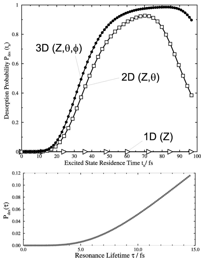
FIG. 8. Top : Asymptotic desorption probability P_{\text{des}}(t_n) ; open triangles: 1D-calculations in Z with \theta and \phi frozen at ground-state equilibrium values; open squares: 2D-calculation in Z and \theta with \phi frozen; filled circles: 3D-calculation in Z , \theta , and \phi . Bottom : Lifetime averaged desorption probability (from 3D calculations) as a function of the resonance lifetime \tau .
