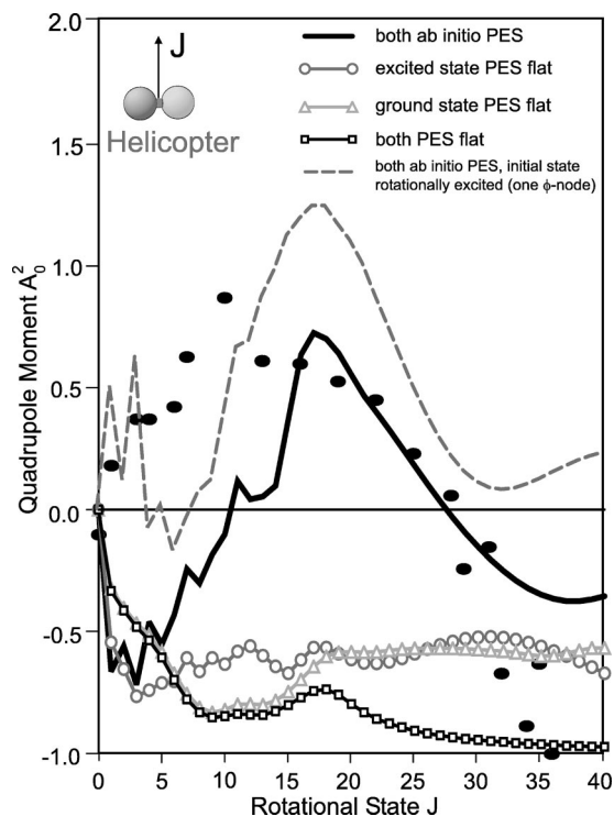
FIG. 11. Quadrupole moment for the desorption of CO from \text{Cr}_2\text{O}_3 as a function of rotational excitation, averaged with respect to the desorption velocity; the resonance-lifetime of the \text{CO}^* -intermediate has been chosen as \tau=10 fs in coincidence with a reasonable desorption probability. Filled circles: Experimental data points.
