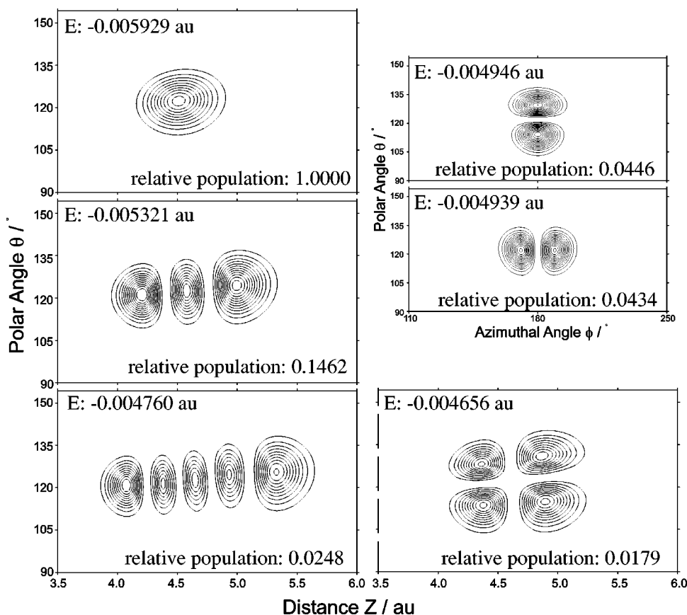
FIG. 5. Eigenstates of the three-dimensional electronic ground-state PES. Left : Excitation of molecule-surface vibration. Right : Excitation of frustrated rotation. Absolute energies E and relative populations P/P_0 at the experimental temperature of T = 100 K are given. The Z-\theta distributions are shown for the azimuthal equilibrium configuration ( \phi = 180^\circ ). The \theta-\phi distributions are shown for the equilibrium center-of-mass distance ( Z = 4.5 a.u.).
