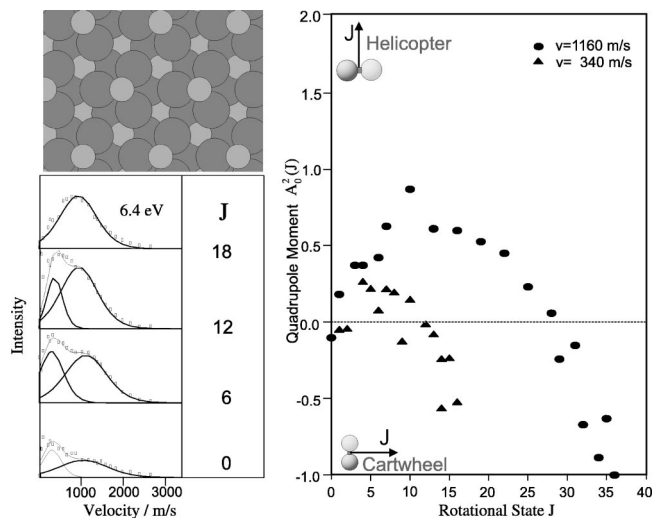
FIG. 1. Experimental results after photodesorption of CO from the \text{Cr}_2\text{O}_3(0001) -surface with 6.4 eV radiation. Left : Geometrical structure of the terminating layer (top), velocity distributions as function of the desorbate rotational state (bottom)— Right : quadrupole moment of desorbing CO as function of rotational state for a low and a high velocity.
