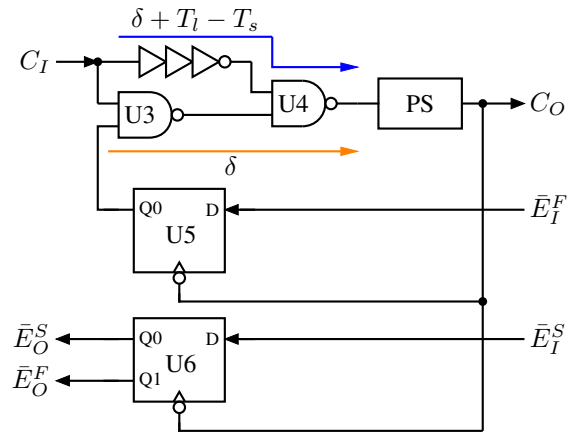
Figure 4. Delay Element Implementation (DE-I). U5 and U6 are falling edge triggered and have setup hold times of t_{set} and t_{hold} . Outputs Q0 are slow-masking (i.e., 0-masking), and output Q1 is fast-masking (i.e., 1-masking). PS is a pulse shaping module, cf. Figure 5. (Authors: FKLW)
