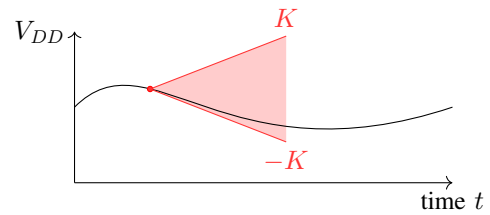
Figure 1. Assumption on droops: V_{DD} has maximum slope K and minimum slope -K . (Authors: FKLW)
