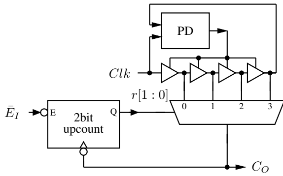
Figure 3. Phase accumulator implementation ( \varphi -DLL-I) based on tapped DLL, formed by the phase detector PD controlling a starved inverter chain, a counter, and a MUX to select the phase [14]. Note the absence of a synchronizer for the counter enable in our design variant. (Authors: FKLW)
