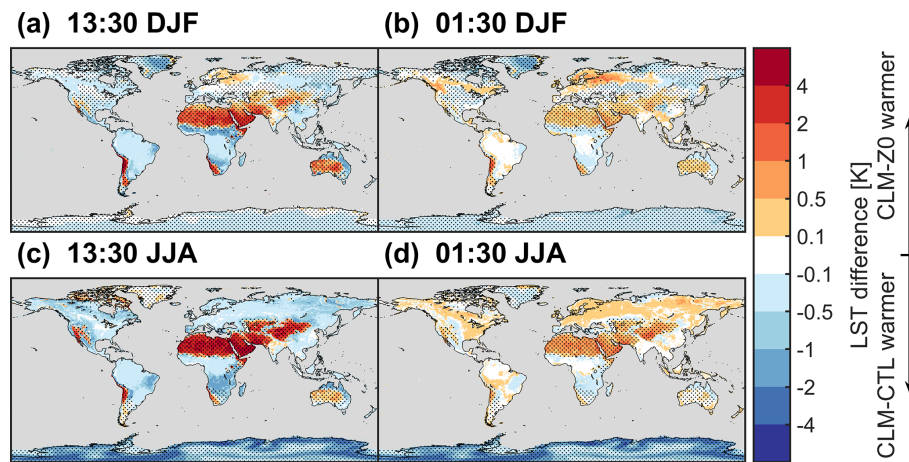
Figure 7. LST difference between CLM-Z0 and CLM-CTL. (a, c) LST difference at 13:30 local solar time and (b, d) difference at 01:30 local solar time. (a, b) Boreal winter (DJF) and (c, d) boreal summer (JJA). The stippling shows areas dominated by bare soil with a seasonal average VAI below 0.5 \text{ m}^2 \text{ m}^{-2} . Note the non-linear color scale.
