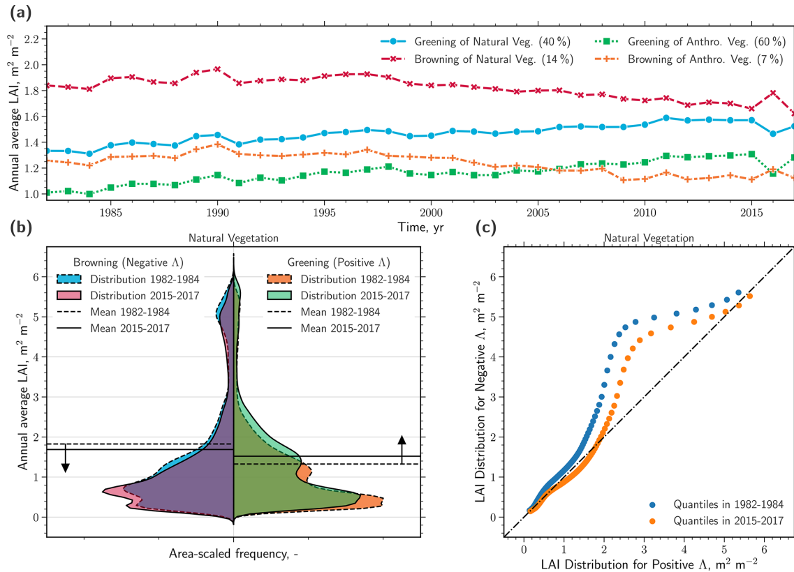
Figure 3. Observed homogenization of the global natural vegetation. (a) Time series of the area-weighted annual average LAI (GIMMS LAI 3g , 1982–2017) of natural and anthropogenic vegetation for regions of positive (greening) and negative (browning) trends. Only regions exhibiting significant trends are considered (Mann–Kendall significance test, p < 0.1 ) and are referred to as \Lambda . The percentages in parentheses in the legend represent the respective proportions with respect to the total area. (b) Violin plot comparison of probability density functions (PDFs, Gaussian kernel density estimation; all PDFs scaled to contain the same area) of LAI distributions of natural vegetation for negative (left) and positive (right) \Lambda , and in time, 1982–1984 (dashed) versus 2015–2017 (solid). The horizontal lines represent the mean values for the respective period. (c) Q–Q (quantile–quantile) plot comparing the distributions of LAI for negative ( x axis) and positive ( y axis) \Lambda and their change over time, 1982–1984 (blue dots) versus 2015–2017 (orange dots).
