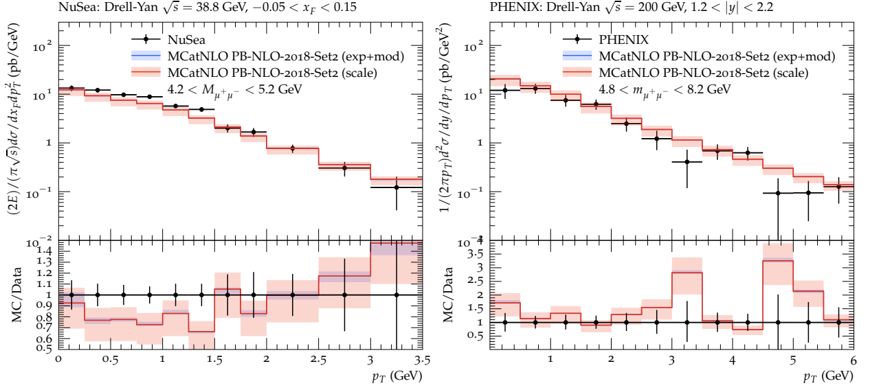
Figure 4.18: Transverse momentum spectra in low-mass Drell-Yan lepton pair production [302] from the parton branching (PB) method, compared with (left) NuSea measurements [303] and (right) PHENIX measurements [304].
