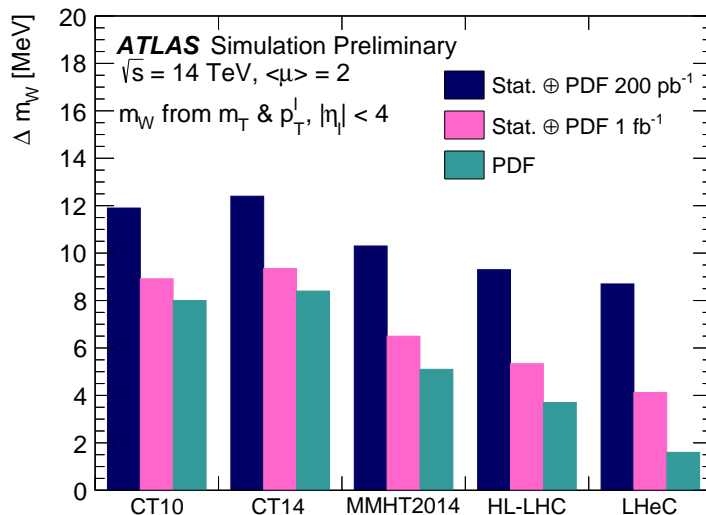
Figure 9.2: Measurement uncertainty of m_W at the HL-LHC with 200 \text{ pb}^{-1} (dark blue) and 1 \text{ fb}^{-1} (pink) of collected low pile-up data for different present and future PDF sets from Ref. [723]. The green area indicates the PDF uncertainty from those sets alone. The projections are obtained from a combined fit to the simulated p_T^\ell and m_T distributions in the acceptance |\eta| < 4 .
