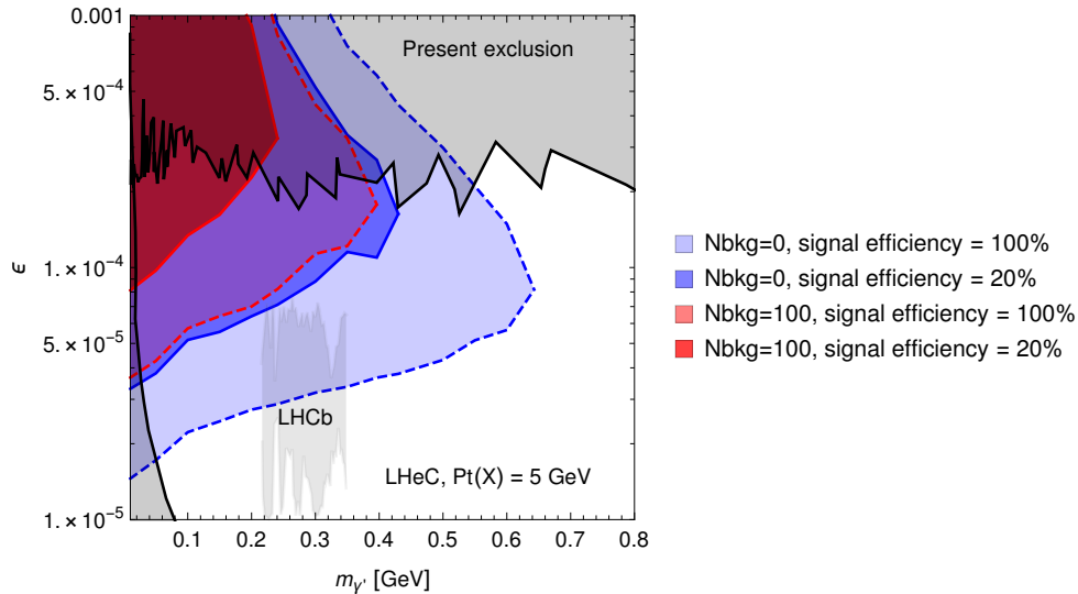
Figure 8.11: Projected sensitivity of dark photon searches at the LHeC via displaced dark photon decays from Ref. [669]. The sensitivity contour lines are at the 90 % confidence level after a transverse momentum cut on the final state hadrons of 5 GeV. The blue and red areas denote the assumption of zero and 100 background events, respectively, the solid and dashed lines correspond to a reconstruction efficiency of 100 % and 20 %, respectively. See Ref. [669] for details.
