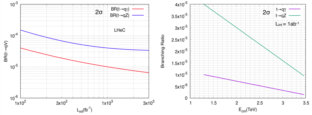
Figure 5.17: Expected sensitivities on FCNC t \rightarrow qV branching ratios (left), as a function of the integrated luminosity [487, 488]. Right: the expected upper limits on FCNC t \rightarrow qV branching ratios are shown dependent on the centre-of-mass-energy.
