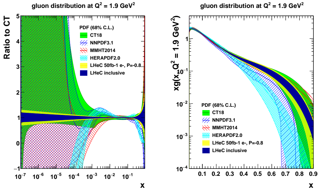
Figure 3.15: Gluon distribution at Q^2 = 1.9 \text{ GeV}^2 as a function of x . Left: the distribution is displayed as the ratio to the CT18 PDF set and highlights the low x region. Right: the distribution is shown on a linear x scale and highlights the high x region. The yellow band corresponds to the “LHeC 1st run” PDFs (D2), while the dark blue shows the “LHeC inclusive” PDFs (D4+D5+D6+D9), as described in the text. Both LHeC PDFs shown are scaled to the central value of CT18.
