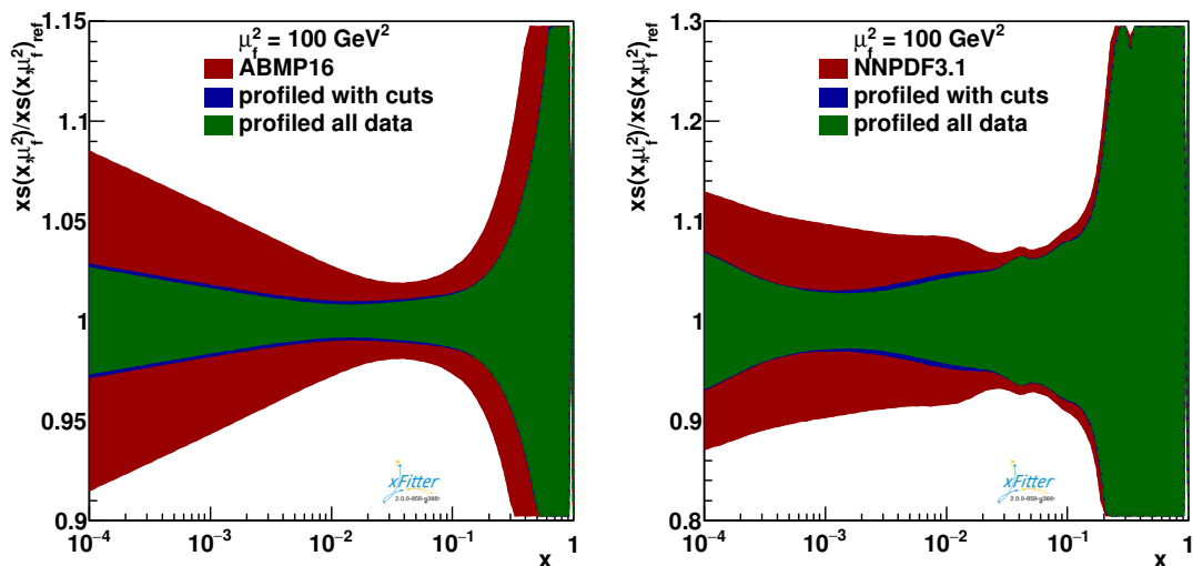
Figure 3.13: Constraints on the strange quark PDF x_s using simulated data for charged-current production of charm quarks at the LHeC, from a profiling study [80] using the ABMP16 (left) and the NNPDF3.1 (right) PDF sets. The red band displays the nominal PDF uncertainties, and the green and blue bands the improved uncertainties due to the LHeC strange quark data.
