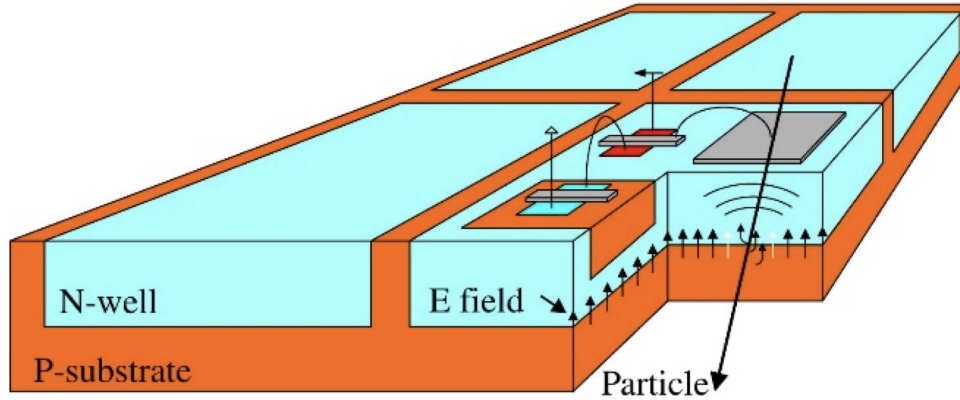
Figure 12.10: Typical sensor cross-section of a DMAPS detector in a HV-CMOS process [900].
