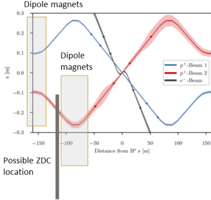
Figure 12.16: Possible location for a ZDC for the linac–ring IR design of LHeC as shown in Fig. 10.28. The solid rectangle represents the potential location and magnets overlaid.
