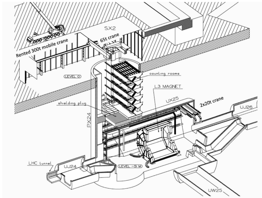
Figure 12.18: View of the cavern infrastructure at Point 2 [913]. The support structure of the magnet of the L3 experiment (at the centre) will house and support the LHeC detector.
