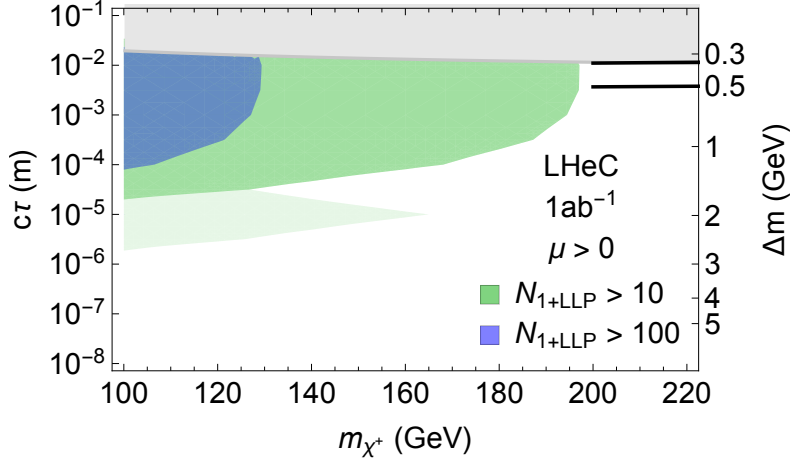
Figure 8.6: Exclusion limits on Higgsino masses as a function of their lifetime from Ref. [642]. Coloured regions denote where 10 or 100 events with at least one LLP decay are observed. Light shading indicates the uncertainty in the predicted number of events due to different hadronisation and LLP reconstruction assumptions. The black curves are the optimistic and pessimistic projected bounds from HL-LHC disappearing track searches.
