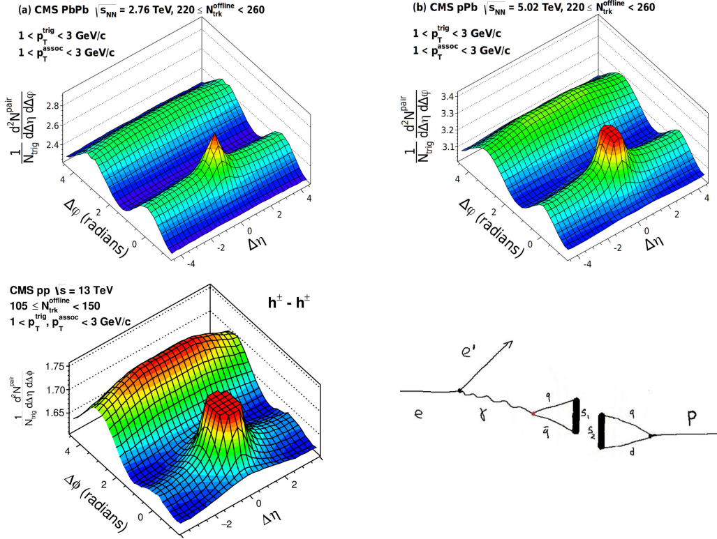
Figure 6.18: Left and top right: Collective effects seen in high-multiplicity two-particle azimuthal correlation, as observed by CMS in PbPb, pPb [562], and pp [563] collisions. Bottom right: Schematic illustration for the production of ridge -like effects in ep or eA scattering at the LHeC [564].
