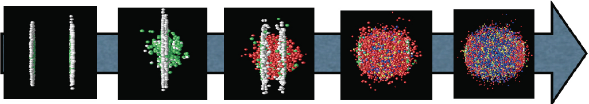
Figure 9.15: Sketch of a heavy ion collision with time running left to right, going from the approach of two ultrarelativistic Lorentz-contracted nuclei, the collision and parton creation in the central rapidity region, the beginning of expansion and formation of the QGP, the expansion of the QGP until hadronisation, and, finally, the expansion of the hadronic gas.
