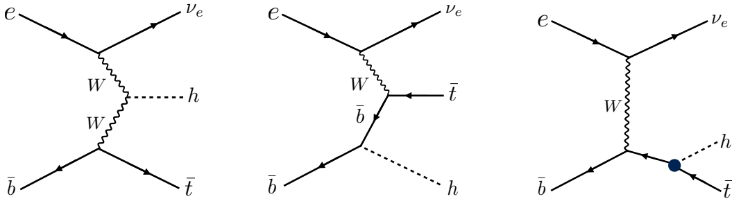
Figure 7.14: Leading order Feynman diagrams contributing to the process pe^- \rightarrow \bar{t}h\nu_e in high energy e^-p collisions. The full circle in the right diagram shows the top-quark–Higgs coupling of interest in this section.
