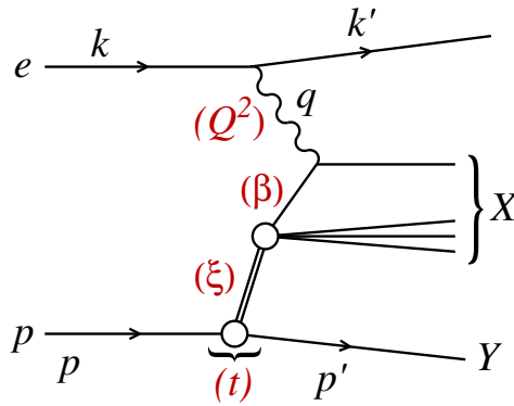
Figure 4.21: A diagram of a diffractive NC event in DIS together with the corresponding variables, in the one-photon exchange approximation. The incoming proton scatters elastically or is dissociated into a low mass excitation Y . The system of particles denoted by X is then separated from the proton (or its excitation Y ) by a large rapidity gap. Double line indicates a diffractive exchange in the t channel.
