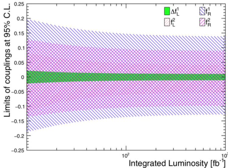
Figure 5.13: Expected sensitivities on the SM and anomalous Wtb couplings, as a function of the integrated luminosity [473].
