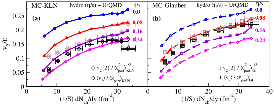
Figure 9.17: Comparison of the universal v_2(\eta/s)/\varepsilon vs. (1/S)(dN_{\text{ch}}/dy) curves with experimental data for \langle v_2 \rangle [790], v_2\{2\} [791], and dN_{\text{ch}}/dy [792] from the STAR Collaboration. The experimental data used in (a) and (b) are identical, but the normalisation factors \langle \varepsilon_{\text{part}} \rangle and S used on the vertical and horizontal axes, as well as the factor \langle \varepsilon_{\text{part}}^2 \rangle^{1/2} used to normalize the v_2\{2\} data, are taken from the MC-KLN model in (a) and from the MC-Glauber model in (b). Theoretical curves are from simulations with MC-KLN initial conditions in (a) and with MC-Glauber initial conditions in (b). Taken from [786].
