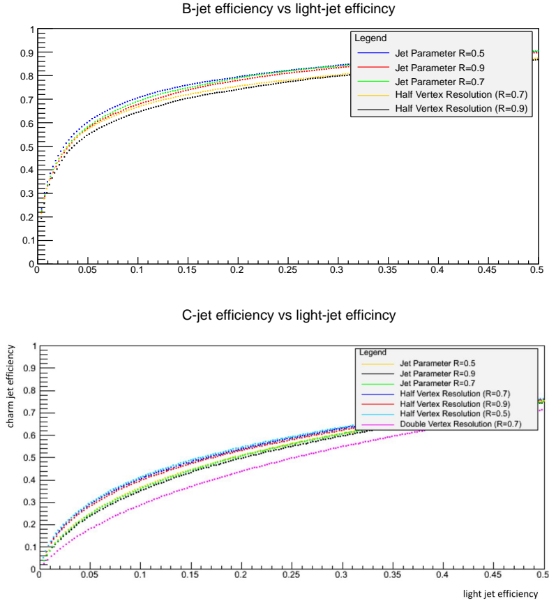
Figure 7.7: Expected average efficiency to tag a b -jet (upper plot) and charm-jet (lower plot) versus the light-jet efficiency (x-axis) based on Tevatron-style jet tagging [604]. Events are selected at DELPHES detector level using a CC multi-jet sample and for an integrated luminosity of 100 \text{ fb}^{-1} . The coloured lines correspond to the choice of the anti-kt distance parameter R and different assumptions in the impact parameter resolution of 10 (5) \mu\text{m} (nominal, no text added in legend), 5 (2.5) \mu\text{m} (Half Vertex Resolution), 20 (10) \mu\text{m} (Double Vertex Resolution) for tracks with 0.5 < p_T < 5 ( > 5 ) GeV within |\eta| < 3.5 .
