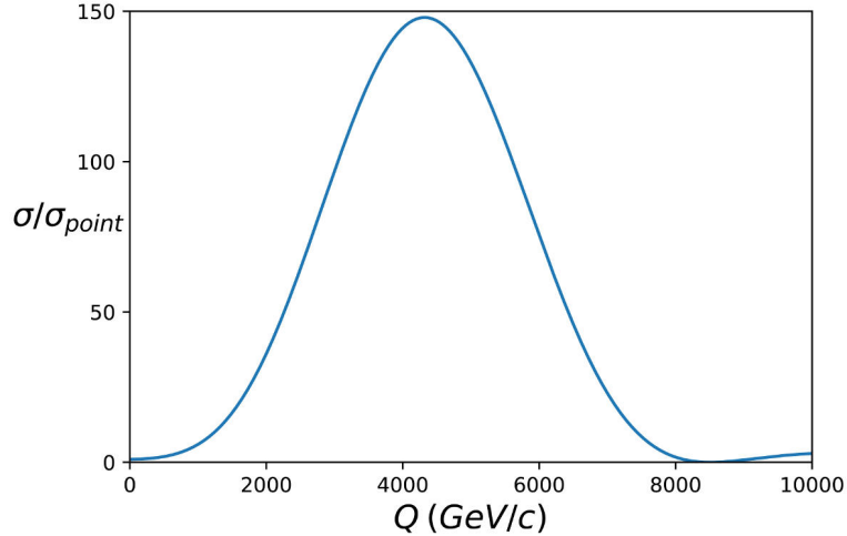
Figure 8.16: Form factor effect in the e-p interaction produced by substructure according to Model II of Hofstadter [707] with the model parameters given in the text.
