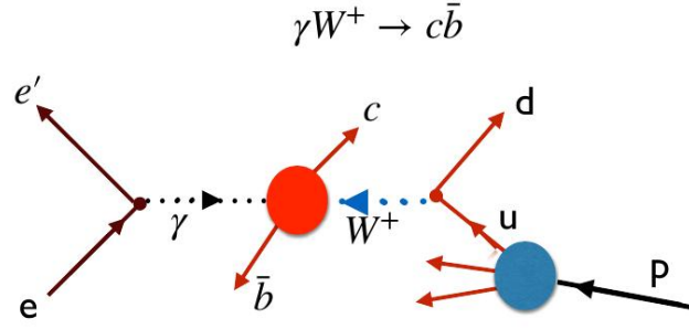
Figure 8.13: The radiation amplitude zero of the Standard Model in \gamma W^+ \rightarrow c\bar{b} and \gamma u \rightarrow W^+ d . A prediction for the angular distribution \frac{d\sigma}{d\cos(\theta_{CM})}(\gamma u \rightarrow W^+ d) is provided in Ref. [676].
