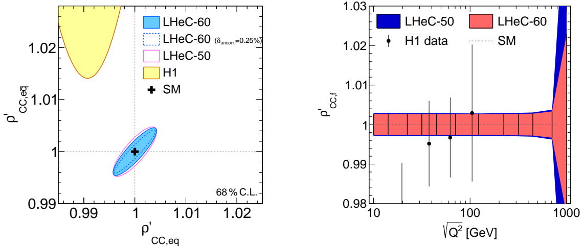
Figure 5.9: Left: anomalous modifications of the charged current form factors \rho'_{CC,eq} and \rho'_{CC,e\bar{q}} for different LHeC scenarios in comparison with the H1 measurement [423]. Right: scale dependent measurement of the anomalous modification of the charged current form factor \rho'_{CC}(Q^2) , assuming \rho'_{CC,eq} = \rho'_{CC,e\bar{q}} = \rho'_{CC} .
