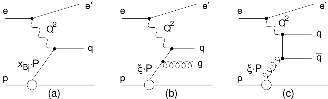
Figure 4.1: Leading order diagrams for inclusive DIS (a) and jet production (b,c) in the Breit frame (taken from Ref. [139]).
