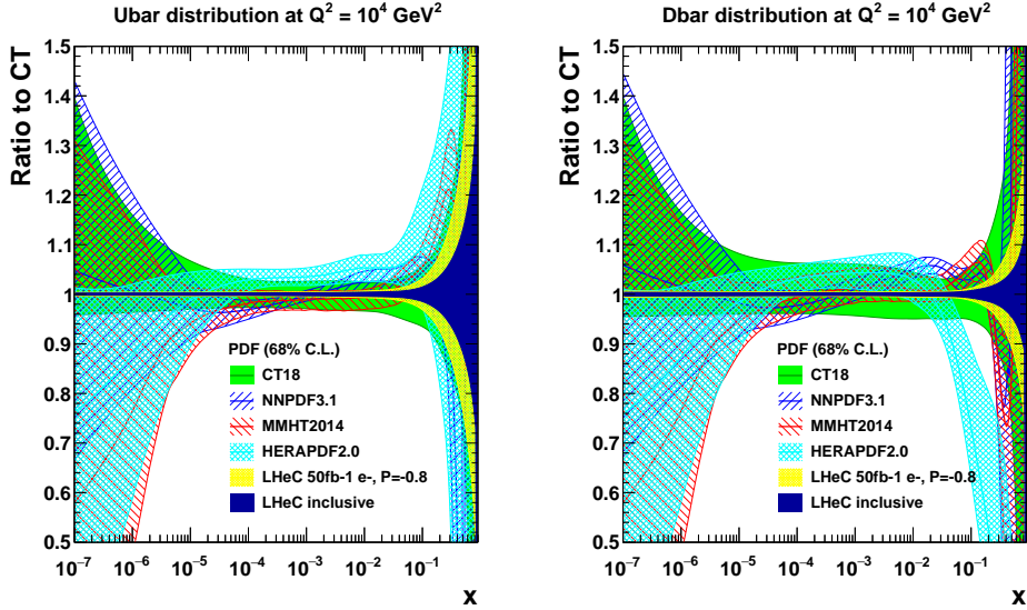
Figure 3.11: Sea quark distributions at Q^2 = 10^4 \text{ GeV}^2 as a function of x , displayed as the ratio to the CT18 PDF set. The yellow band corresponds to the “LHeC 1st run” PDFs (D2), while the dark blue shows the final “LHeC inclusive” PDFs (D4+D5+D6+D9), as described in the text. Both LHeC PDFs shown are scaled to the central value of CT18.
