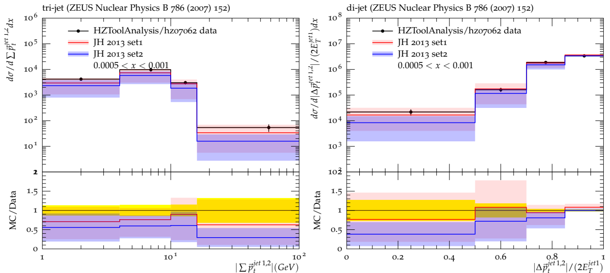
Figure 4.17: Momentum correlations in DIS multi-jet final states at low x computed from the CCFM Monte Carlo [288] with TMD parton densities JH2013 [296], compared with the measurements [295]: (left) tri-jets; (right) di-jets.
