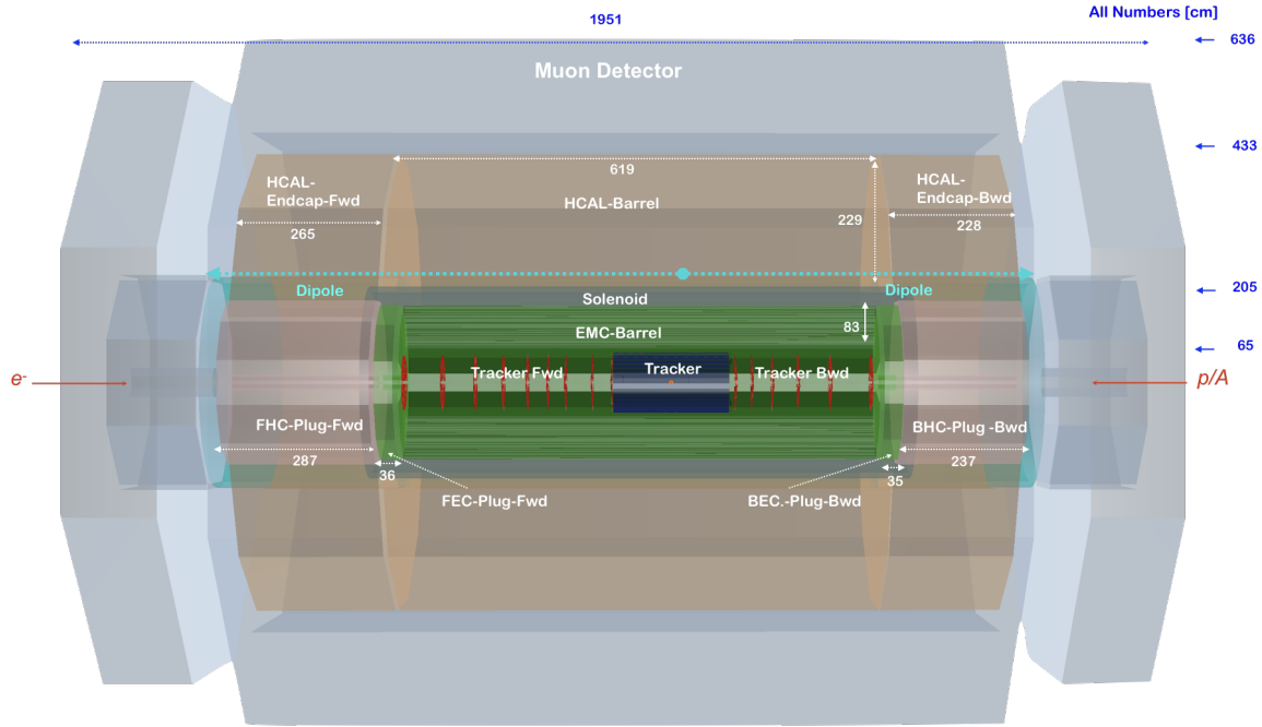
Figure 12.21: Side view of a low energy FCCeh ( E_p = 20 TeV) concept detector, designed using the DD4hep framework [897], showing the essential features. The solenoid is again placed between the ECAL-Barrel and Hadronic-Barrel calorimeters and is housed in a cryostat in common with the beam steering dipoles extending over the full length of the barrel and plug hadronic calorimeters. The sizes have been chosen such that the solenoid/dipoles and ECAL-Barrel systems as well as the whole tracker are also suitable to operate after an upgrade of the beam energy to E_p = 50 TeV.
