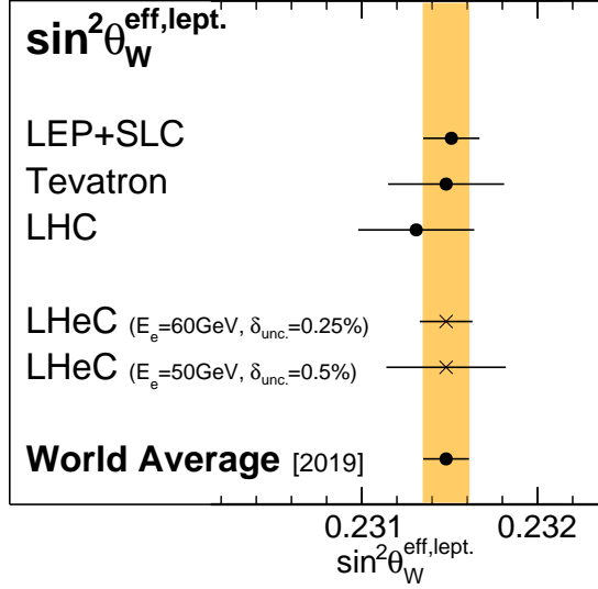
Figure 5.7: Comparison of the determination of \sin^2 \theta_W^{\text{eff},\ell}(M_Z^2) from LHeC inclusive DIS data with recent averaged values. Results from LEP+SLC [444], Tevatron [446], LHC [447–450] and the world average value [450] are all obtained from a combination of various separate measurements (not shown individually) (see also Ref. [451] for additional discussions). For LHeC, the experimental and PDF uncertainties are displayed.
