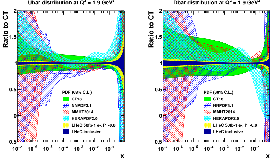
Figure 3.10: Sea quark distributions at Q^2 = 1.9 \text{ GeV}^2 as a function of x , displayed as the ratio to the CT18 PDF set. The yellow band corresponds to the “LHeC 1st run” PDFs (D2), while the dark blue shows the final “LHeC inclusive” PDFs (D4+D5+D6+D9), as described in the text. Both LHeC PDFs shown are scaled to the central value of CT18.
