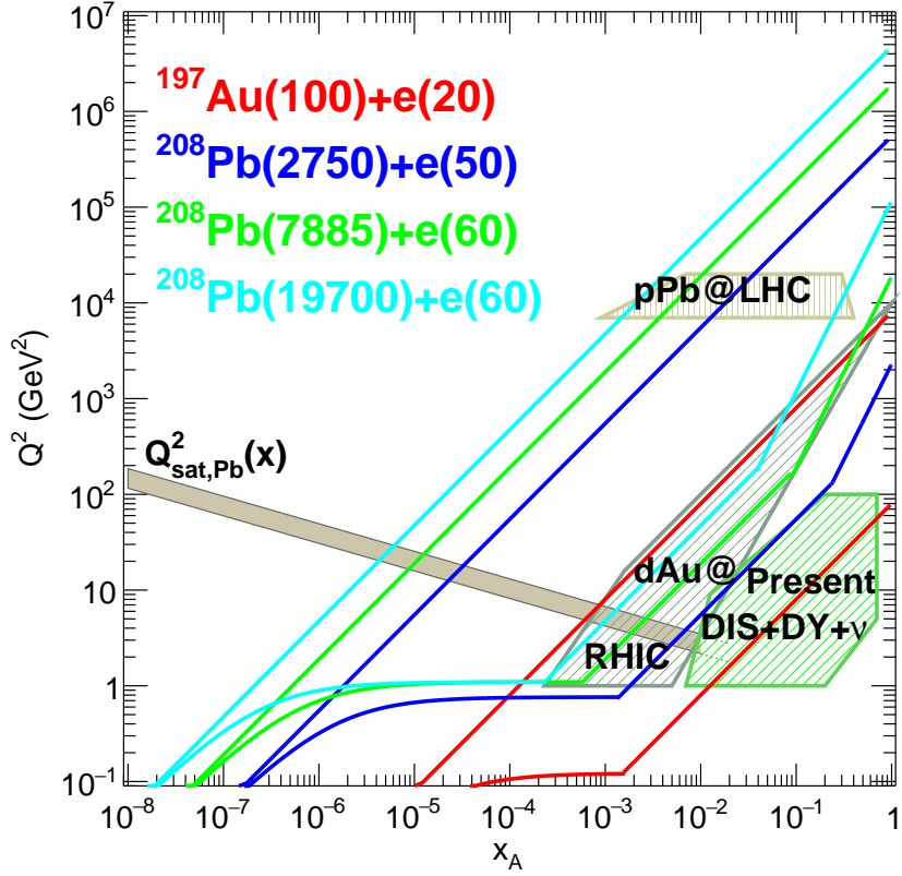
Figure 6.1: Kinematic regions in the x - Q^2 plane explored by different data sets (charged lepton and neutrino DIS, DY, dAu at RHIC and pPb at the LHC) used in present nPDF analyses [503], compared to the ones achievable at the EIC (red), the LHeC (ERL against the HL-LHC beams, dark blue) and two FCC-eh versions (with Pb beams corresponding to proton energies E_p = 20 TeV - green and E_p = 50 TeV - light blue). Acceptance of the detector for the electrons is taken to be 1^\circ < \theta < 179^\circ , and 0.01(0.001) < y < 1 for the EIC (all other colliders). The saturation scale Q_{sat} shown here for indicative purposes only, see also [504], has been drawn for a Pb nucleus considering an uncertainty \sim 2 and a behaviour with energy following the model in [505]. Note that it only indicates a region where saturation effects are expected to be important but there is no sharp transition between the linear and non-linear regimes.
