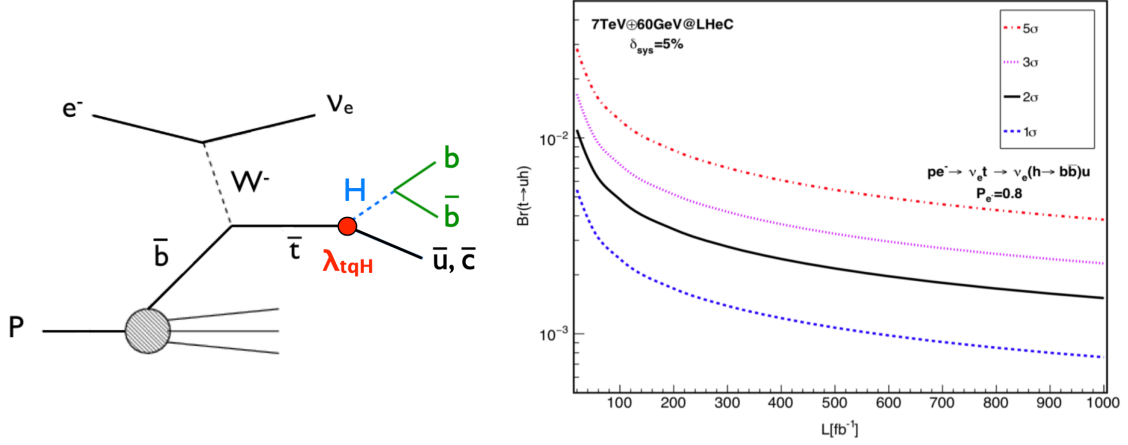
Figure 5.18: Example Feynman graph for associated single top quark and Higgs boson production via FCNC tqH couplings (left). Expected sensitivities on FCNC t \rightarrow uH branching ratios are given as a function of the integrated luminosity [492] (right).
