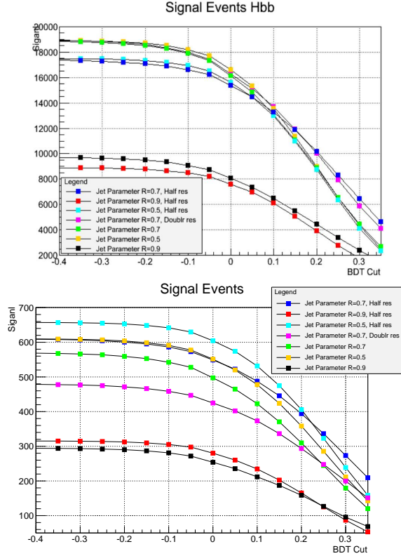
Figure 7.8: Expected H \rightarrow b\bar{b} (left) and H \rightarrow c\bar{c} (right) signal events as a function of the BDT score. Events are selected at DELPHES detector level for an integrated luminosity of 1 \text{ ab}^{-1} and -80\% electron polarisation. The symbols correspond to the choice of the anti-kt distance parameter R and different assumptions in the impact parameter resolution of 10 (5) \mu\text{m} (nominal, no further text in legend added), 20 (10) \mu\text{m} (Doubl res), 5 (2.5) \mu\text{m} (Half res) for tracks with 0.5 < p_T < 5 (> 5) GeV within |\eta| < 3.5 .
