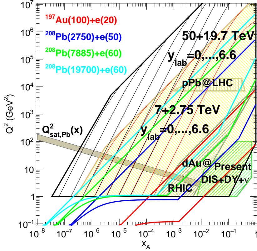
Figure 9.18: Kinematic regions in the x - Q^2 plane explored by data sets (charged lepton and neutrino DIS, DY, dAu at RHIC and pPb at the LHC) used in present nPDF analyses [503], compared to the ones achievable at the EIC (red), the LHeC (ERL against the HL-LHC beams, dark blue) and two FCC-eh versions (with Pb beams corresponding to proton energies of 20 TeV - green and 50 TeV - light blue). Acceptance is taken to be 1^\circ < \theta < 179^\circ , and 0.01(0.001) < y < 1 for the EIC (all other colliders). The areas delimited by thick brown and black lines show the regions accessible in pPb collisions at the LHC and the FCC-hh (50 TeV) respectively, while the thin lines represent constant rapidities from 0 (right) to 6.6 (left) for each case. The saturation scale Q_{sat} shown here for indicative purposes only, see also [504], has been drawn for a Pb nucleus considering an uncertainty \sim 2 and a behaviour with energy following the model in [505]. Note that it only indicates a region where saturation effects are expected to be important but there is no sharp transition between the linear and non-linear regimes.
