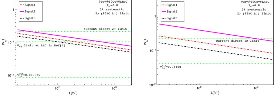
Figure 5.14: Expected sensitivities on |V_{td}| (left) and |V_{ts}| (right), as a function of the integrated luminosity [478].
