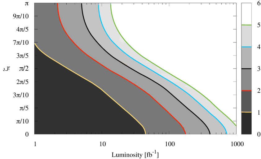
Figure 7.17: Exclusion contours for \zeta_t as a function of integrated luminosity for \sqrt{s} = 1.3 \text{ TeV} (from Ref. [484]). The shaded areas under a contour-line are excluded. The blue and black lines represent the 4\sigma and 3\sigma regions. Results are obtained based on fiducial cross-sections (see text).
