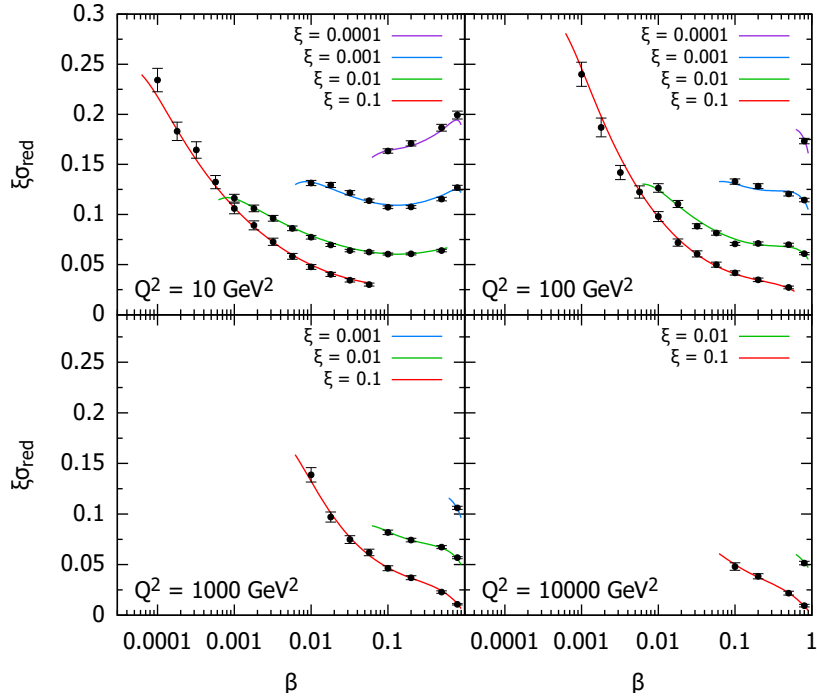
Figure 4.24: Selected subset of the simulated data for the diffractive reduced cross section as a function of \beta in bins of \xi and Q^2 for ep collisions at the LHeC. Based on the extrapolation of the ZEUS-SJ fit to HERA data. The curves for \xi = 0.01, 0.001, 0.0001 are shifted up by 0.04, 0.08, 0.12, respectively. Integrated luminosity is taken to be 2 \text{ fb}^{-1} . Figure taken from [346].
