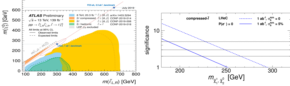
Figure 8.5: Left: Benchmark assumption on slepton masses and 2019 reach of current ATLAS searches for sleptons (figure adapted from Ref. [644]). Right: Significances as varying the masses of \tilde{\chi}_1^\pm and \tilde{\chi}_2^0 for the compressed-slepton scenario at the LHeC with unpolarised beams and 1 \text{ ab}^{-1} luminosity. For dashed (solid) curve, a systematic uncertainty of 0% (5%) on the background is considered. The figure is from Ref. [643].
