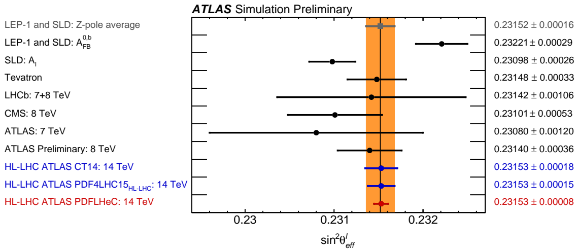
Figure 9.1: Comparison of measurements or combinations of \sin^2\theta_{\text{eff}}^{\ell} with the world average value (orange band) and the projected uncertainties of measurements at the HL-LHC from Ref. [717]. For the HL-LHC the central values are set to the world average value and uncertainties are displayed for different assumptions of the available PDF sets, similar to Tab. 9.1.
