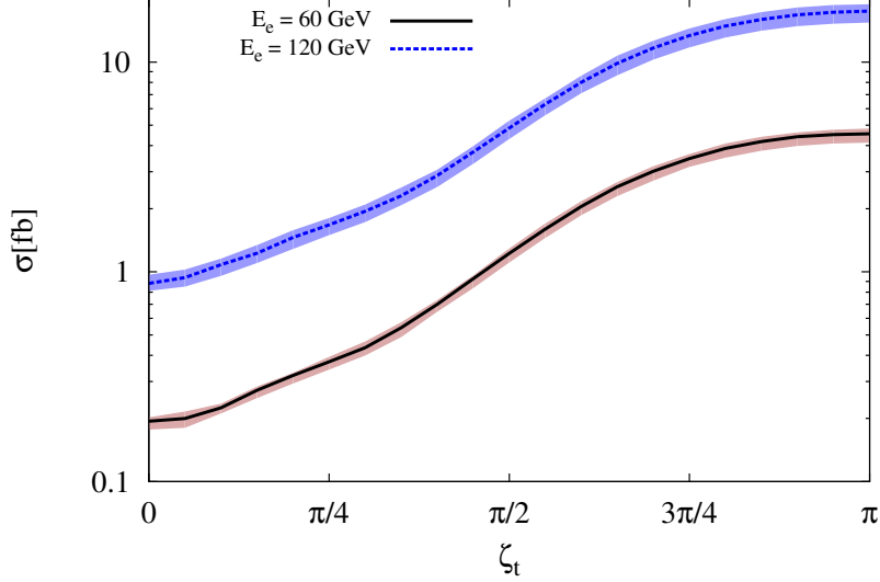
Figure 7.16: Total cross section of the Higgs boson produced in association with a single top as a function of \zeta_t , including scale uncertainties (taken from Ref. [484]). The black solid and blue dotted lines correspond to E_e = 60 and 120 GeV, respectively. These are obtained for fixed E_p = 7 TeV and scales \mu_F = \mu_R = (m_t + m_h)/4 .
