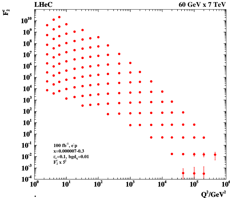
Figure 3.6: Simulation of the measurement of the charm quark distribution expressed as F_2^c = e_c^2 x(c + \bar{c}) in neutral current e^-p scattering. The vertical error bars indicate the full systematic and statistical uncertainties added in quadrature, but are mostly smaller than the marker size. The minimum x (left top bin) is at 7 \cdot 10^{-6} , and the data extend to x = 0.3 (right bottom bin). The simulation uses a massless scheme and is only indicative near threshold albeit the uncertainties entering the QCD PDF analysis are estimated consistently.
