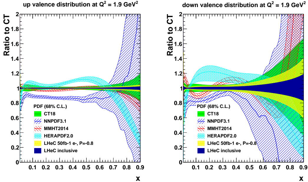
Figure 3.8: Valence quark distributions at Q^2 = 1.9 \text{ GeV}^2 as a function of x , displayed as a ratio to the CT18 [67] PDF set. The yellow band corresponds to the “LHeC 1st run” PDFs (D2), while the dark blue shows the final “LHeC inclusive” PDFs based on the data sets (D4+D5+D6+D9), as described in Sect. 3.3.1. For the purposes of illustrating the improvement to the uncertainties more clearly, the central values of the LHeC PDFs have been scaled to the CT18 PDF, which itself is displayed by the green band.
