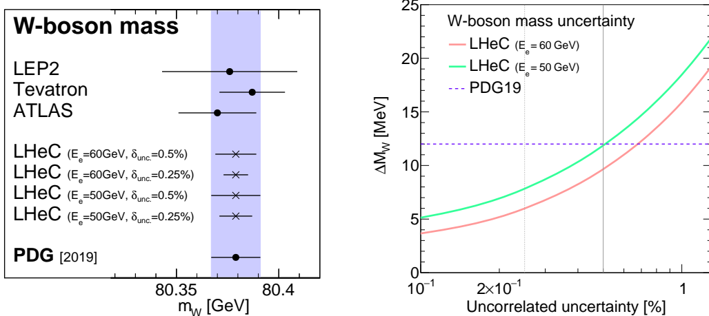
Figure 5.2: Left: Measurements of the W -boson mass assuming fixed values for the top-quark and Z -boson masses at the LHeC for different scenarios in comparison with today’s measurements [437–439] and the world average value (PDG19) [183]. For LHeC, prospects for E_e = 60 GeV and 50 GeV are displayed, as well as results for the two scenarios with 0.5 % or 0.25 % uncorrelated uncertainty (see text). Right: Comparison of the precision for M_W for different assumptions of the uncorrelated uncertainty of the pseudodata. The uncertainty of the world average value is displayed as horizontal line. The nominal (and alternative) size of the uncorrelated uncertainty of the inclusive NC/CC DIS pseudodata is indicated by the vertical line (see text).
