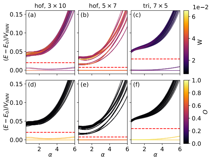
FIG. 13. Signatures of WC and FCI on the low-lying energy spectrum for models with Chern number C = 2 with the filling factor \nu = \frac{1}{5} for different plaquettes: Hofstadter model (hof) 3 \times 10 (first column) and 5 \times 7 (second column), and triangular lattice (tri) 7 \times 5 (third column). In the upper row, we plot the Cartesian crystallization strength W , and the lower row displays the overlap O with model FQH states. The overlaps in the momentum subspaces not corresponding to a model FQHE ground state are set to 0 by definition.
