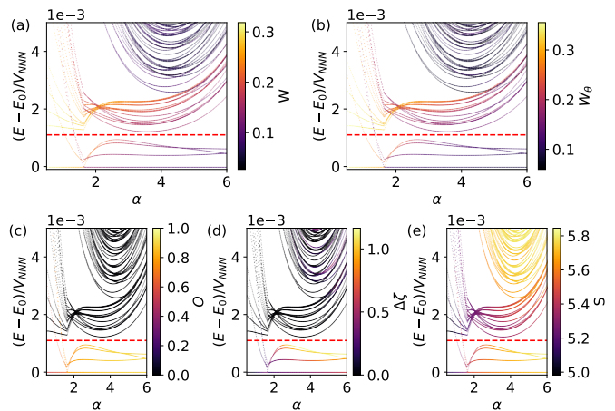
FIG. 4. The energy spectrum of a 5 \times 7 kagome system as a function of \alpha , normalized by the next-nearest-neighbor interaction V_{NNN} . The color denotes Wigner crystallization indicators in the upper row: (a) Cartesian crystallization strength, (b) polar crystallization strength, and FCI indicators in the lower row: (c) overlap with model FQH states, (d) the gap in the entanglement spectrum, (e) entanglement entropy. In (c), the overlaps in the momentum subspaces not corresponding to a model FQHE ground state are set to 0 by definition.
