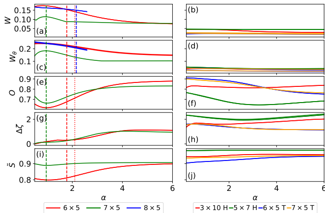
FIG. 7. The FCI and WC characteristics as a function of \alpha for different models and plaquettes at filling \nu = 1/5 for the one chosen state. The left column corresponds to the kagome lattice with the flat band with Chern number C = 1 (plots: (a), (c), (e), (g), (i)), the right column corresponds to the triangular lattice model (T) and Hofstadter model (H) with the flat band with Chern number C = 2 (plots: (b), (d), (f), (h), (j)). The different plaquettes sizes are denoted by different colors. In the first row the Cartesian crystallization strength W is shown (plots (a) and (b)), in the next row shows polar crystallization strength W_\theta (plots (c) and (d)). In the last three rows the FCI characteristics are presented: the overlap with model FQHE state (plots (e) and (f)), the entanglement gap (plots (g) and (h)), and the renormalized entanglement entropy \bar{S} = (S - S_{\min}) / (S_{\max} - S_{\min}) (plots (i) and (j)). The dashed vertical lines denote the \alpha values for which the gap above the five quasi-degenerate FCI states closes. The dotted vertical line corresponds to the location of the characteristic crossing of all five quasi-degenerate states. The results for the 8 \times 5 plaquette are obtained only for some characteristics and only in a limited range of \alpha , because of the numerical complexity of the considered system and problems with numerical convergence of diagonalization problem, especially in the limit of high \alpha values.
