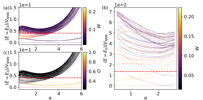
FIG. 12. The Cartesian strength of Wigner crystallization W ((a) and (b)), and overlap O with the model FQHE state (c) on the energy spectrum of the 7 \times 5 ((a) and (c)) and 8 \times 5 (b) kagome lattice at filling \nu = 1/5 . The overlaps in the momentum subspaces not corresponding to a model FQHE ground state are set to 0 by definition.
