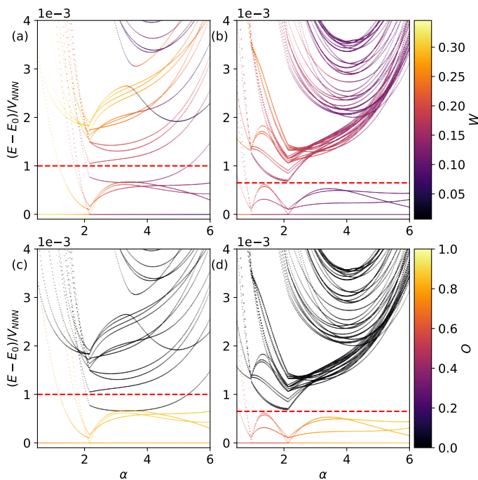
FIG. 11. The Cartesian strength of Wigner crystallization W (upper row), and overlap O with the model FQHE states (lower row) on the energy spectrum of the 4 \times 7 (left column) and 6 \times 7 (right column) kagome lattice at filling \nu = 1/7 . The overlaps in the momentum subspaces not corresponding to a model FQHE ground state are set to 0 by definition.
