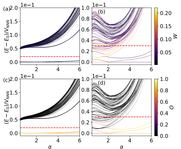
FIG. 6. The energy spectrum of 6 \times 5 C = 1 and C = 2 plaquettes as a function of \alpha , normalized by the next-nearest-neighbour interaction V_{NNN} at filling \nu = 1/5 . The left column corresponds to the triangular lattice system with the flat band with Chern number C = 2 (plots (a) and (c)), the right column corresponds to the kagome system with the flat band with Chern number C = 1 (plots (b) and (d)). The color denotes Cartesian Wigner crystallization strength in the upper row (plots (a) and (b)), and overlap with the model FQHE state in the lower row (plots (c) and (d)). The overlaps in the momentum subspaces not corresponding to a model FQHE ground state are set to 0 by definition.
