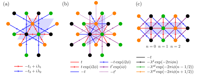
FIG. 1. The lattice models used in our work: (a) kagome lattice (b) triangular lattice (c) generalized Hofstadter model on square lattice. Only the hoppings starting and/or ending within a given unit cell (purple parallelograms) are shown.
