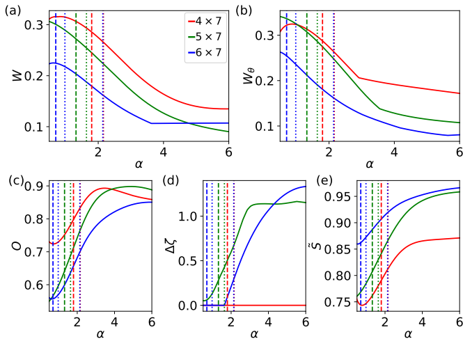
FIG. 5. The FCI and WC characteristics as a function of \alpha for three kagome systems with C = 1 at filling \nu = 1/7 (a) Cartesian crystallization strength, (b) polar crystallization strength, (c) overlap with model states, (d) entanglement gap, (e) renormalized entanglement entropy \tilde{S} = (S - S_{\min}) / (S_{\max} - S_{\min}) . The dashed vertical lines denote the \alpha values for which the gap above the seven quasi-degenerate FCI states closes. The dotted vertical lines correspond to the location of the characteristic crossing of all seven quasi-degenerate states (there are two such crossings for the 6 \times 7 system, see Fig. 11).
