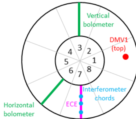
Figure 12. Schematic view of JET from the top, indicating octant numbers and the position of DMV1 and of interferometry, bolometry and ECE systems.
