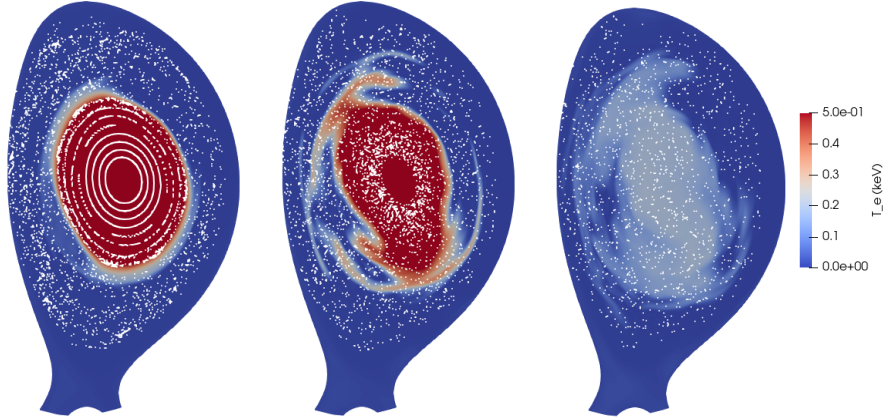
Figure 7. Poloidal cross-section of the electron temperature, with a Poincaré cross-section overlaid, in the injection plane at t = 4.62 (left), 4.80 (middle) and 5.09 ms (right) for Case C (see Table 1). The color scale is saturated at 0.5 keV so as to highlight the dynamics in the cold regions.
