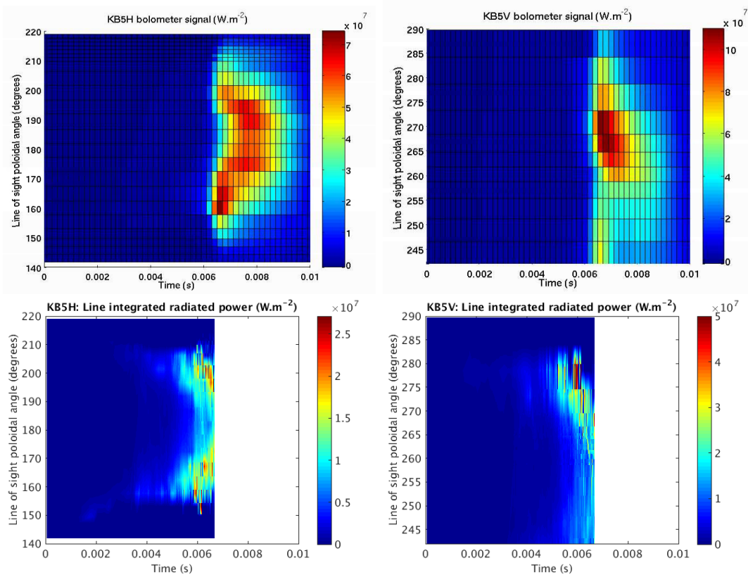
Figure 13. Experimental (top row) and synthetic (bottom row) bolometry measurements for the horizontal (KB5H, left column) and vertical (KB5V, right column) bolometers. Please note the different color scales.
