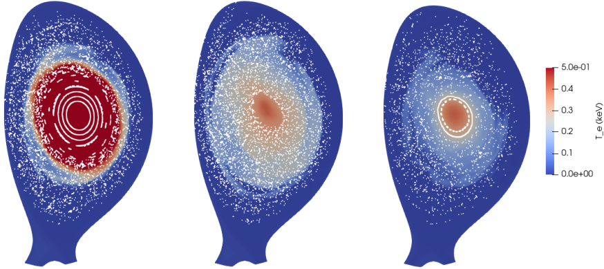
Figure 5. Poloidal cross-section of the electron temperature, with a Poincaré cross-section overlaid, in the injection plane at t = 4.92 (left), 5.95 (middle) and 6.39 ms (right) for Case A (see Table 1). The color scale is saturated at 0.5 keV so as to highlight the dynamics in the cold regions.
