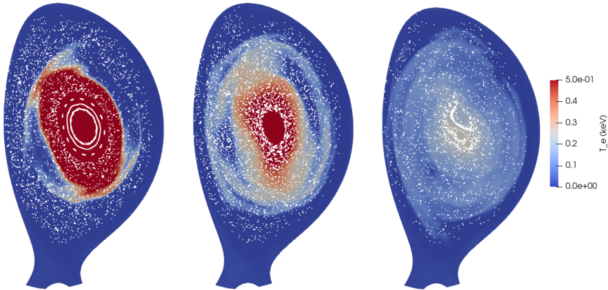
Figure 6. Poloidal cross-section of the electron temperature, with a Poincaré cross-section overlaid, in the injection plane at t = 4.62 (left), 4.91 (middle) and 5.09 ms (right) for Case B (see Table 1). The color scale is saturated at 0.5 keV so as to highlight the dynamics in the cold regions.
