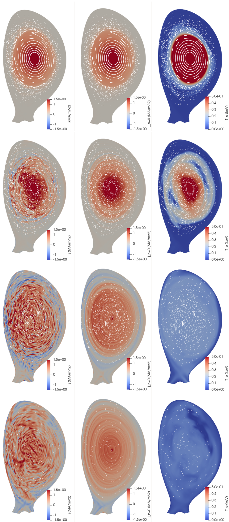
Figure 17. Poloidal cross-sections of the toroidal current density j_\phi (left), the axisymmetric part of the toroidal current density j_{\phi,n=0} (middle), and the electron temperature T_e (right) at times 5.26, 5.72, 6.05 and 6.54 ms (top to bottom) for Case D.
