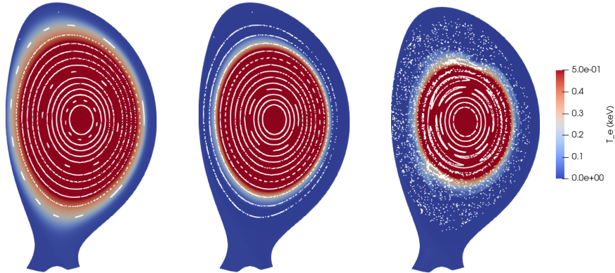
Figure 4. Poloidal cross-section of the electron temperature, with a Poincaré cross-section overlaid, in the injection plane at t = 0 (left), 2.78 (middle) and 4.33 ms (right) for Cases A, B and C, which are identical in this phase (see Table 1). The color scale is saturated at 0.5 keV so as to highlight the dynamics in the cold regions.
