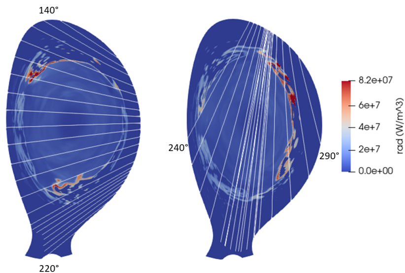
Figure 14. Poloidal cross-section of the radiated power per unit volume at 6.24 ms in the plane of the horizontal (KB5H, left) and vertical (KB5V, right) bolometers, with lines of sight shown in white and extreme angles indicated for easier comparison with Fig. 14.
