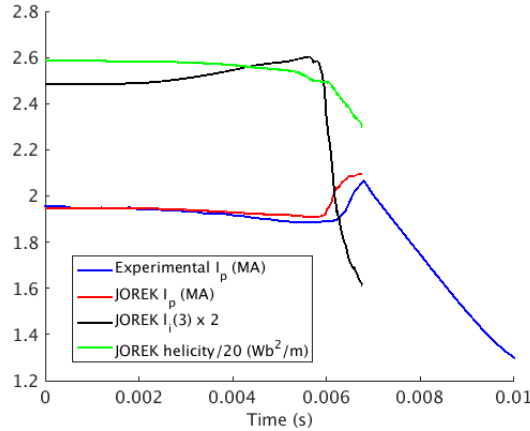
Figure 20. Evolution of the experimental and simulated plasma current as well as simulated plasma internal inductance and global magnetic helicity for Case D.
