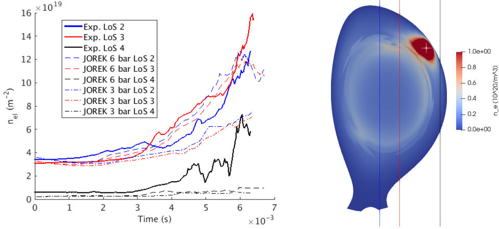
Figure 3. Left: Comparison between experimental (plain lines) and synthetic interferometry data from two JOREK simulations with DMV1 pressures of 6 (dashed) and 3 bar (dash-dotted). Right: Cross-section of the electron density from the 6 bar simulation showing the interferometry lines with the same color code as in the left figure.
