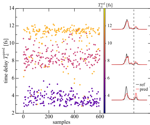
FIG. 9. Same as Fig. 8 but for 3D helium for which the network was not trained. The distribution of predicted time-delays shows three main peaks at 4, 8, 12 fs. The single-shot spectra are averaged over all spectra with time-delays in an interval of 1 fs about the three peaks. The averaged spectra are passed through the trained network to obtain the corresponding purified spectra shown on the right (red). The three averaged reference spectra (black) are obtained in the same way.
