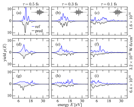
FIG. 5. Prediction of 3D helium spectra (black) for partially coherent pulses (1). The reference 3D helium spectra are shown in blue.
