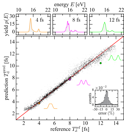
FIG. 7. Predicted time-delays against reference time-delays for the test data. The pulse energy is E_p = 1.6 \times 10^{16} W fs/cm 2 . The error distribution of the time-delays for the test data is shown in the lower inset. The red line represents error free prediction. The trained network is transferred to the 3D helium spectra for three time delays: 4 fs, 8 fs, and 12 fs with the reconstructed time delays shown as circles and double pulse shapes sketched. The upper inset gives the corresponding photoelectron spectra.
