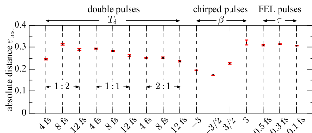
FIG. 2. Absolute distance error \epsilon_{\text{test}} (8d) of the different predicted spectra for test data: double pulses with time delay T_d and amplitude ratios A_1 : A_2 as indicated, chirped pulses with chirp parameter \beta , and partially coherent pulses with coherence time \tau .
