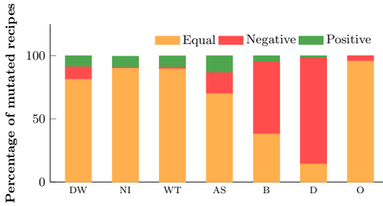
Fig. 8. Effect of different settings on the precision and performance of the abstract interpreter. (DW: NUM_DELAY_WIDEN, NI: NUM_NARROW_ITERATIONS, WT: NUM_WIDEN_THRESHOLDS, AS: array smashing, B: backward analysis, D: abstract domain, O: ingredient ordering).
