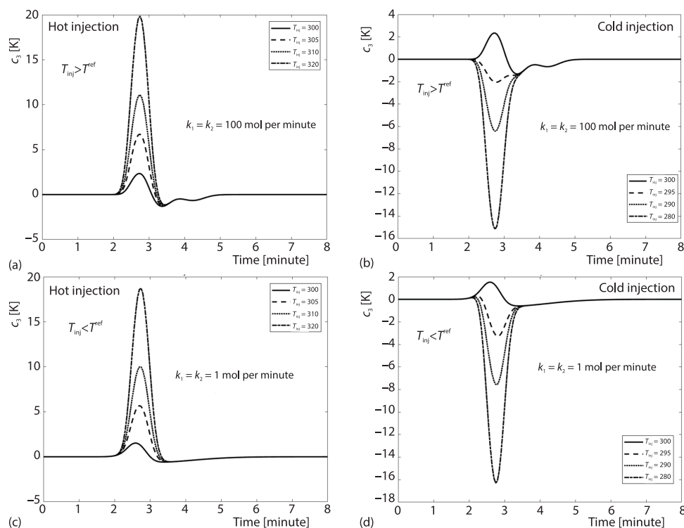
Figure 6. The effect of T_{inj} \neq T^{ref} on profiles for C_d/C_r = 1 ; here, two different values of mass transfer coefficients are considered; all other parameters are given in tab. 1
