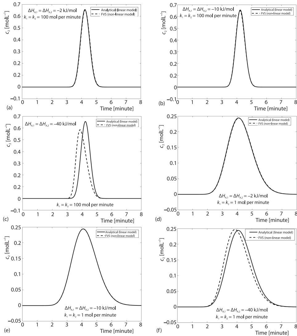
Figure 3. A comparison of concentration profiles of the second component obtained from analytical and numerical solutions for two different values of mass transfer coefficient k_i = 1 or 100 mol per minute ( i = 1, 2 ) when \Delta H_{A,i} \neq 0
