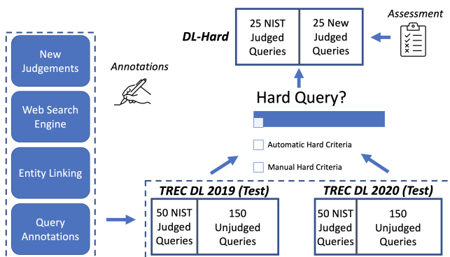
Figure 2: DL-HARD dataset overview.
