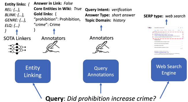
Figure 1: DL-HARD annotation process overview.
