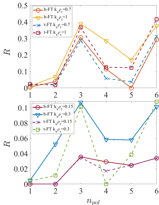
Figure 6. Dependency of the ZF residual level, R , with the FT length for the two FTs and several radial scales of the perturbation k_x , obtained from simulations with GENE in the W7-X KJM magnetic configuration.
