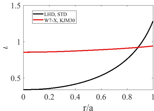
Figure 1. Radial profile of the rotational transform for the two magnetic equilibria used in this work: the vacuum standard configuration of LHD and a high mirror (KJM) configuration of W7-X with \beta = 3\% .
