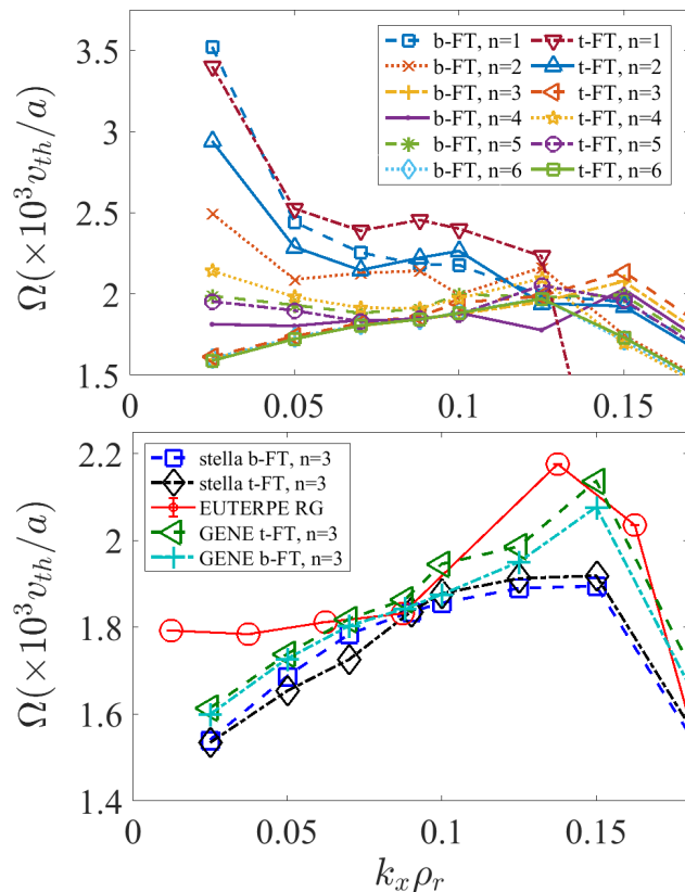
Figure 7. ZF oscillation frequency versus k_x in the W7-X configuration at r/a=0.5 from simulations with GENE in FTs with lengths n_{pol} = 1 - 6 (top). Comparison of ZF frequency in FT simulations with GENE and stella with n_{pol} = 3 and RG simulations with EUTERPE in W7-X (bottom).
