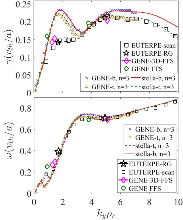
Figure 12. Comparison of growth rate \gamma (top) and frequency \omega (bottom) vs normalized wavenumber k_y \rho_r for FT, FFS and RG simulations in the KJM configuration of W7-X with \beta=3\% at r/a = 0.5 . Several FFS and RG simulations using different resolutions are included (see text and table 2).
