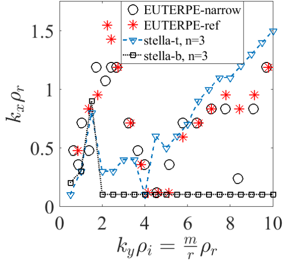
Figure 14. Radial scale k_x of the most unstable mode in RG simulations with EUTERPE scanning for different k_y and also for simulations with stella in the triangular and bean FTs at n = 3 . The radial scale is obtained in EUTERPE by Fourier transforming the potential profile at \phi = 0 .
