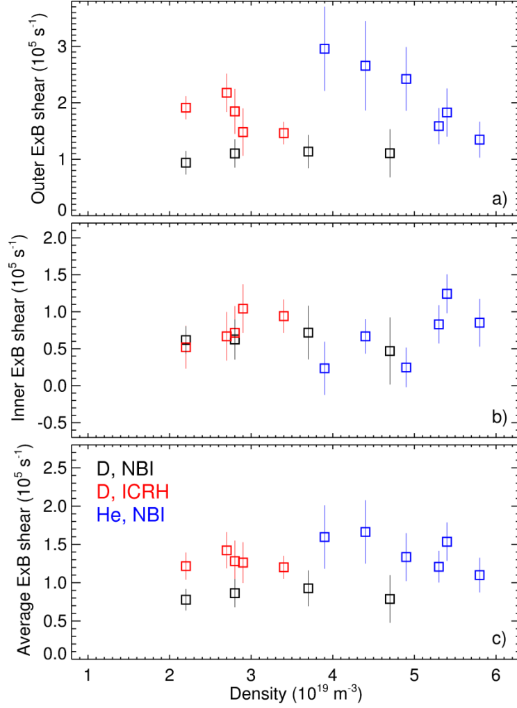
Figure 5: Outer, inner and average E×B flow shear at the L-H transition estimated from DBS v_{\perp} measurements at the separatrix, well and pedestal regions.
