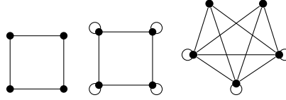
FIGURE 1. The graphs C_4 , C_4^o , and \Gamma_3
