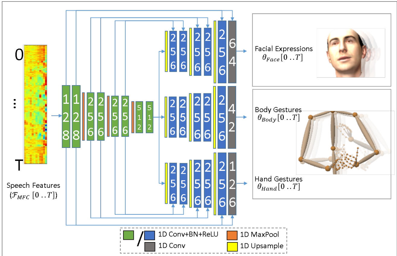
(a) Generator architecture.
