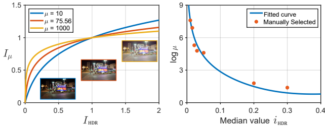
Figure 4: Left: Adaptive \mu -law compression (Eq. 2) for different \mu values and the corresponding compressed HDR images. In this case \mu = 75.56 has been selected for this image using Eq. 3. Right: Experimentally derived \mu selection as a function of HDR image median intensity i_{\text{HDR}} .
