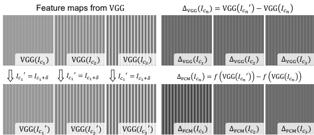
Figure 6: Left: VGG feature maps (1st layer, 2nd channel) for three input sinusoids of increasing image contrast ( c_1 < c_2 < c_3 ) (upper row) that is distorted by further increasing their amplitudes by the same factor \delta (bottom row). Right: the differences \Delta_{VGG} between the VGG feature maps, which are computed for each sinusoid and its distorted version, show a weak dependence to the input sinusoid contrast (upper row), while the corresponding differences \Delta_{FCM} resulting from our feature contrast masking model stronger penalize the distortion for smaller contrast sinusoids.
