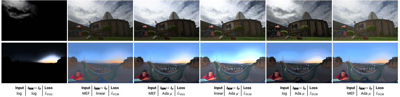
Figure 10: Example visualizations of our ablation study. Better contrast, brightness and detail reproduction is achieved with our full pipeline including multiple exposure fusion (MEF), adaptive \mu -law compression (Ada \mu ), and \mathcal{L}_{\text{FCM}} loss.
