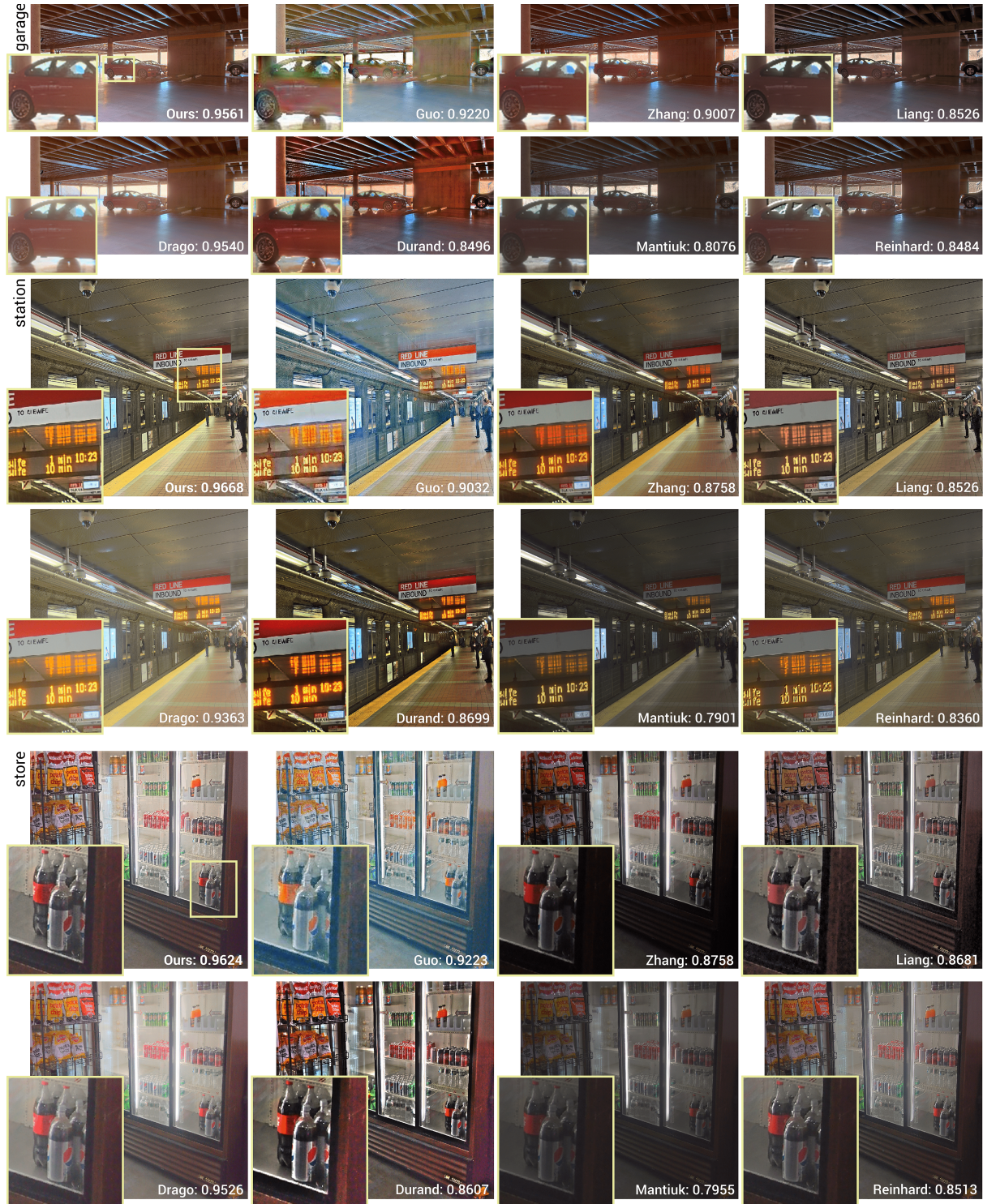
Figure 7: Visual comparisons for the best performing methods and their TMQI scores. Overall, our results achieve good contrast reproduction while preserving the details (highlights of the bottles in store , floor in station ) and avoiding visual artifacts (display sign in station , car edges and windows in garage ). Please refer to the text for an in-depth discussion of the observed differences.
