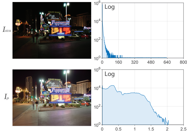
Figure 3: Image appearance and logarithmic histogram of pixel intensities for a transformed HDR image. Top Row: I_{\text{HDR}} with the mean normalized to 0.5. Bottom row: I_{\mu} derived using the adaptive \mu -law compression (Eqs. 2 and 3). Notice the dramatically different scales on the x -axis.
