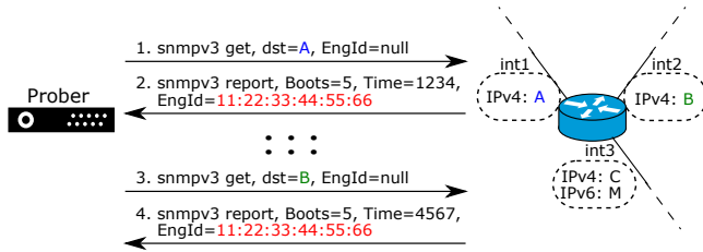
Figure 1: Unauthenticated, unsolicited SNMPv3 probes to router IPs return the SNMP engine uptime, reboot count, and engine ID. The engine ID is a unique, persistent identifier, typically formed from a MAC address on the device. Here, IPv4 interfaces A and B return the same engine ID, facilitating efficient alias resolution and vendor fingerprinting. Similarly, our technique can identify dual-stack aliases, e.g., IPv6 address M is an alias of A, B and C.
