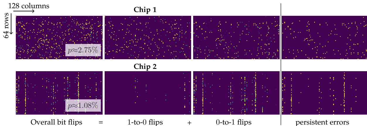
Fig. B: Low-Voltage Induced Bit Errors on Profiled Chips. We break the the bit error distribution of chips 1 and 2 down into 1-to-0 and 0-to-1 bit flips. Additionally, we show that most of the bit errors are actually persistent and, thus, not subject to randomness. As before, we show a sub-array of size 64 \times 128 from all profiled bit cells (i.e., across all SRAM arrays). Sec. B includes details on profiling.
