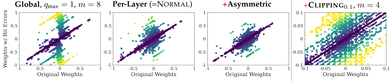
Fig. 4: Quantization and Random Bit Errors. Original weights (x-axis) plotted against perturbed weights with bit errors (y-axis), for different fixed-point quantization schemes with m = 8 bit (left) and p = 2.5\% . We also show the m = 4 bit case with CLIPPING at w_{\max} = 0.1 , cf. Sec. 4.2. Color indicates absolute error: from zero (violet) to the maximal possible error (yellow) of 1 (left) and 0.1 (right). Asymmetric per-layer quantization reduces the impact of bit errors compared to the symmetric per-layer/global quantization. Clipping reduces absolute error, but the errors relative to w_{\max} increase.
