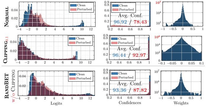
Fig. 6: Effect of Weight Clipping. On CIFAR10, weight clipping constrains the weights (right), thereby implicitly limiting the possible range for logits (left, blue). However, even for w_{\max}=0.1 the DNN is able to produce high confidences (middle, blue), suggesting that more weights are used to obtain these logits. Furthermore, the impact of random bit errors, p = 1\% , on the logits/confidences (red) is reduced significantly. RANDBET (trained with p = 1\% , w/o weight clipping), increases the range of weights and is less effective at preserving logit/confidence distribution.
