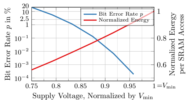
Fig. A: Energy and Low-Voltage Operation. Average bit error rate p (blue, left y-axis) from 32 14nm SRAM arrays of size 512 \times 64 from [5] and energy (red, right y-axis) vs. voltage (x-axis). Voltage is normalized by V_{min} , the minimal measured voltage for error-free operation, as well as the energy per SRAM access at V_{min} . SRAM accesses have significant impact on the DNN accelerator’s energy [18]. Reducing voltage leads to exponentially increasing bit error rates.
