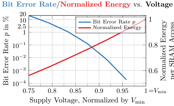
Fig. 1: Energy and Low-Voltage Operation. Average bit error rate p (blue, left y-axis) from 32 14nm SRAM arrays of size 512 \times 64 from [5] and energy (red, right y-axis) vs. voltage (x-axis). Voltage is normalized by V_{\min} , the minimal measured voltage for error-free operation, and the energy per SRAM access at V_{\min} . SRAM accesses have significant impact on the DNN accelerator’s energy [18]. Reducing voltage leads to exponentially increasing bit error rates.
