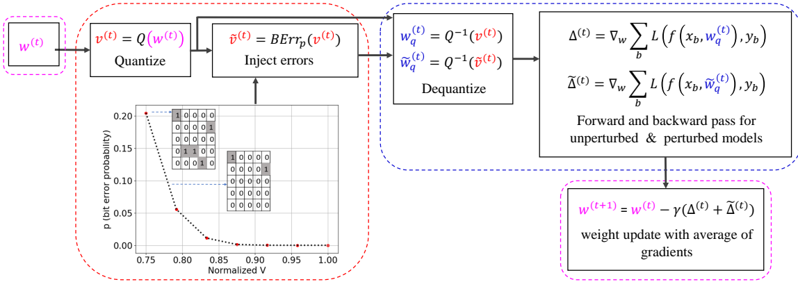
Fig. 5: Random Bit Error Training (RANDBET) . We illustrate the data-flow for RANDBET as in Alg. 2. Here, BErr_p injects random bit errors in the quantized weights v^{(t)} = Q(w^{(t)}) , resulting in \tilde{v}^{(t)} , while the forward pass is performed on the de-quantized perturbed weights \tilde{w}_q^{(t)} = Q^{-1}(\tilde{v}^{(t)}) , i.e., fixed-point arithmetic is not emulated. The weight update during training is not affected by bit errors and computed in floating point .
