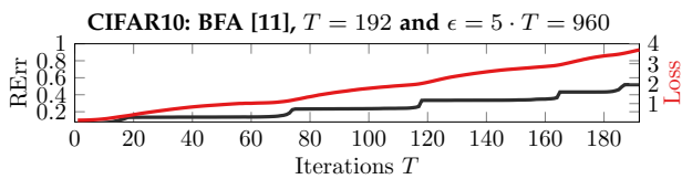
Fig. 8: BFA Iterations . RErr and loss (after bit errors, in red) plotted against BFA iterations. We allow 5 bit flips per iteration, totaling 960 bit errors for 192 iterations. RErr tends to increase (roughly) in steps of \sim 10\% by flipping predictions consecutively to a constant one for each class.
