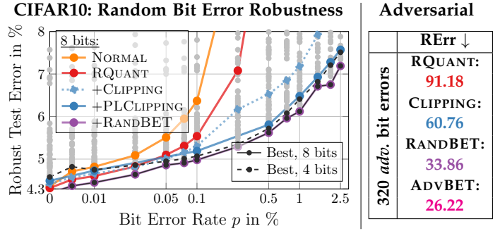
Fig. 2: Robustness to Random Bit Errors. Left: Robust test error RErr after injecting random bit errors (lower is better ↓, y-axis) plotted against bit error rate p (x-axis). For 8 bit, robust quantization (RQUANT, red), additionally weight clipping (CLIPPING, dotted blue) or per-layer weight clipping (PLCLIPPING, solid blue) and finally adding random bit error training (RANDBET, violet) robustness improves significantly. Robustness to higher bit error rates allows more energy efficient operation, cf. Fig. A. The Pareto optimal frontier is shown for 8 bit (black solid) and 4 bit (dashed) quantization. Right: RErr against up to 320 adversarial bit errors, showing that CLIPPING combined with RANDBET or ADVBET also allow secure operation.
