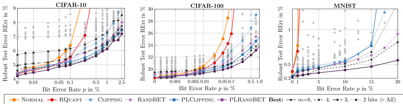
Fig. 7: Bit Error Robustness on CIFAR10, CIFAR100 and MNIST. Average RErr plotted against bit error rate p , both in %. We considered various models (in \bullet gray), corresponding to different w_{\max} and p during training. We explicitly plot the best model for each bit error rate: for NORMAL (orange), RQUANT (red), CLIPPING (blue) and RANDBET (violet). Note that these might correspond to different w_{\max} and p (also across datasets). Across all approaches, we plot the per-error-rate best model in black: for m = 8, 4, 3, 2 bits, depending on dataset. For 8 bit and low bit error rates, CLIPPING is often sufficient. However, for 4 bit or higher bit error rates, RANDBET is crucial to keep RErr low.
