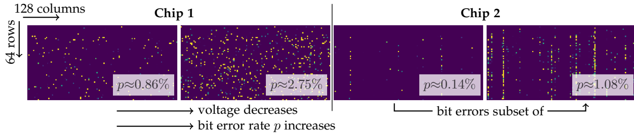
Fig. 3: Exemplary SRAM Bit Error Patterns. Measured bit errors from two chips with on-chip SRAM (left and right), showing bit flip probability for a segment of size 64 \times 128 bits: yellow indicates a bit flip probability of one, violet indicates zero probability. We show measurements corresponding to two supply voltages. With lower voltage, bit error rate increases. Also, the bit errors for higher voltage (= lower bit error rate) are a subset of those for lower voltage (= higher rate), cf. Sec. 3. Our error model randomly distributes bit errors across space. However, as example, we also show SRAM chip 2 which has a different spatial distribution with bit errors distributed along columns. We aim to obtain robustness across different memory arrays, voltages and allowing arbitrary DNN weight to memory mappings.
