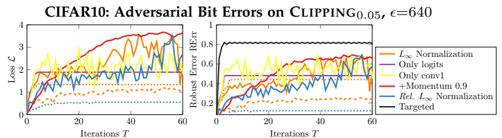
Fig. 9: Adversarial Bit Error Iterations . We plot loss, cf. Eq. (1), and robust error RErr against iterations, both measured on the 100 held-out test examples used to find, i.e., train, adversarial bit errors. Clearly, L_\infty gradient normalization with momentum (in red), targeting first convolutional (yellow) or logit layer (violet) is most effective for untargeted attacks. Unfortunately, the attack gets easily stuck in bad optima if learning rate is not optimal. Targeted attacks simplify optimization and are often more effective (black, right).
