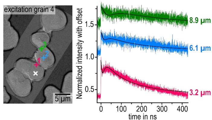
Figure 4.8: Optical reflection image and PL transients upon excitation on grain four of \text{MAPbI}_3 cluster. Optical reflection image overlaid with the AFM deflection signal from Figure 4.6. The white cross marks the excitation position, detection positions of PL transients on the right indicated by the magenta, blue and green crosses. Fit according to Equation 4.3 shown in black.
