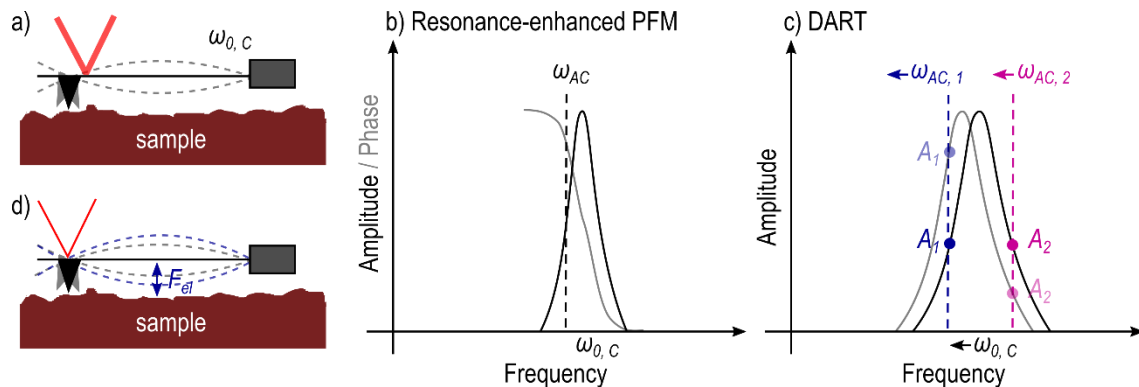
Figure 1.18: a) Schematic of contact resonance \omega_{0,c} as grey dashed lines, forming a standing wave motion. b) Contact resonance in frequency spectrum with PFM AC excitation close to the contact resonance \omega_{0,c} at \omega_{AC} . Detection at the same frequency leads to enhanced signal-to-noise ratio. c) DART working principle using two excitation and detection frequencies \omega_{AC,1} and \omega_{AC,2} left and right of the contact resonance. An additional feedback compares the amplitude ratio at both frequencies A_1/A_2 and adjusts the drive frequencies to maintain a constant ratio, thereby compensating for shifts in the contact resonance \omega_{0,c} . 209 d) Accurate positioning of the interferometric displacement sensor above the tip reduces the influence of electrostatic crosstalk F_{el} on the PFM data. 210
