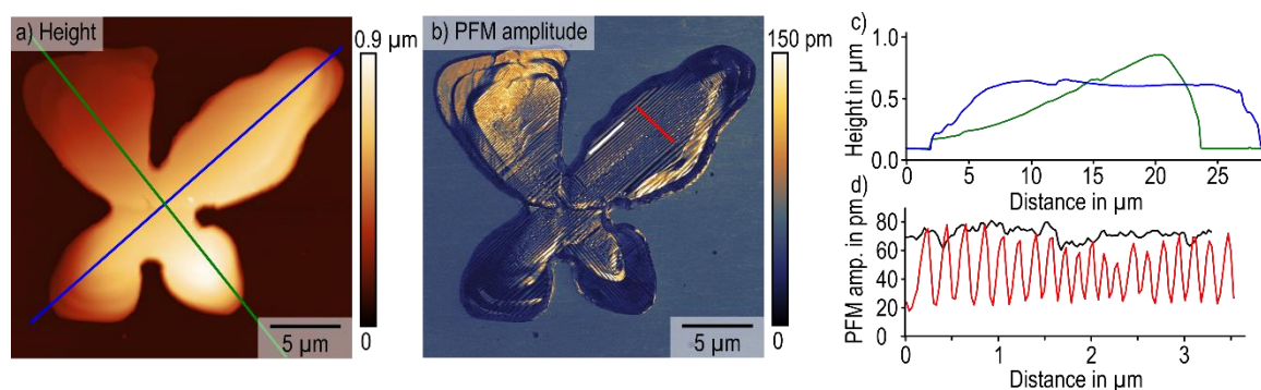
Figure 3.9: Lateral PFM measurement on a large, isolated MAPbI 3 grain on fused silica. a) The height channel shows a four-armed crystallite with a maximum thickness of 0.8 \mu\text{m} . b) The PFM amplitude displays the characteristic striped domain pattern assigned to ferroelasticity. c) Height profiles extracted along green and blue line in a). d) PFM amplitude profiles extracted along the red and white line in b), showing an average domain spacing of 130 \text{ nm} in the red profile. Lateral PFM performed with 2\text{V} AC excitation close to lateral contact resonance at 718 \text{ kHz} .
