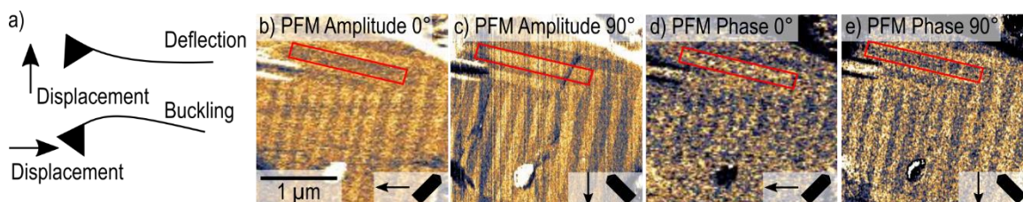
Figure 3.5 a) Illustration of difference between vertical deflection and cantilever buckling. (b–e) Vertical PFM measurement on MAPbI 3 film ( V_{ac} = 2.5 V, f_{Drive} = 300 kHz, and scan angle = 45°; cantilever orientation and fast scan direction are indicated in the insets in the lower right corners. b) PFM amplitude at 0° sample rotation and c) at 90° sample rotation, d) PFM phase at 0° sample rotation, and e) at 90° sample rotation. The red box marks the same domain in (b–e). Reprinted with permission from J. Phys. Chem. C 2016, 120, 10, 5724–5731. Copyright 2016 American Chemical Society.
