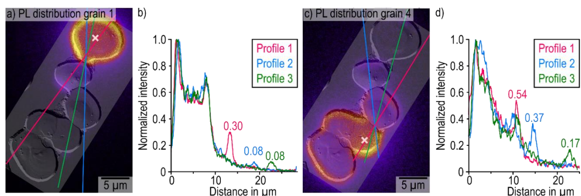
Figure 4.10: a) Static PL distribution of \text{MAPbI}_3 grain cluster upon local optical excitation in grain one overlaid with a semitransparent image of the AFM deflection from Figure 4.6. The excitation position is marked by the white cross, extraction positions of the three line profiles in b) shown by the magenta (Profile 1), blue (Profile 2) and green line (Profile 3). c) Static PL distribution of \text{MAPbI}_3 grain cluster upon local optical excitation in grain four overlaid with a semitransparent image of the AFM deflection from Figure 4.6. The excitation position is marked by the white cross, extraction positions of the three line profiles in d) shown by the magenta (Profile 1), blue (Profile 2) and green line (Profile 3). All line profiles were smoothed with a 7-point moving average. Excitation with 633 nm wavelength, a fluence of 0.77 \mu\text{J cm}^{-2} , a repetition rate of 20 MHz and 0.82 \mu\text{m} beam diameter (SI in Appendix 8.2, Figure 8.8).
