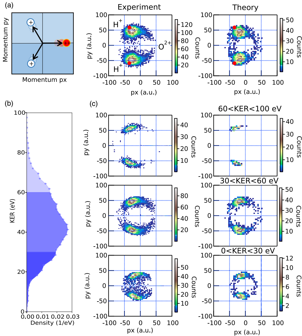
FIG. 2. Newton diagrams. (a) Newton diagrams (experiment and theory) of the ion momenta for O^{2+} and two H^+ ions detected in coincidence, where the oxygen momentum defines the x axis, for the full KER range. On the left, the employed momentum coordinate system is shown. The red dots mark the momentum values expected for an instantaneous Coulomb explosion. (b) Distribution of the KER for the three fragments. (c) Newton diagrams (experiment and theory) for selected KER ranges, indicated in (b) by the different color shadings.
