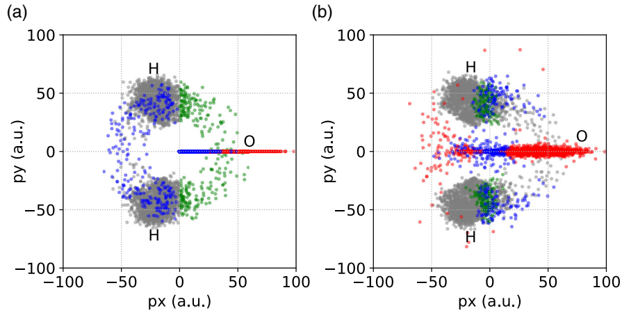
FIG. 10. Final ion momenta for \text{H}_2\text{O}^{4+} in two different orientations. (a) The momenta are oriented such that the final oxygen momentum is oriented along the x axis. (b) The momenta are oriented according to the initial geometry (oxygen is initially on the positive x axis). Gray dots mark proton momenta; red dots mark oxygen momenta. Green dots mark proton momenta with a positive component along the corresponding oxygen momentum. Blue dots mark the corresponding partner proton and oxygen momenta.
