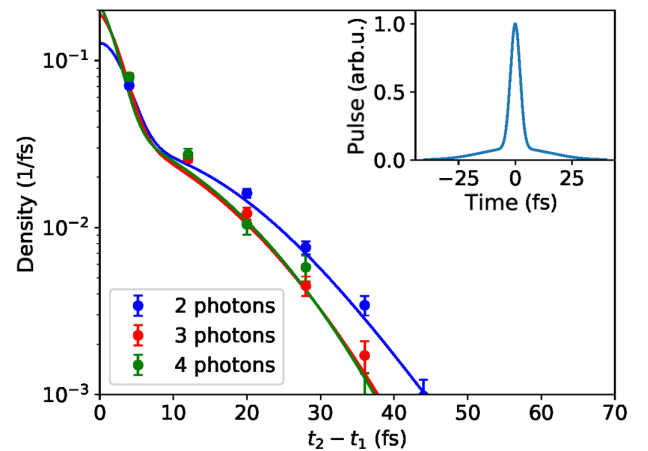
FIG. 17. Differential probability distribution of the time between the first and second photoionizations, t_2 - t_1 . The inset shows the employed double-Gaussian temporal pulse shape. Solid lines show results from an analytical model assuming constant ionization cross sections, and dots depict results from the actual simulation. Error bars depict standard errors.
