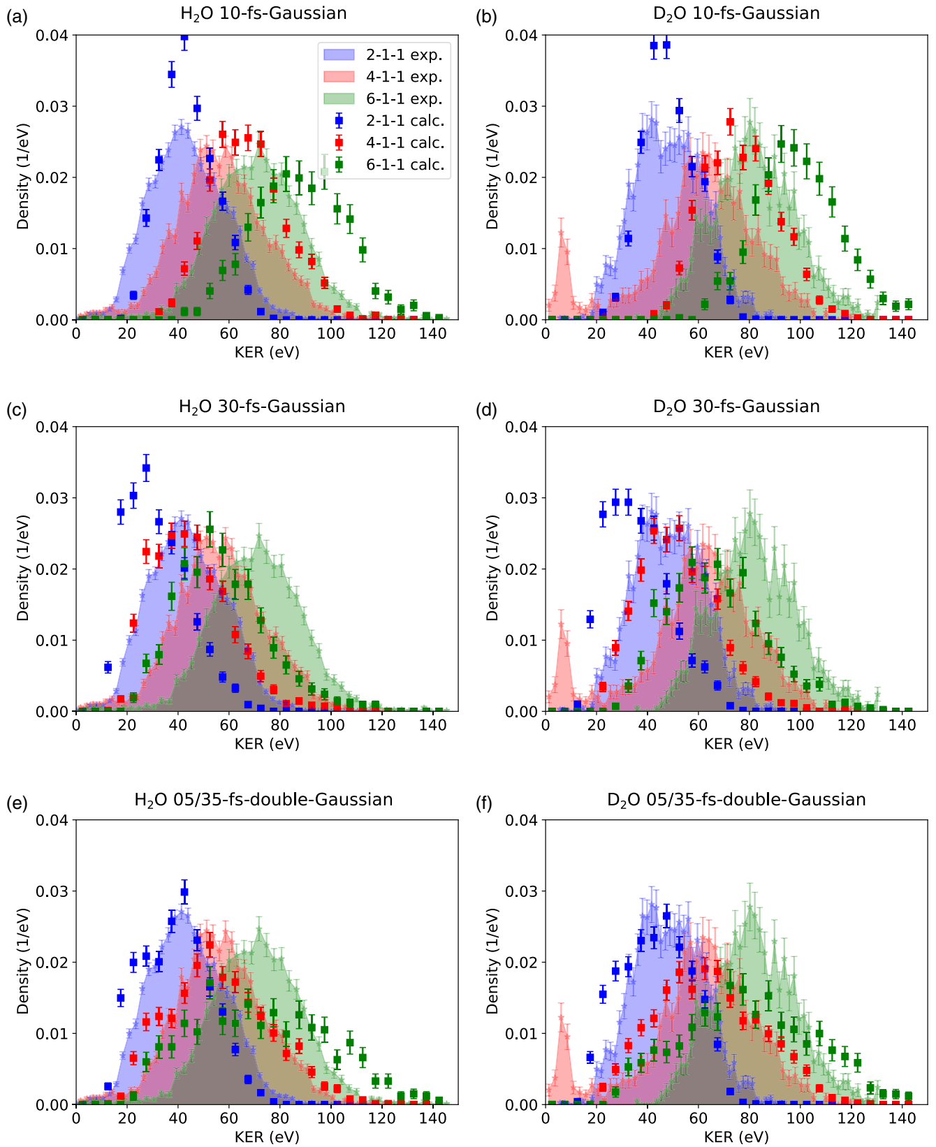
FIG. 9. Total kinetic energy release for \text{H}_2\text{O} and \text{D}_2\text{O} for different coincidence channels and for different temporal pulse shapes. Here, x-1-1 labels coincidence channels with final oxygen fragment charge +x and hydrogen charges +1 . The squares show data from the simulation; the asterisks and the shaded areas show data from the experiment. The error bars show standard errors due to finite sampling. Note that the peak at 10 eV for \text{D}_2\text{O} in the experimental data is an artifact caused by \text{He}^+ .
