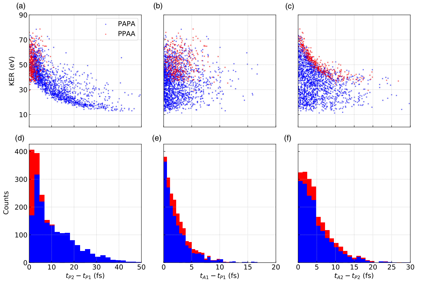
FIG. 11. Scatter plots [(a)–(c)] showing the relation of different ionization times with KER, and histograms [(d)–(f)] showing the distribution of ionization times for \text{H}_2\text{O} and the coincidence with \text{O}^{2+} and 2\text{H}^+ . In the plots, t_{P1} and t_{P2} are the times of the two photoionization events, and t_{A1} and t_{A2} are the times of the two Auger decay steps. PAPA ionization sequences are marked in blue, and PPAA ionization sequences are marked in red.
