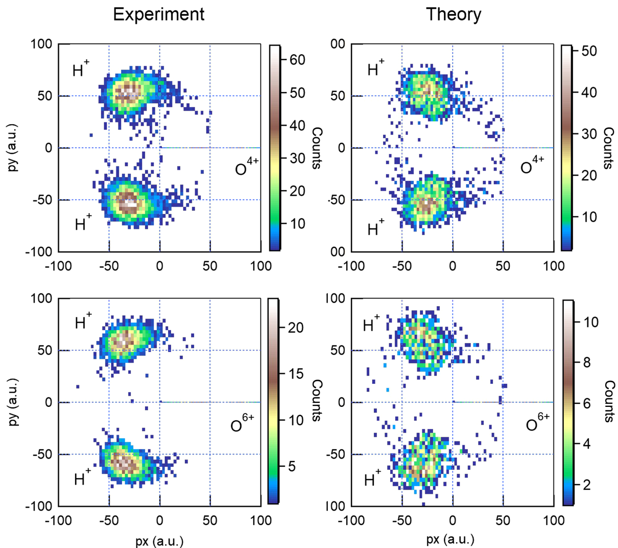
FIG. 5. Newton diagrams for the coincidences \text{O}^{4+} + 2\text{H}^+ and \text{O}^{6+} + 2\text{H}^+ . The left panels show experimental data; the right panels show data from the simulation.
