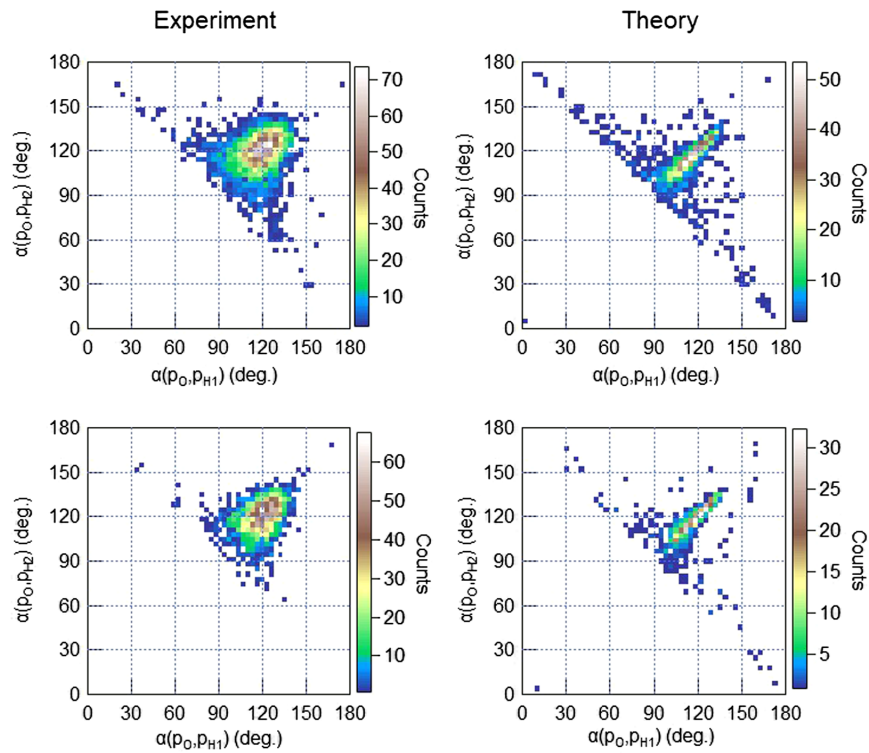
FIG. 13. Hydrogen-oxygen momentum angle pairs for different coincidence channels (top: 4-1-1; bottom: 6-1-1). The left column shows experimental results; the right column shows results from the simulation, respectively.
