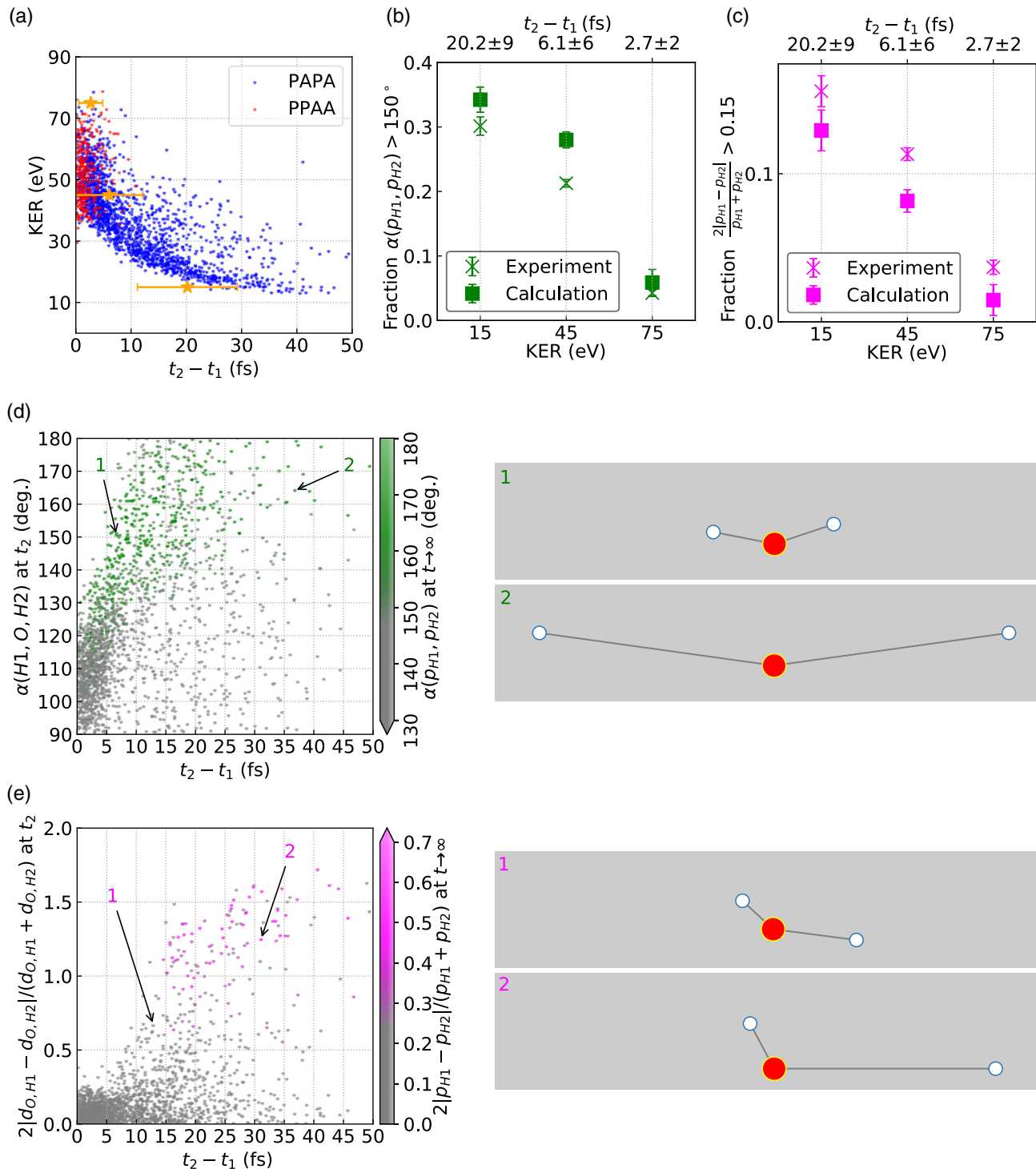
FIG. 4. Evolution in time. (a) KER as a function of time between the first and the second photoionization, t_2 - t_1 (simulation). Two different ionization sequences, alternating photoionization and Auger decay (PAPA) and two photoionizations followed by two Auger decays (PPAA), are marked in different colors. The yellow stars mark average delay times for the three KER bins considered in Figs. 1, 4(b), and 4(c). The bars indicate standard deviations of the delay times within the respective KER bins. (b,c) Fraction of coincidence events with large proton-proton momentum angle and large relative proton momentum asymmetry as a function of KER (experiment and simulation). (d,e) HOH bond angles and asymmetry ratio of the OH distances at the point in time of the second photoabsorption vs time delay with respect to the first photoabsorption (simulations) accompanied by selected snapshots of the molecular geometry. All plots are for coincidences with oxygen charge +2 and 2H^+ ions.
