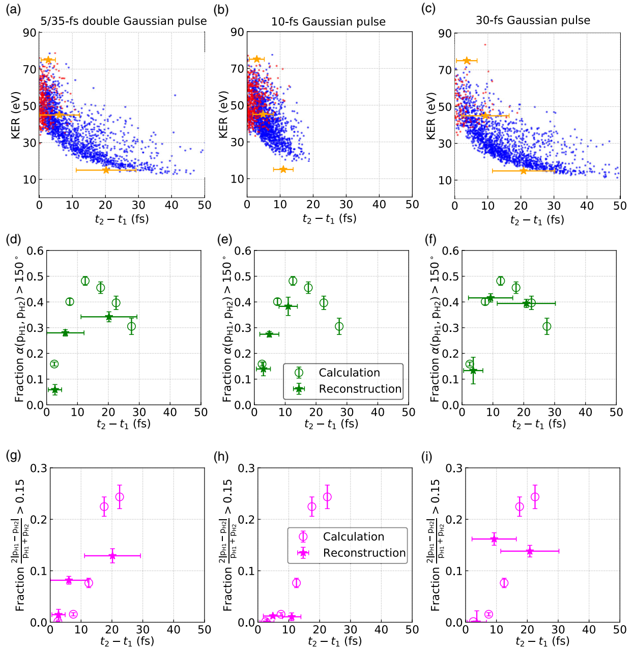
FIG. 16. (a)–(c) KER as a function of time between the first and the second photoionization t_2 - t_1 for different pulse shapes. The yellow stars mark the average timing values for the selected KER bins. The error bar shows the standard deviation of t_2 - t_1 within the bin. (d)–(f) Fraction of proton angles larger than 150^\circ as a function of t_2 - t_1 . (g)–(i) Fraction of proton asymmetry larger than 0.15 as a function of t_2 - t_1 . The circles show the data as extracted from the simulations, and the stars show data, where the timing information has been deduced by the KER–time relation. Vertical error bars indicate standard error, and horizontal error bars indicate the standard deviation of t_2 - t_1 within the selected KER bin.
