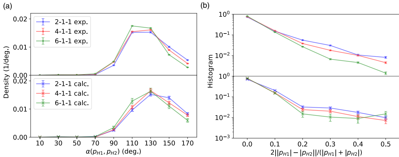
FIG. 6. Distribution of proton momentum angle (a) and proton momentum asymmetry (b) for different charge coincidences (experiment and simulations). The error bars show standard errors due to finite sampling.
