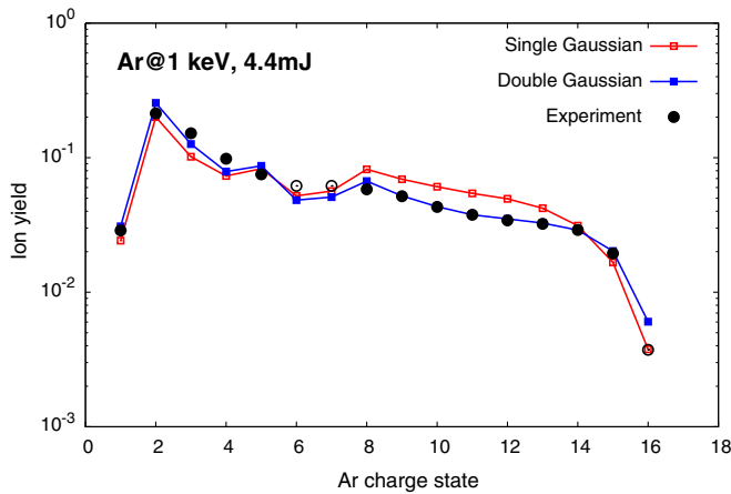
FIG. 14. Argon calibration measurement. The black circles show measured ion yields (open circles are excluded for calibration), and the lines show ion yields as calculated from atomic simulations. The red line shows results obtained with a single Gaussian for the spatial fluence distribution, while the blue line shows results obtained with a double-Gaussian fluence distribution. See text for the optimized parameters of the fluence distribution.
