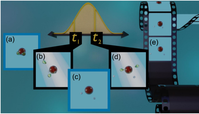
FIG. 1. Two-photon absorption dynamics. (a) Initial \text{H}_2\text{O} geometry. (b) As a consequence of the absorption of a photon (visualized using a bright flash) at time t_1 , and subsequent Auger decay, the water molecule loses two electrons (symbolized by the two green blobs ejected). (c) The doubly charged water molecule undergoes structural deformations. The yellow curve on top represents the temporal shape of the photon beam. (d) Through the absorption of a second photon at time t_2 , the molecule becomes quadruply charged and undergoes a Coulomb explosion. The molecular geometry at time t_2 leads to characteristic momentum vectors for the three fragments, i.e., the two protons and the \text{O}^{2+} ion that are detected for each molecule individually. (e) Using the ion momentum vectors detected in coincidence in combination with theory, information is retrieved on the structural properties of the doubly charged water molecule at a delay of t_2 - t_1 .
