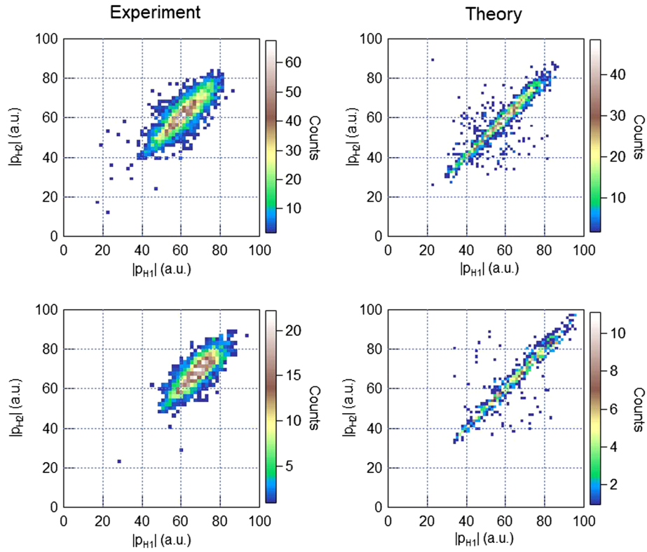
FIG. 12. Hydrogen absolute momenta pairs for different coincidence channels (top: 4-1-1; bottom: 6-1-1). The left column shows experimental results; the right column shows results from the simulation, respectively.
