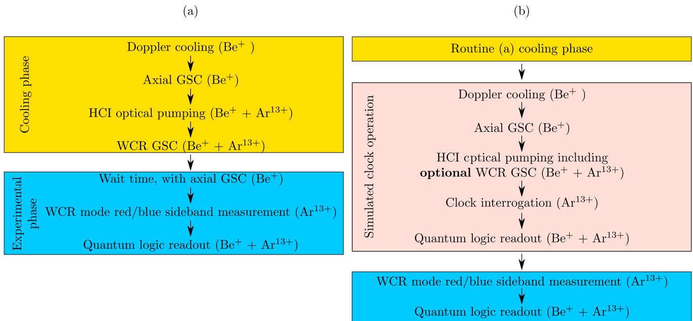
Figure 2. Simplified depiction of the two main experimental sequences used in this work, with the cooling phases (yellow), clock operation (pink) and experimental (blue) phases indicated. GSC = ground-state cooling. The ions involved in each step are also indicated. Sequence (a) was used to measure anomalous heating rates for the WCR modes, Rabi flopping, and for sideband scans. Sequence (b) was used to demonstrate suppression of the heating of the WCR modes during simulated clock operation, as displayed in Fig. 5 in the main manuscript, with the central clock operation section repeated a variable number of times in order to measure the evolution of the WCR mode temperature over an increasing number of cycles.
