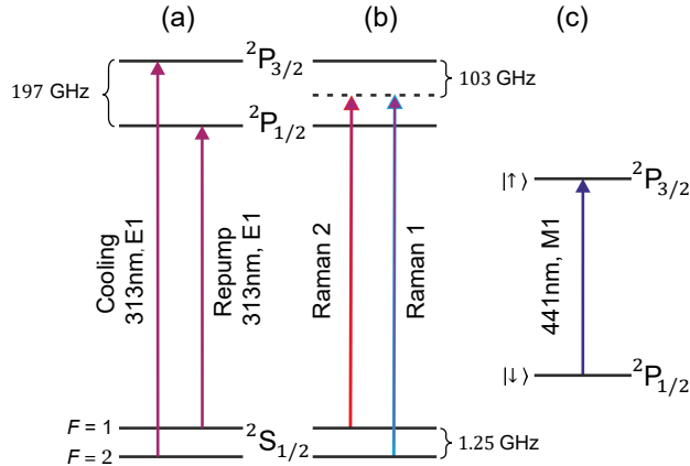
Figure 1. Partial term schemes of {}^9\text{Be}^+ and {}^{40}\text{Ar}^{13+} (energies not to scale), showing the transitions used for manipulation of the two-ion crystal. (a) Doppler cooling and repumping using the \text{Be}^+ ion, (b) driving stimulated Raman transitions on the \text{Be}^+ ion, and (c) driving sideband transitions using the \text{Ar}^{13+} ion. Hyperfine sublevels of the {}^2P_{1/2} and {}^2P_{3/2} states of {}^9\text{Be}^+ are omitted for clarity.
