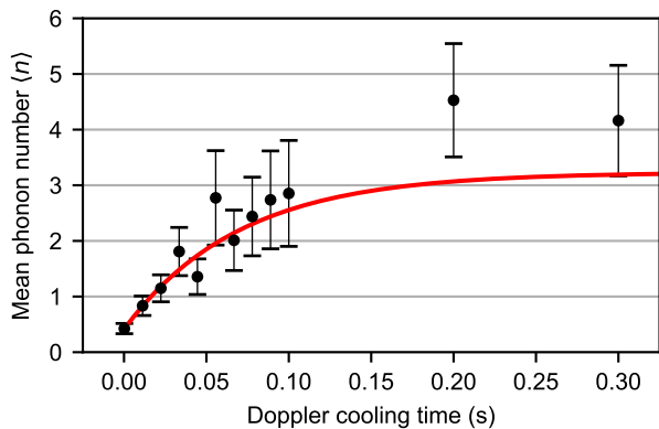
Figure 4. Heating of the y WCR mode out of the ground state during the Doppler cooling pulse applied to the \text{Be}^+ ion (black points), with the expected background from anomalous heating removed. The data is fitted (red line) using a semiclassical model.
