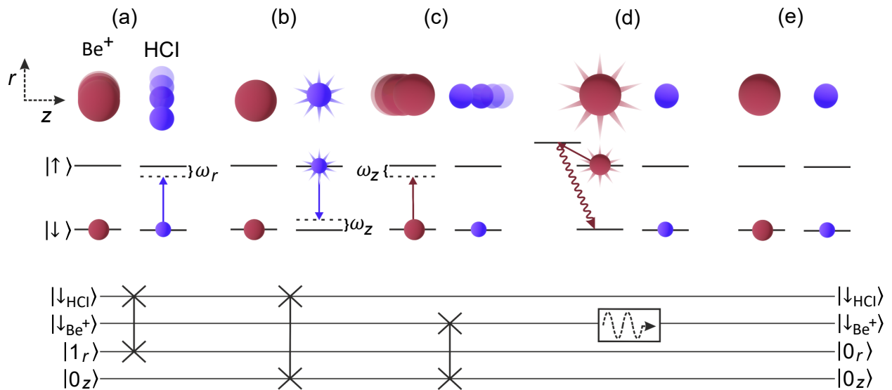
Figure 2. Upper: Scheme of the quantum logic sideband cooling sequence representing the state of the ion crystal before each of the depicted laser pulses is applied. Pulses (a) and (b) on the HCl (purple symbols) swap a phonon from one of the WCR modes ( r ) into the axial out-of-phase mode ( z ) through the excited electronic state of the HCl. Pulse (c) on the \text{Be}^+ ion (red symbols) removes the added phonon from the axial out-of-phase mode and converts it into an electronic excitation of the \text{Be}^+ ion. Pulse (d) dissipatively resets the \text{Be}^+ to its initial electronic state through spontaneous decay, completing the sequence and ensuring unidirectionality and cooling. Solid arrows depict driven transitions, undulating arrows represent spontaneous decay. |\downarrow\rangle and |\uparrow\rangle represent the ground and excited electronic states of the relevant ion, respectively. Lower: Representation of the sequence as a quantum circuit composed of a series of SWAP quantum gates. |1_i\rangle and |0_i\rangle represent the presence and lack of a phonon in mode i , respectively.
