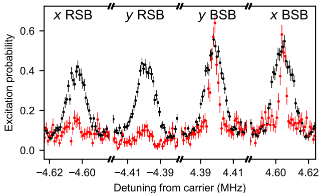
Figure 3. WCR motional sidebands of the two-ion crystal observed on the HCI before (black) and after (red) resolved sideband cooling. The error bars are statistical only, governed by quantum projection noise. The observed difference in the full-width-at-half-maximum values between the two cases is caused by the different lengths of the interrogation pulse used, which were adjusted in each case to produce the highest possible contrast. The scans have been re-centered for presentation, correcting for small drifts in the secular frequencies.
