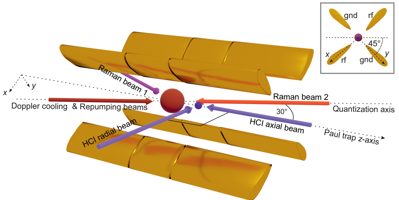
Figure 1. Simplified depiction (not to scale) of the two-ion Coulomb crystal of a single \text{Be}^+ ion (red, left) and a single HCl (purple, right) confined in a linear Paul trap. The laser beams needed for their manipulation are shown. The ions are located on the trap axis ( z ); radial motion evolves on the (x, y) coordinates defined by the trap electrodes which are at 45^\circ to the plane on which all the laser beams lie. The Doppler cooling, repumper, and Raman laser beams all intersect the z -axis at an angle of 30^\circ . The beam for addressing axial motion of the HCl is delivered along the z -axis, and the beam for addressing its radial motion is delivered perpendicular to it. Inset: radial cross section of the ion trap, showing the orientation of the radial trap axes as defined by the radiofrequency (rf) and ground (gnd) electrodes.
