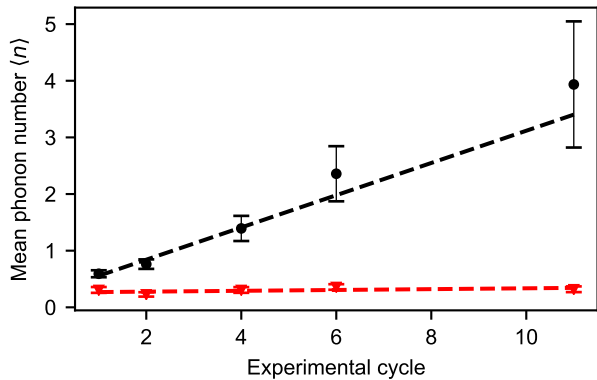
Figure 5. Suppression of the heating of the x WCR mode. Without additional algorithmic cooling, the ion heats up due to the anomalous electric field noise (black circles). A linear fit (black dashed line) implies a heating rate of 8.9(16) phonons/second, consistent with the previously measured value for this mode (see Table I). With one algorithmic cooling cycle applied on each WCR mode per experimental cycle, this heating is suppressed (red triangles), with a fitted heating rate of 0.18(15) phonons/second (red dashed line).
